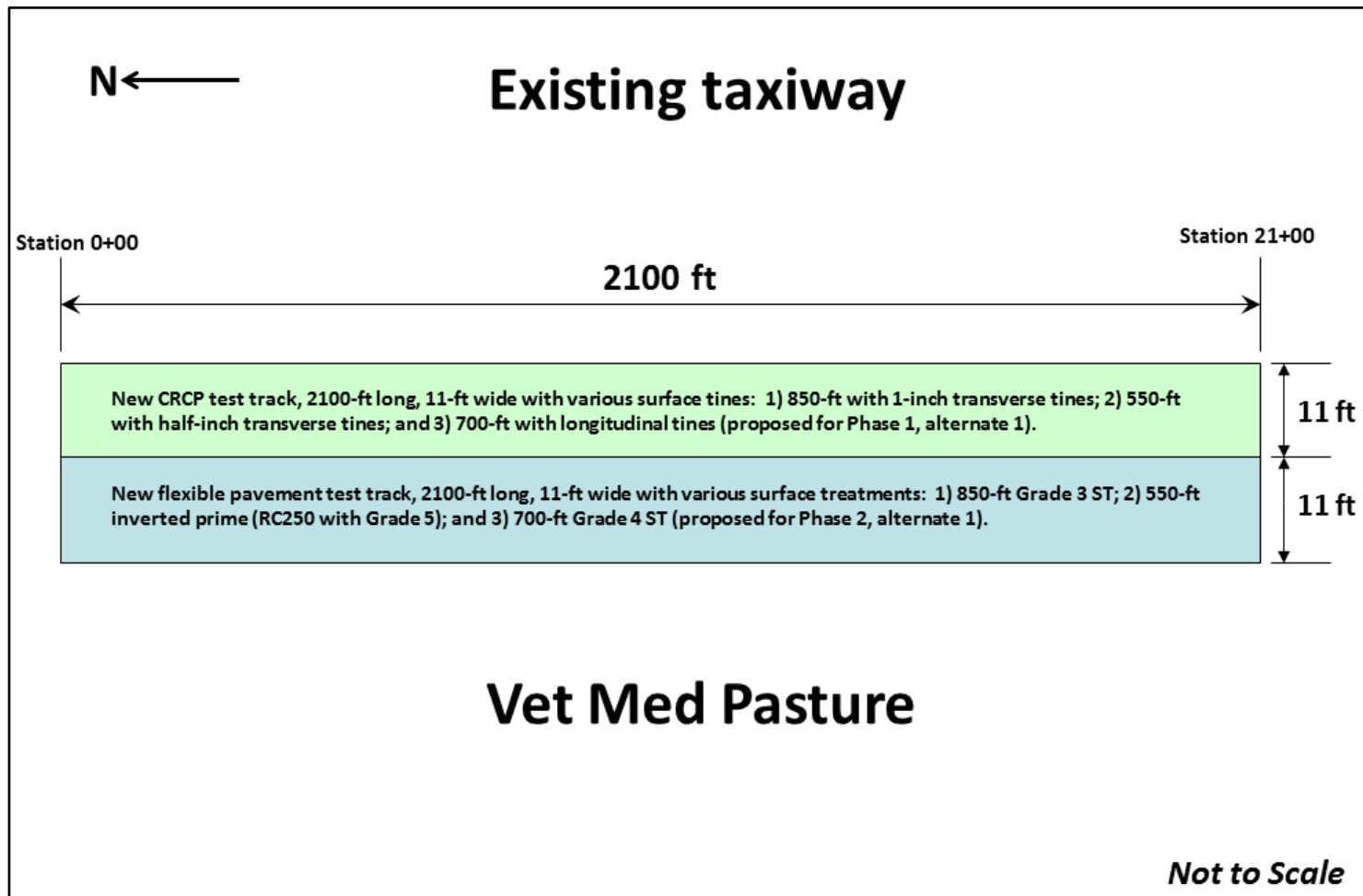
Figure 5. Plan View of Proposed New Test Tracks.
