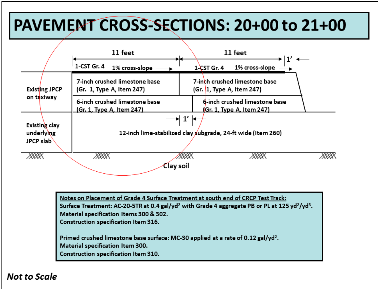
Figure 15. Typical Cross-Section of Optional 100-ft Grade 4 Surface Treatment at South End of CRCP Test Track.
