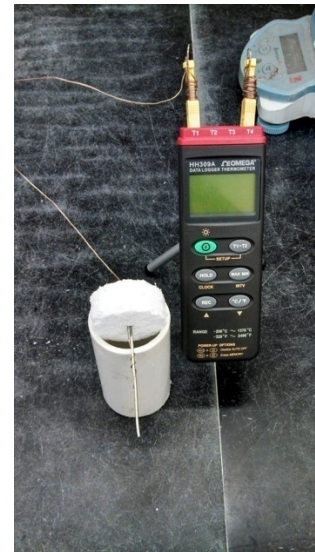
(b) probe placement in specimen
