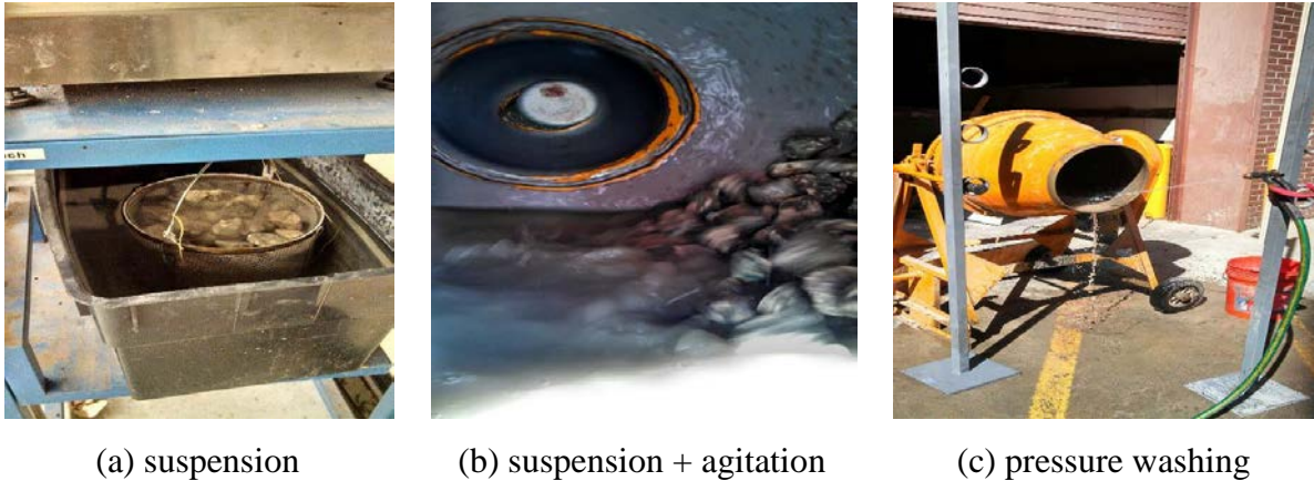
Figure 3.10: Testing Setup for Automated Aggregate Washing
