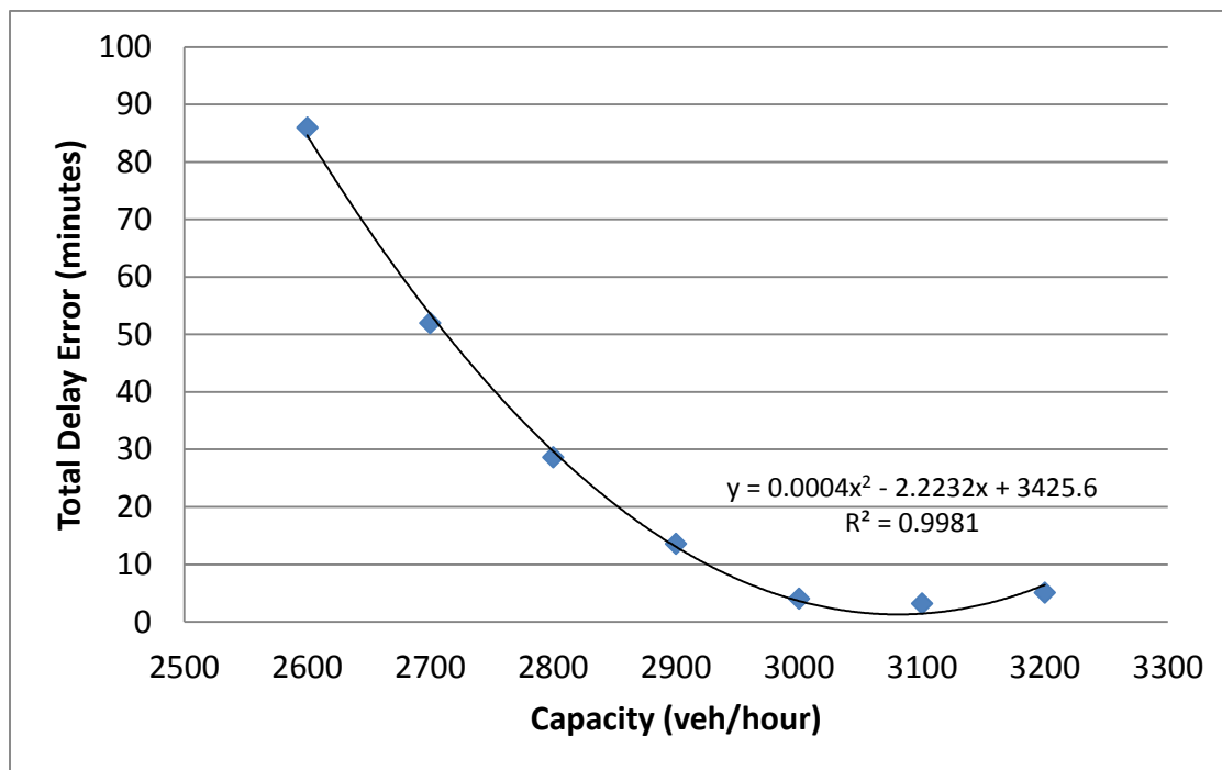
Figure 4.2 Delay error vs. capacity and least squares regression fit for July 19 th work zone data
