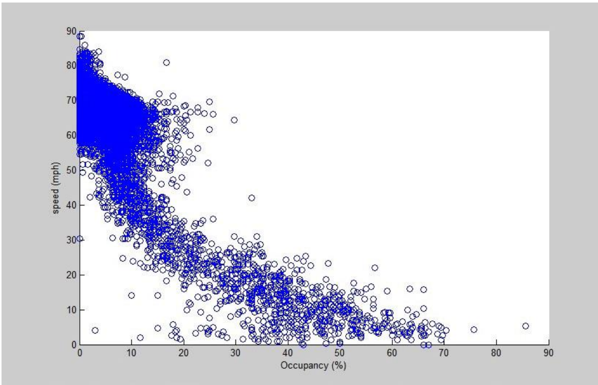
Figure 2.3 Q01: Speed-Occupancy Plot
