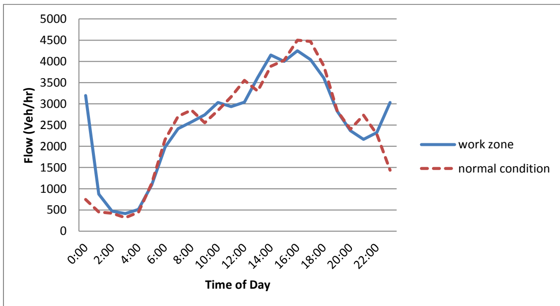
Figure 2.8 Hourly volumes with and without work zone at the westbound I-70 site
