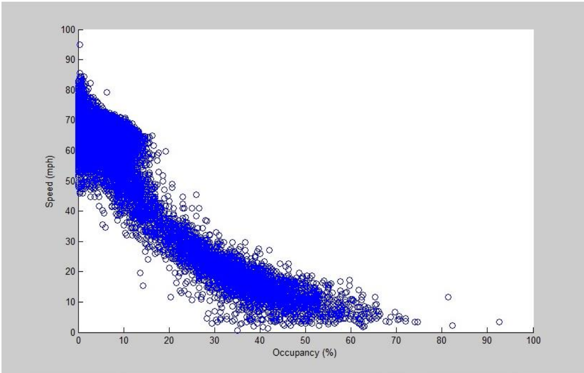
Figure 2.4 Q02: Speed-Occupancy Plot
