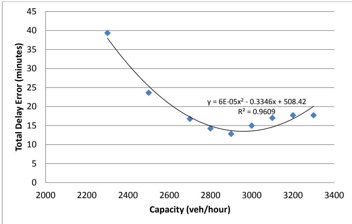
Figure 4.4 Least squares estimation for I-70 work zone
