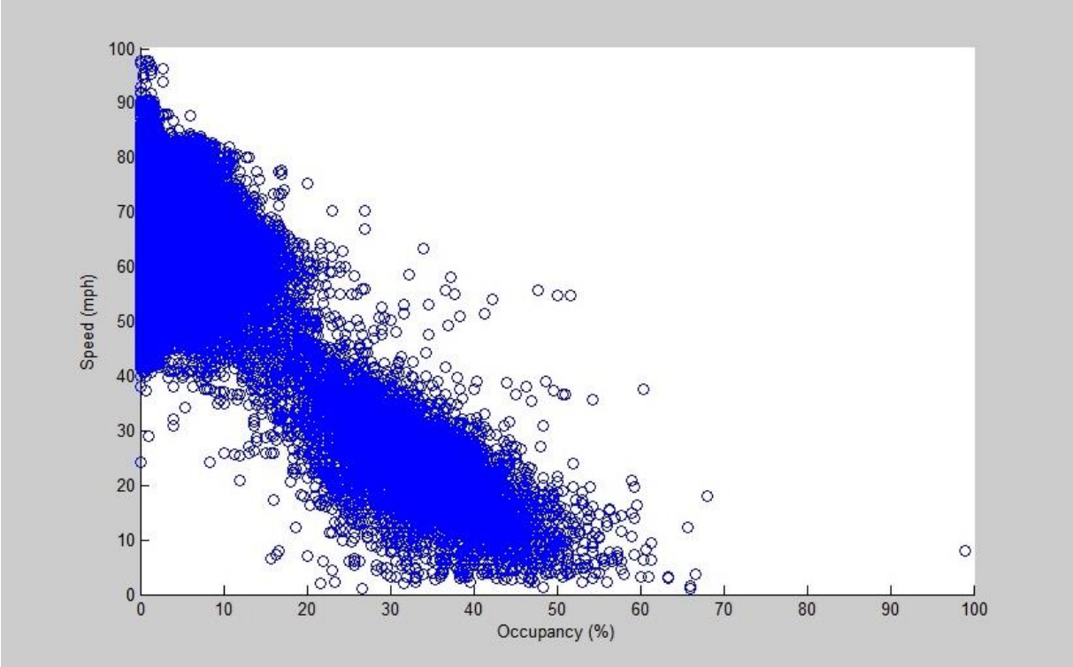
Figure 2.5 Q03: Speed-Occupancy Plot
