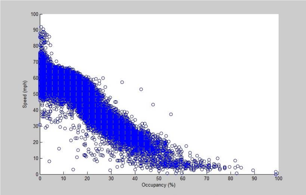
Figure 2.6 Q04: Speed-Occupancy Plot
