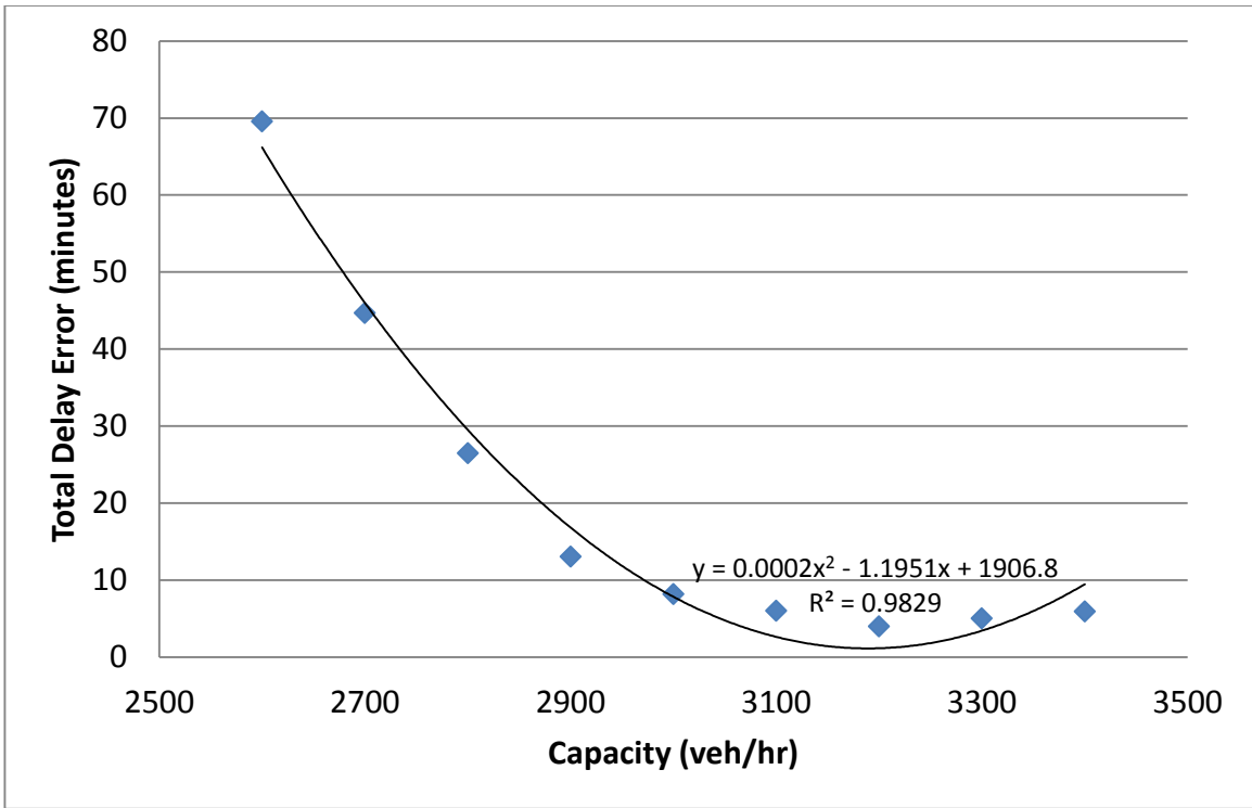
Figure 4.1 Delay error vs. capacity and least squares regression fit for July 10 th work zone data
