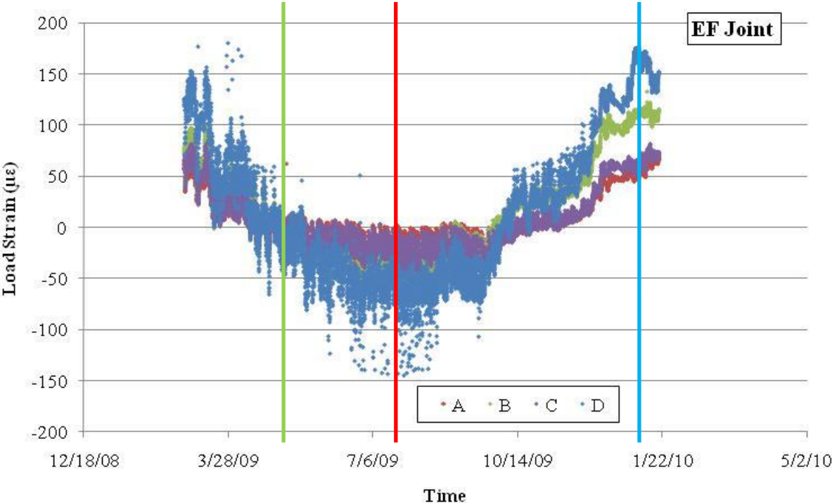
Figure 4.17. Load strain at EF joint
