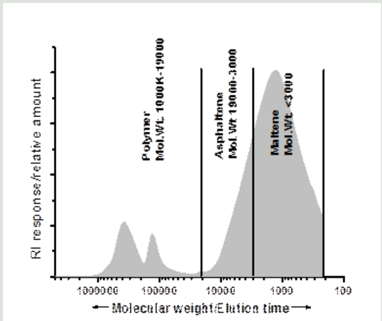
Figure 1 Molecular weight zones assigned in PMAC GPC Chromatogram
