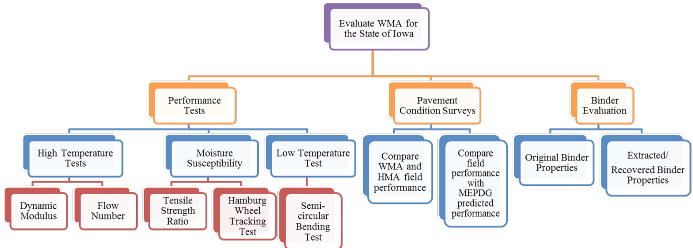
Conceptual diagram of Phase II scope and testing plan
