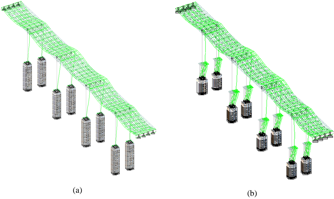
FIGURE 6.21 Deformation of the Bridge (a) before Scour and (b) after Scour with Scour Depth, S_s=5.3\text{m} (17.4 ft)
