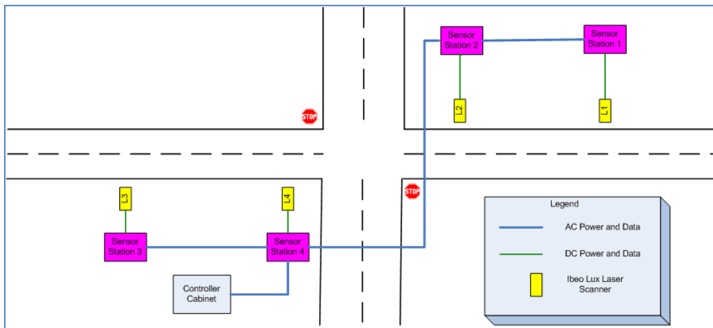
Figure 15: Proposed minimal sensor surveillance system hardware layout for rural two lane highway thru-stop intersections with Ibeo Lux Sensor
