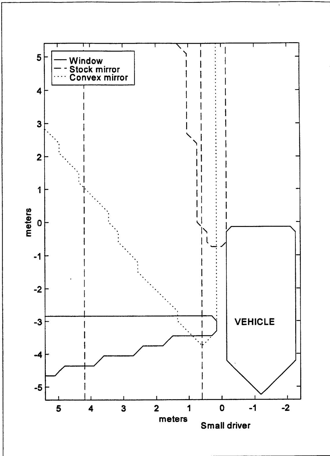
Figure 2.8. Driver's right side field of view for the HMMWV measured using a 5th percentile male driver
