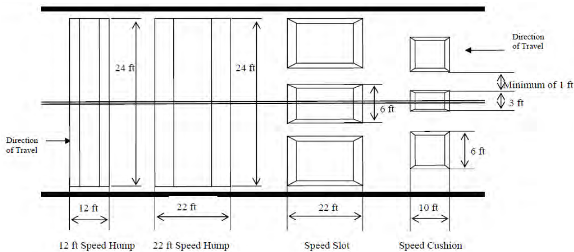
Figure 15: Comparison of speed hump, slot, and cushion (Johnson and Nedzesky, 2004)
