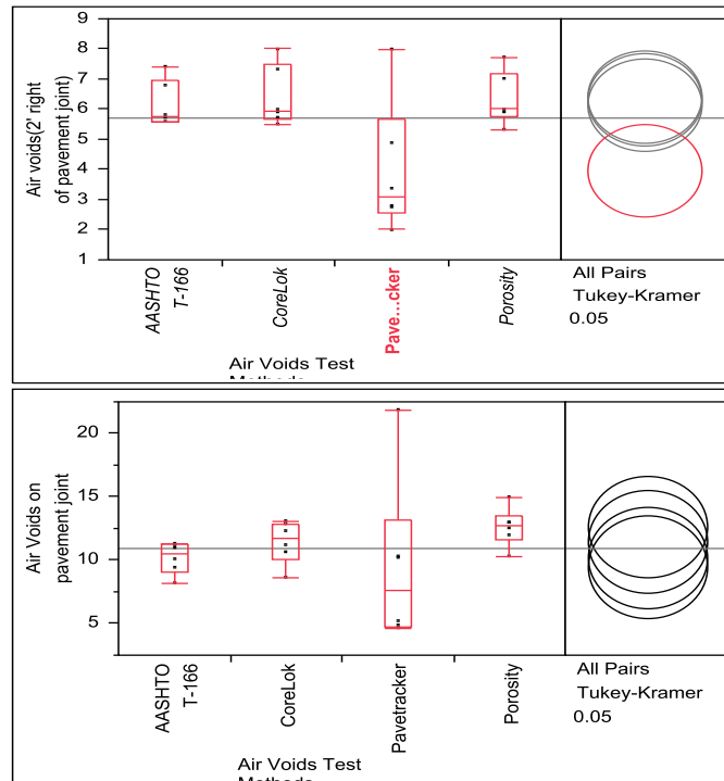
Figure 18. Comparison of air voids test methods by the HSD test for the US 61 project
