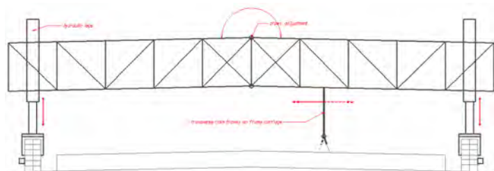
Figure 56. Schematic of transverse tining texture equipment
