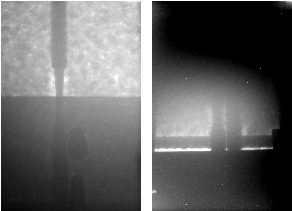
Figure 10. #6 Epoxy-coated reinforcing steel with simulated 50 percent corrosion loss at reference (left) and realistic (right) angles
