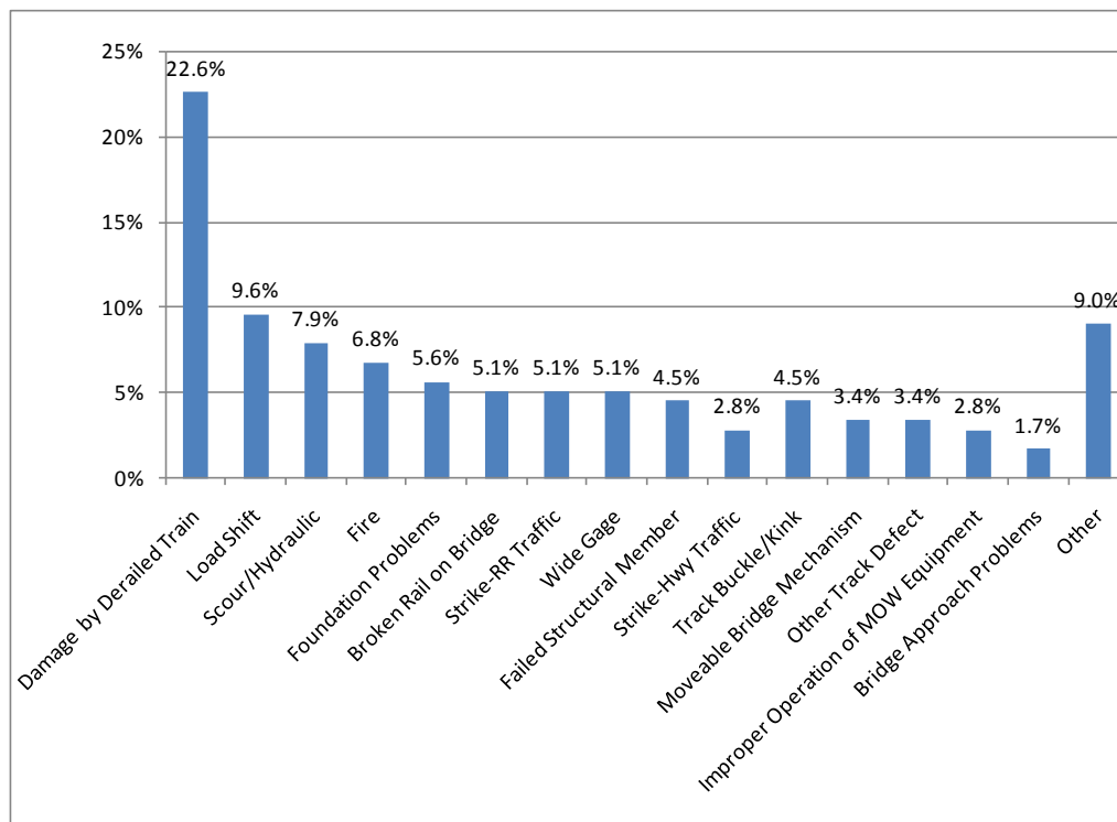
Figure 1. Frequency of FRA Reportable Accidents
