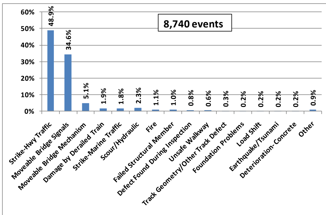
Figure 3. Frequency of Industry Bridge-Related Service Interruptions
