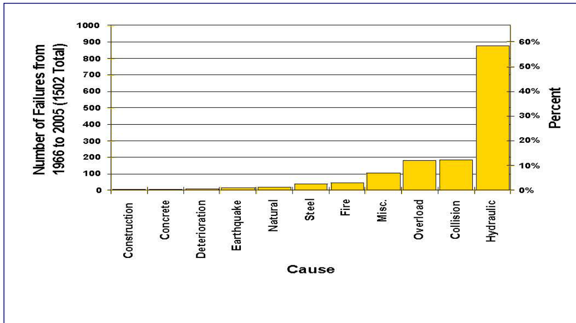
Figure 5. Highway Bridge Failures in United States from 1966 to 2005 (presented by Briaud – Texas Transportation Institute 39 )
