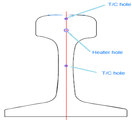
Figure 3. Diagram of End-Drilled Holes
