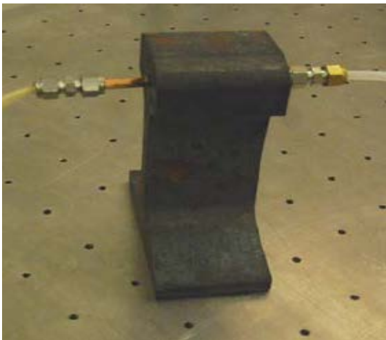
Figure 2. Instrumented Short Rail Section for Lab Test
