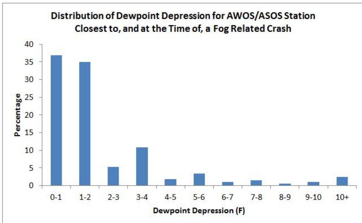
Figure 4.5: Distribution of dew-point depressions for AWOS/ASOS stations closest to and at the time of a fog-related crash
