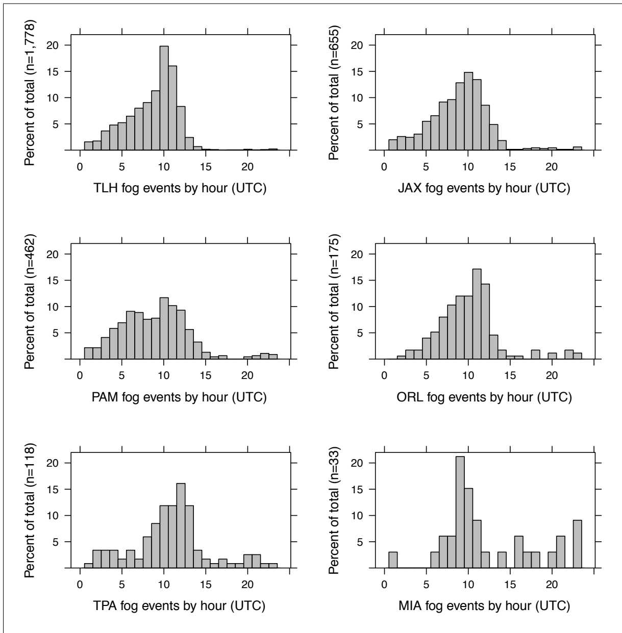
Figure 4.10: Fog occurrence by hour for selected site. EST=UTC-4 hours. EDT=UTC-5hours
