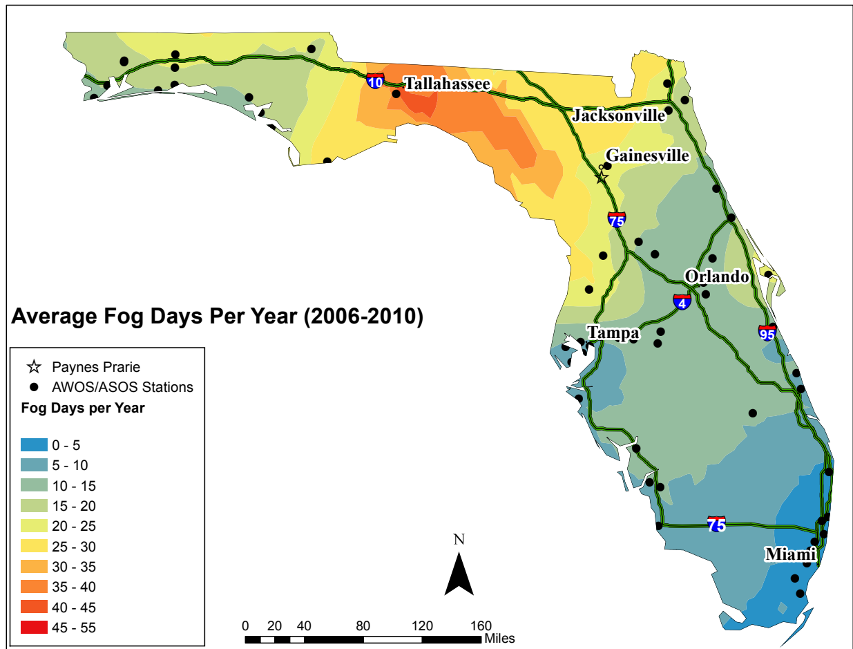
Figure 3.4: Climatological location and frequency of fog in Florida
