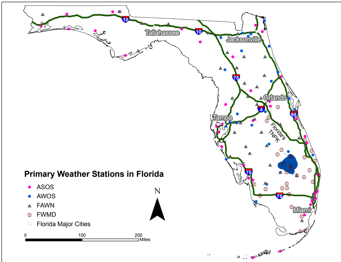
Figure 3.2: Primary Mesonet stations in Florida
