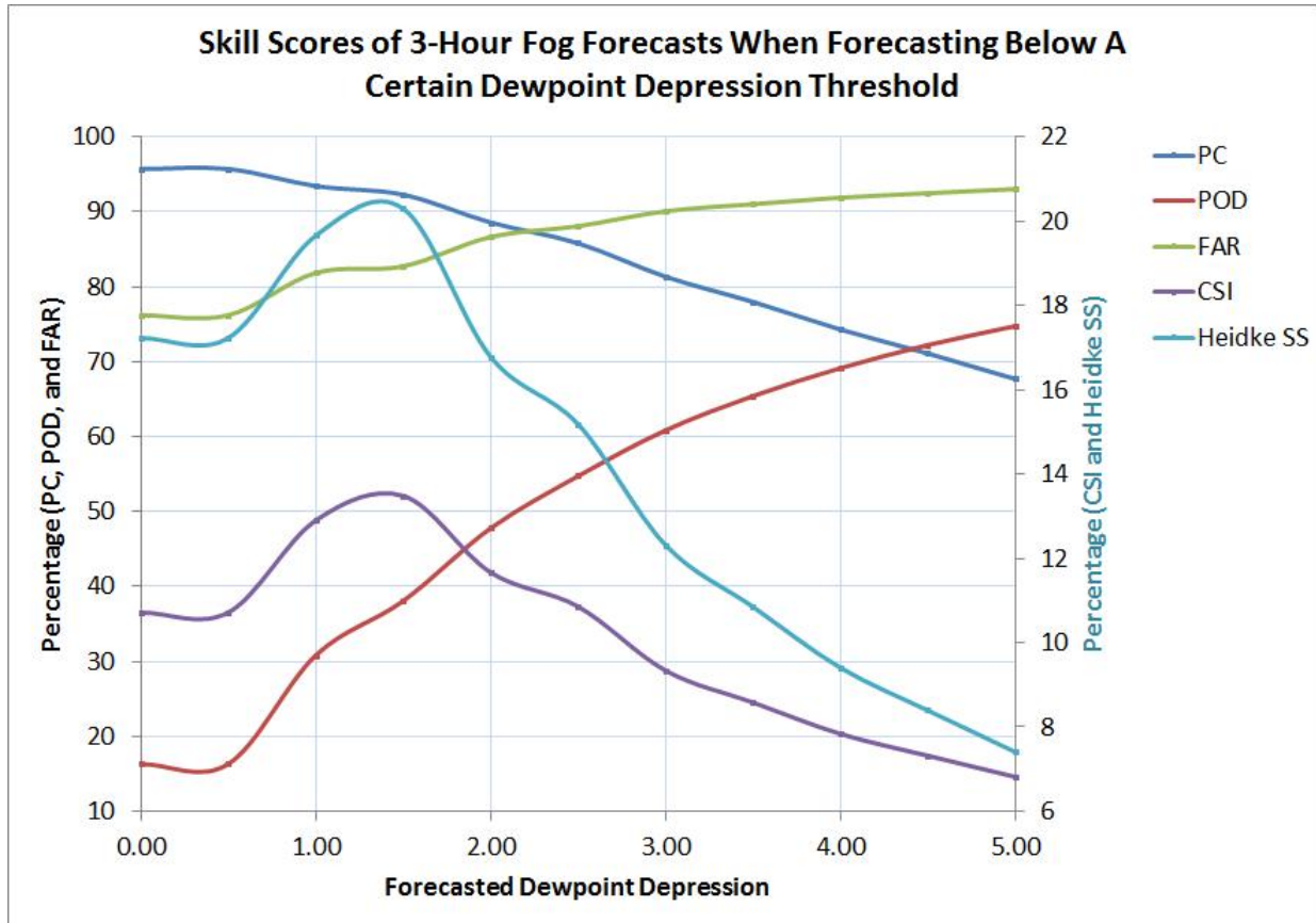
Figure 4.14: Three-hour forecast skill score
