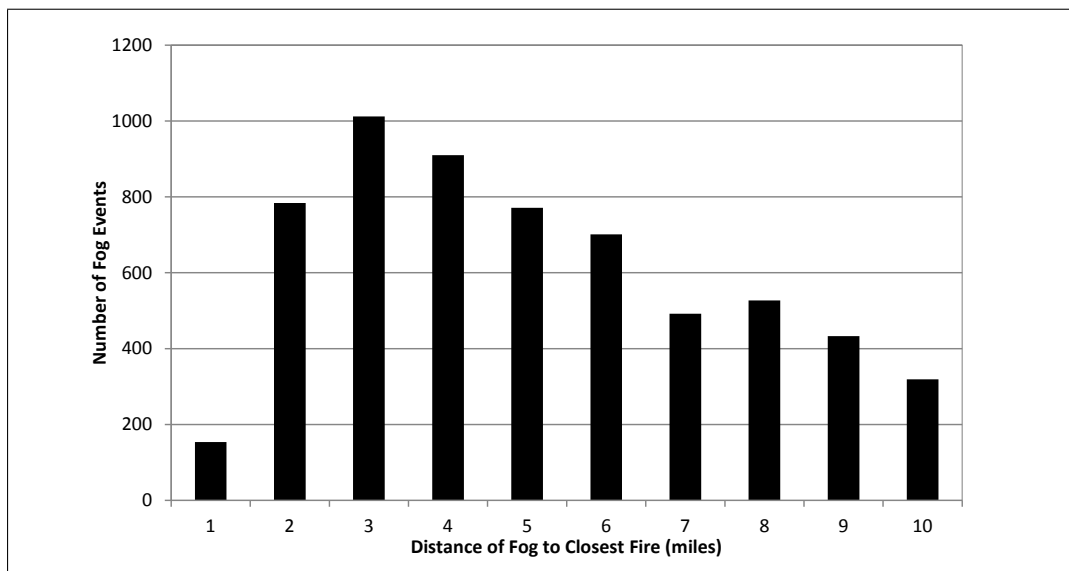
Figure 3.10: Distance in miles to the closest fire at the time of a fog-related crash
