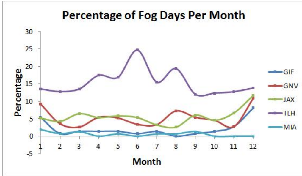
Figure 4.3: Percent of days with fog per month for selected locations
