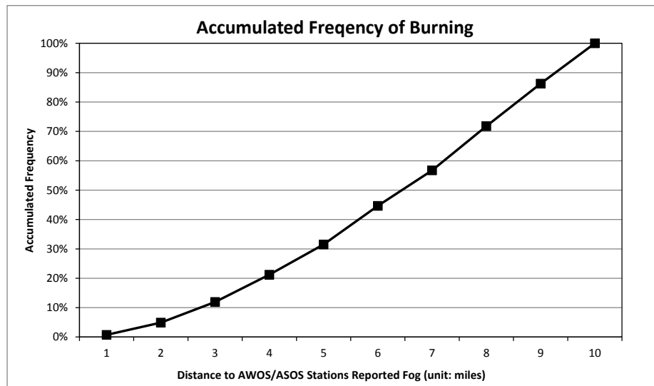
Figure 3.11: The cumulative fire distance to the closest ASOS station. For example, 70% of the fog events within 8 miles or less away from an ASOS or AWOS station
