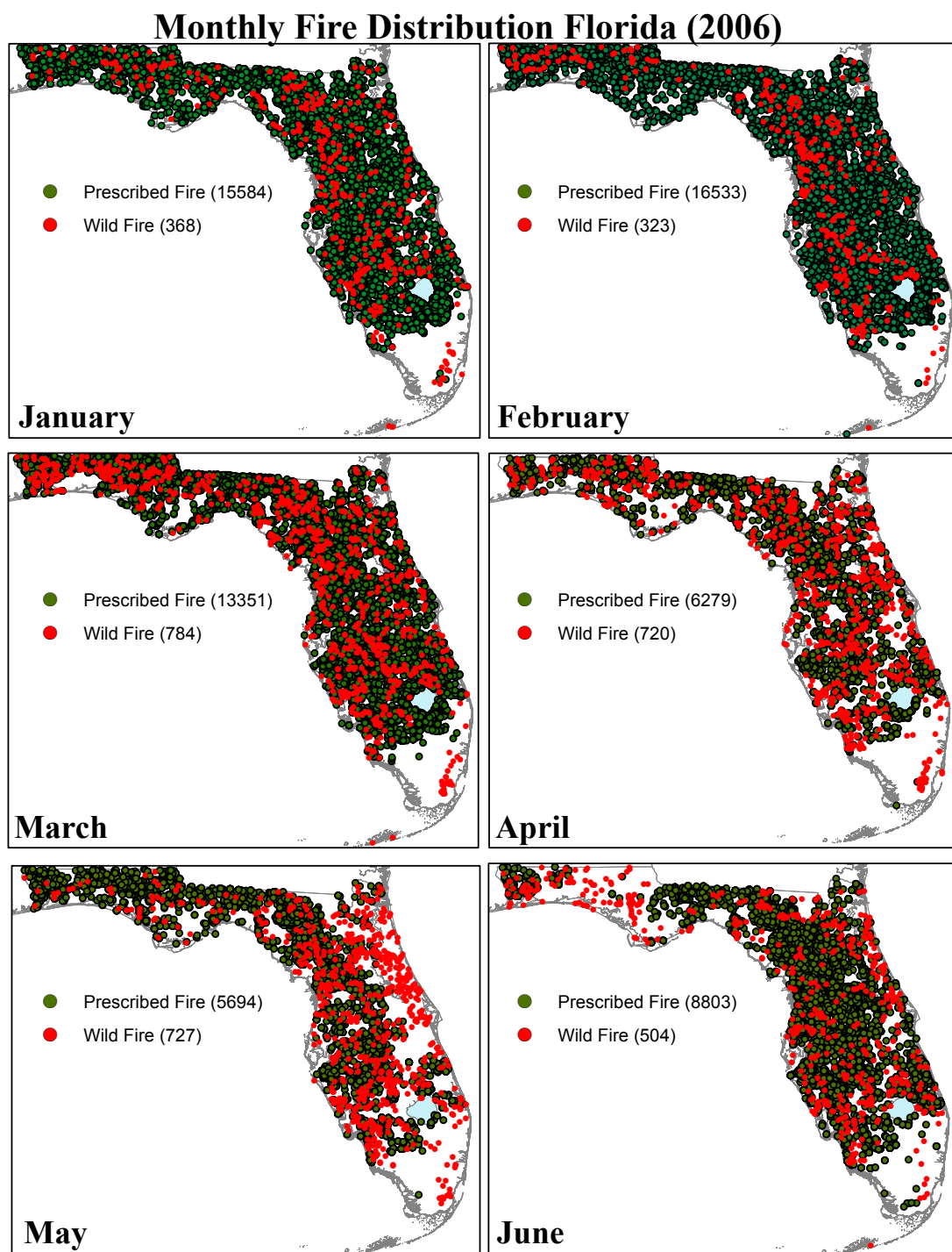
Figure 3.7: Controlled burns and wild fires during the first six months of 2006
