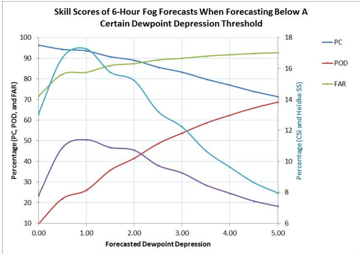
Figure 4.13: Six-hour forecast skill score
