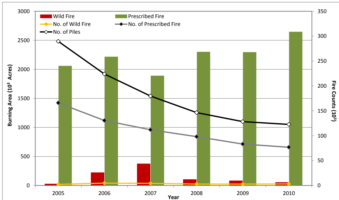
Figure 3.9: Fire counts and area burned during a 6-year period for wild fires and controlled burns
