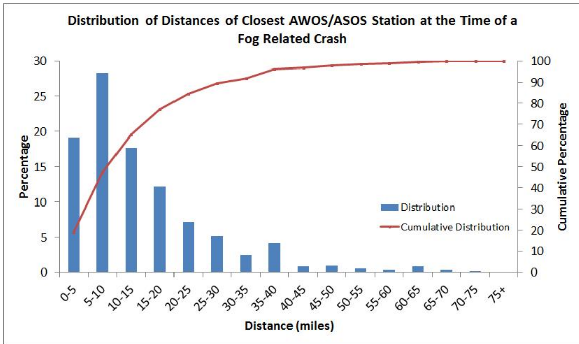
Figure 4.1: The distribution distance in miles from crash to the closest AWOS/ASOS station
