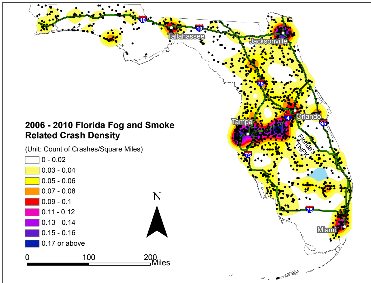
Figure 3.14: Location of all fog- and smoke-related crashes
