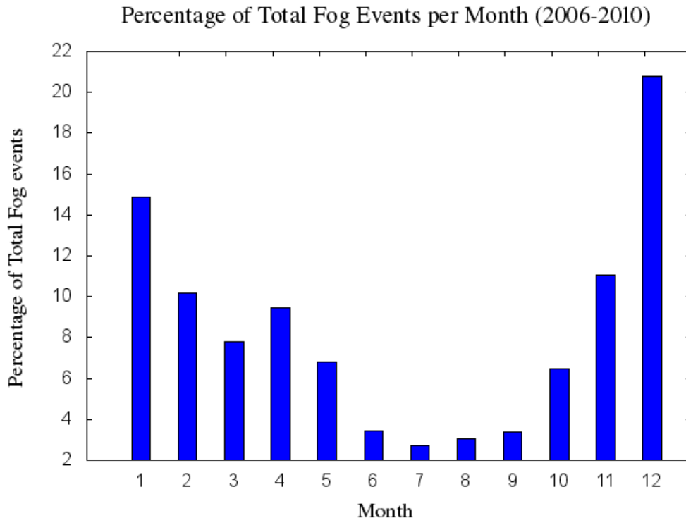
Figure 3.5: Percent of the total fog occurrence given by month of the year
