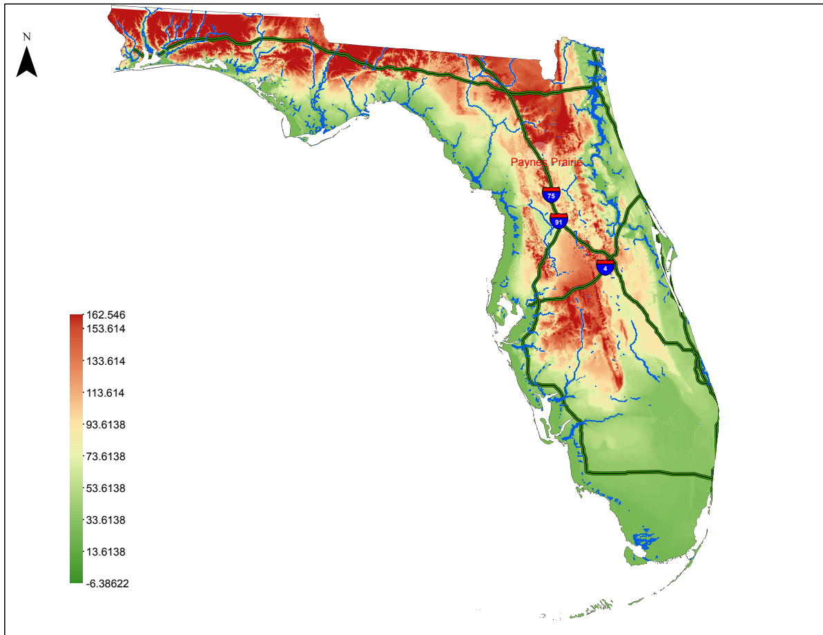
Figure 3.3: Topography of Florida
