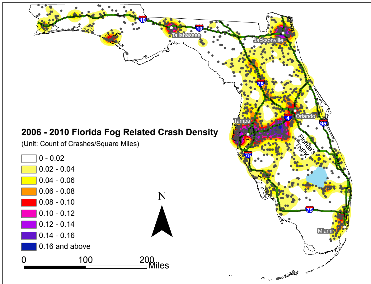
Figure 3.13: Crash density due only to fog.
