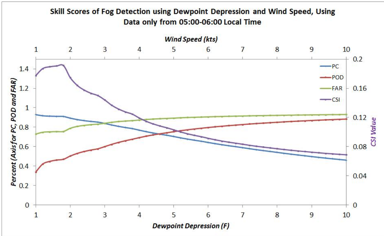
Figure 4.7: Skill scores of fog detection using dew-point depression and wind speed from 5:00 a.m. – 6:00 a.m. local time
