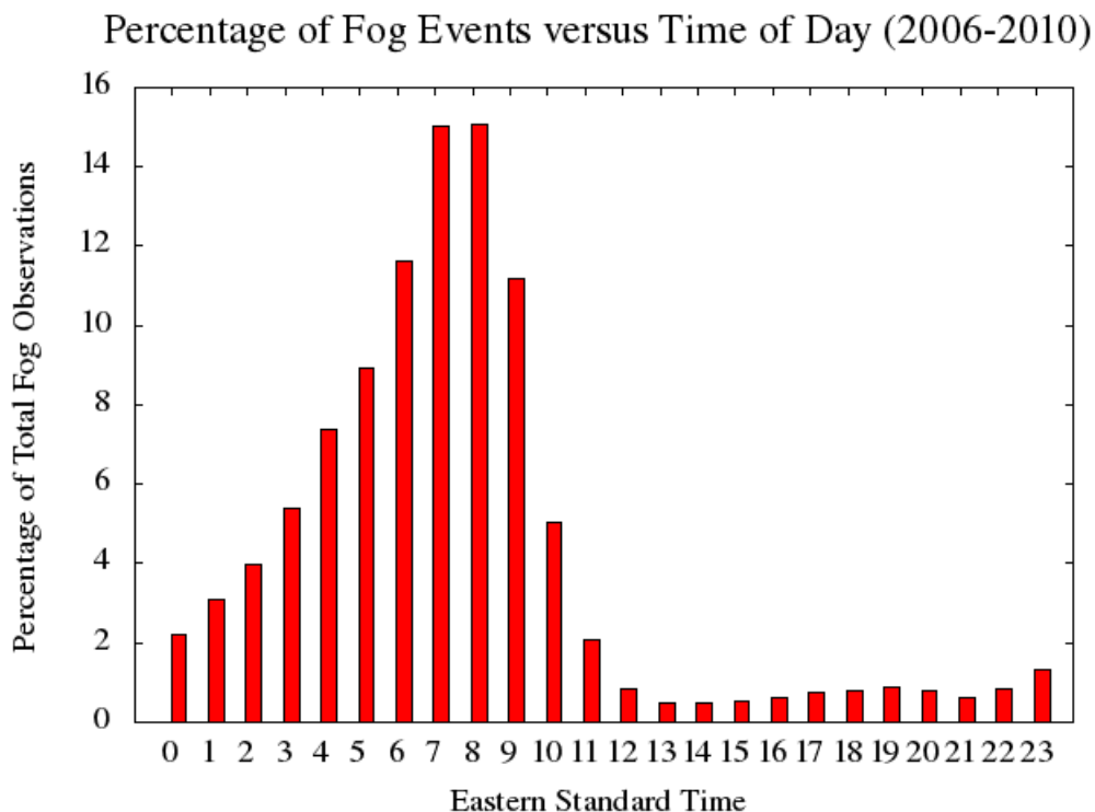
Figure 3.6: Percent of total fog occurrence given by the time of day
