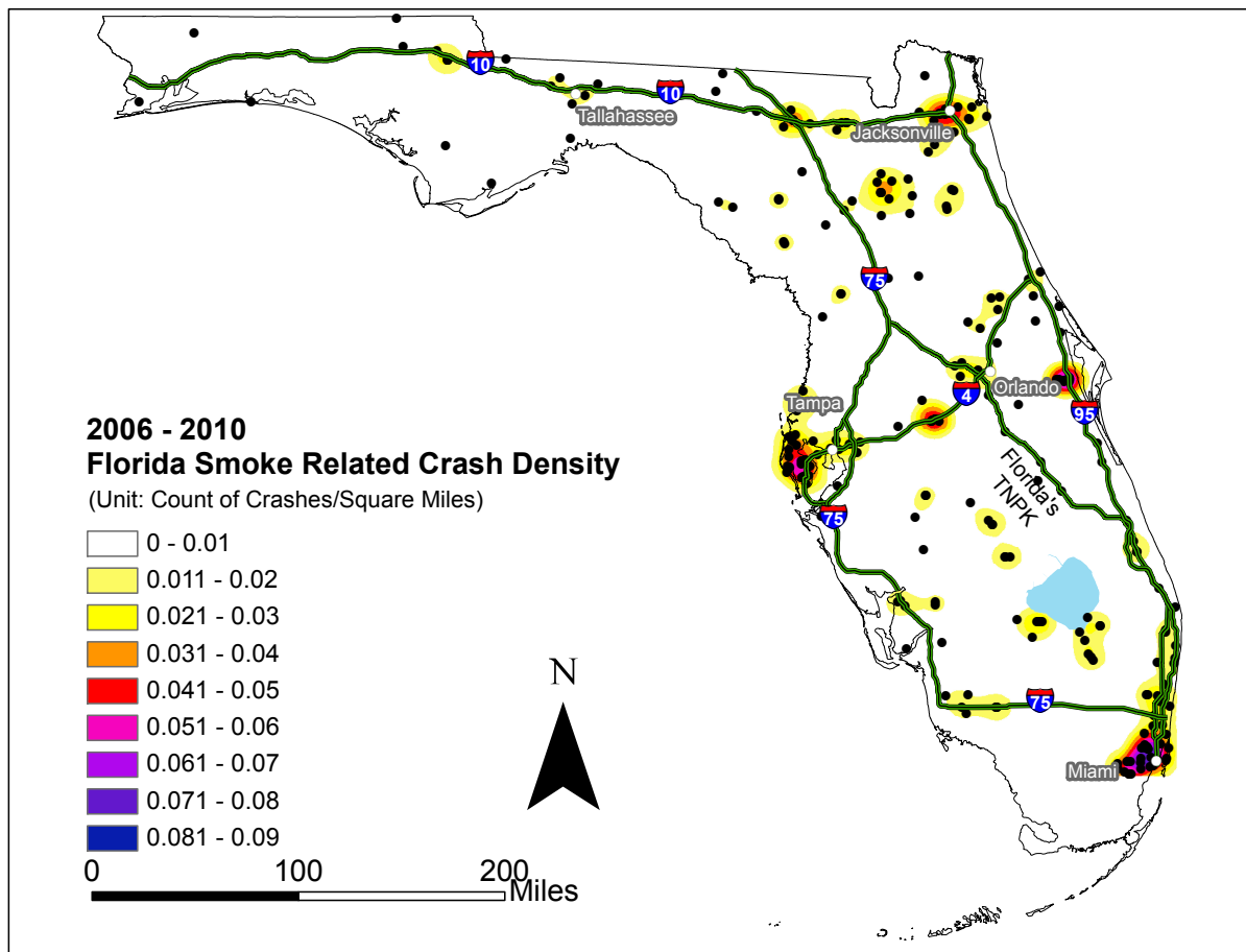
Figure 3.12: Crash density due only to smoke
