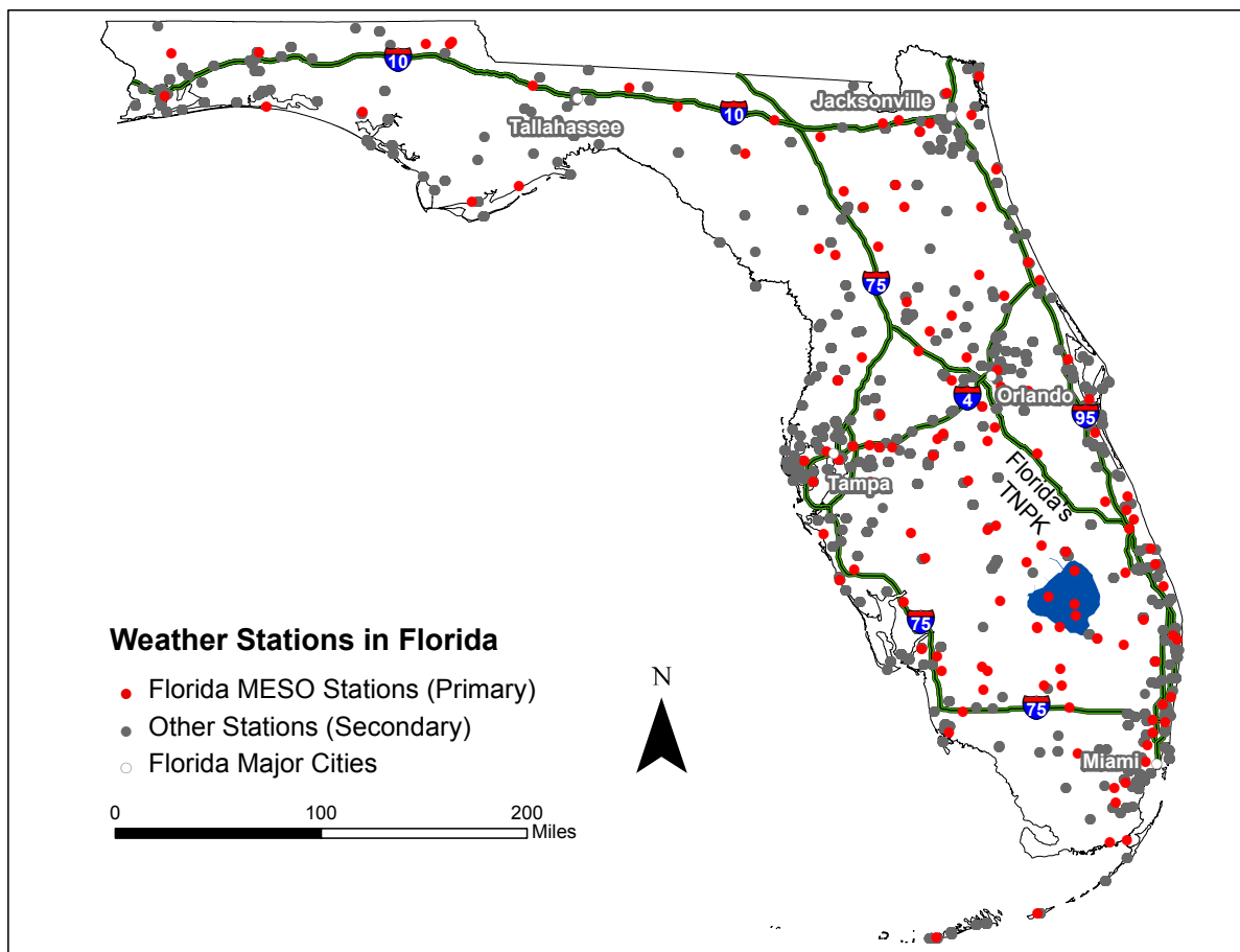
Figure 3.1: All Mesonet stations in Florida
