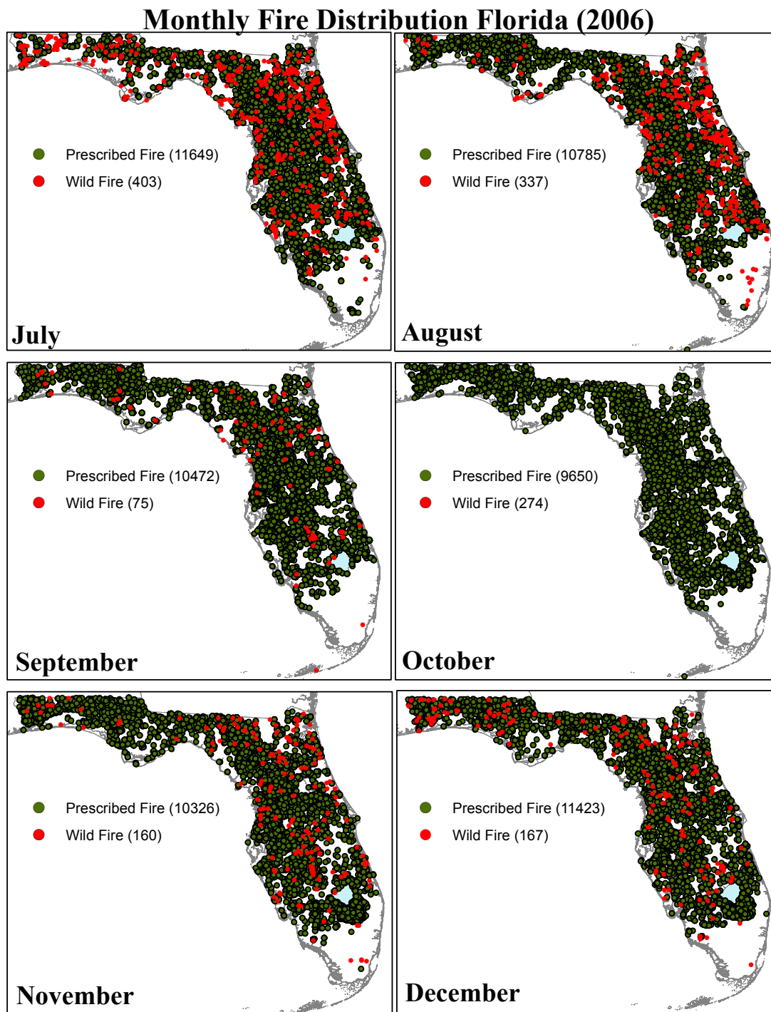
Figure 3.8: Controlled burns and wild fires during the last six months of 2006
