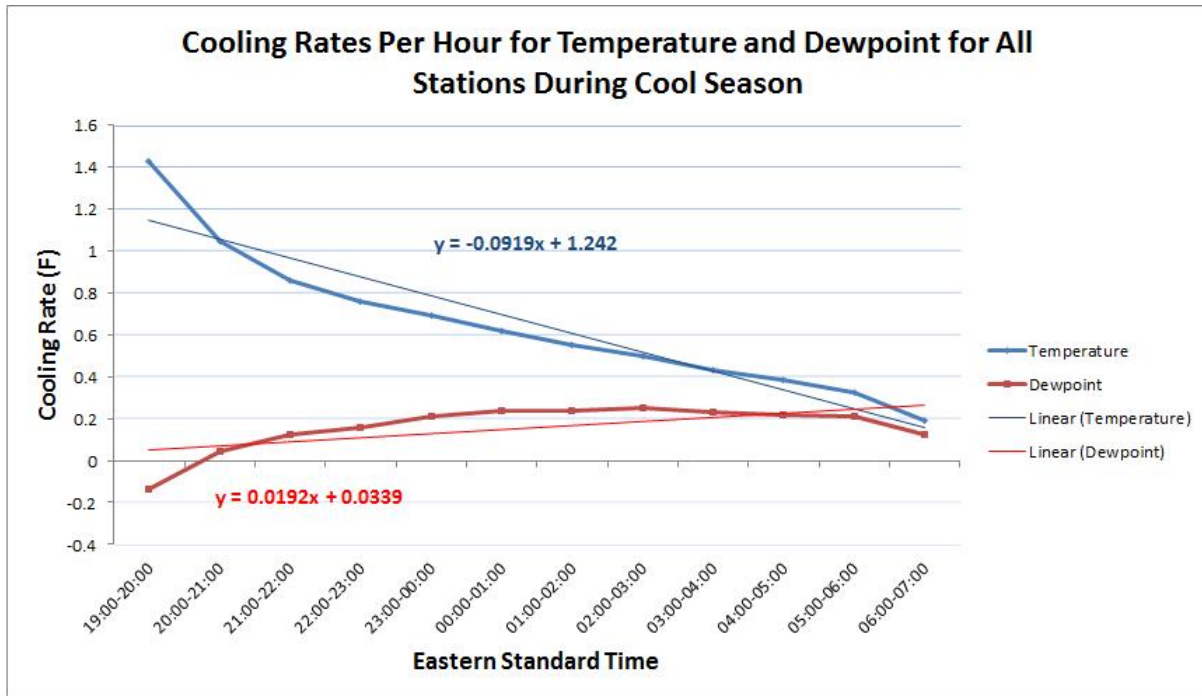
Figure 4.8: Rate of cooling of the temperature expected (averaged over all station and for five years during the cool months
