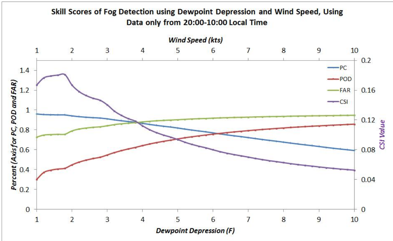
Figure 4.6: Skill scores of fog Detection using dew-point depression and wind speed from 20:00 p.m. – 10:00 a.m. local time
