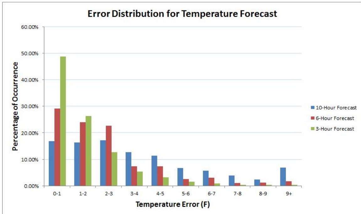
Figure 4.9: Forecast temperature error
