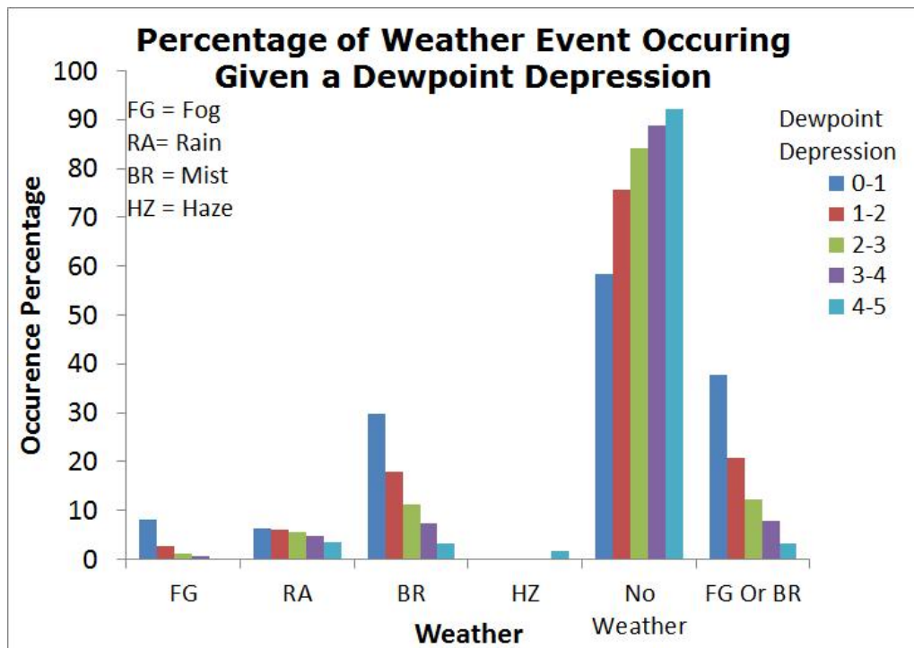
Figure B.1: Percent of type of weather event for specific dew-point depressions
