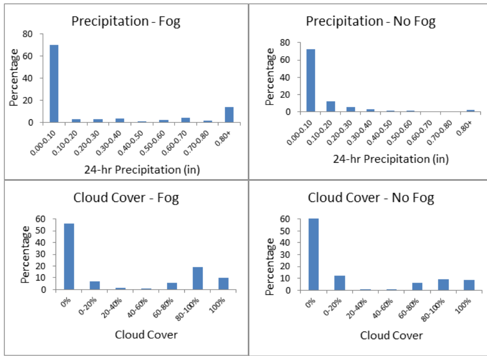
Figure B.4: Fog cover vs different measured variables continued
