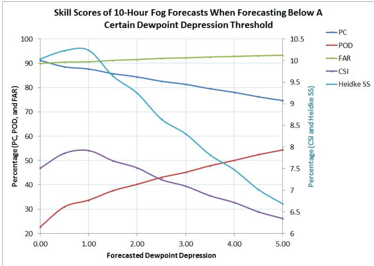
Figure 4.12: Ten-hour forecast skill score
