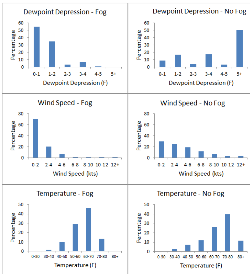
Figure B.3: Fog cover vs different measured variables
