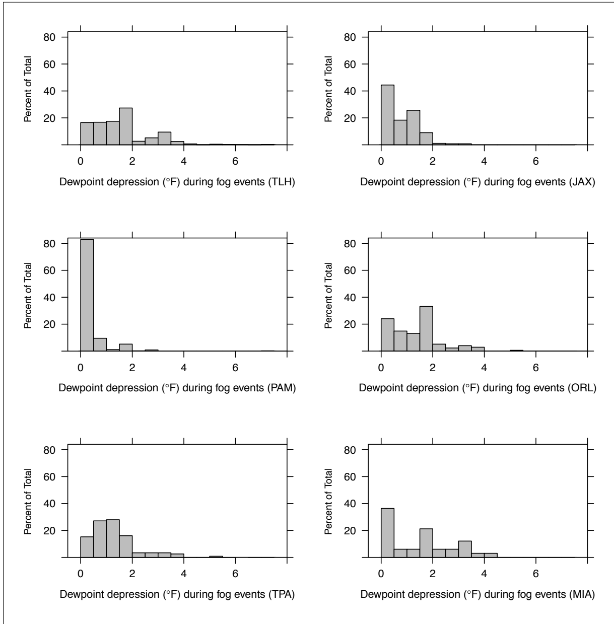
Figure 4.11: Fog dew point depression on nights when fog occurred (EST)
