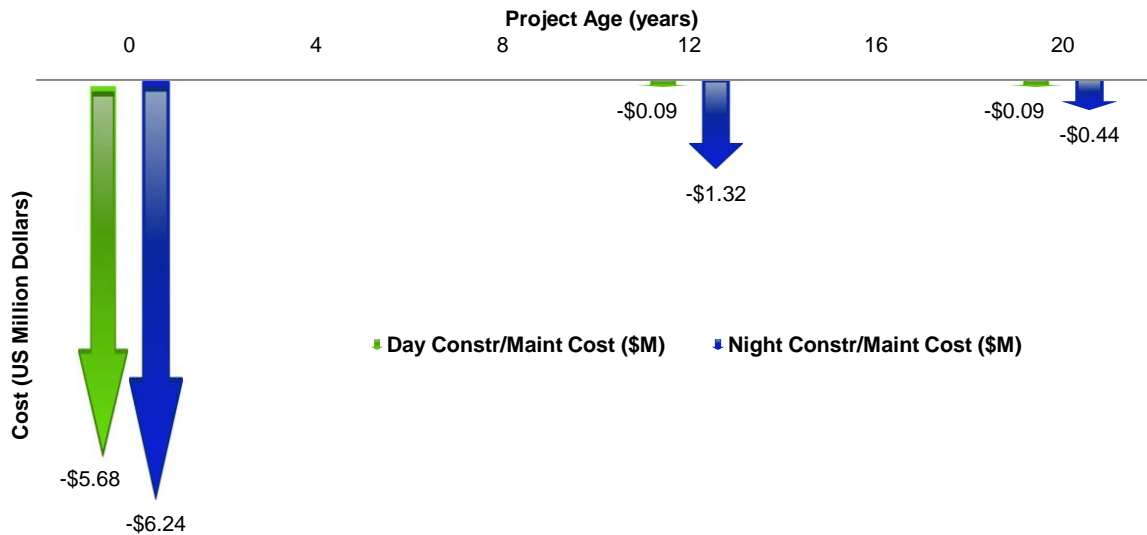
Figure 6-2. cash flow diagram for day and night LCCA
