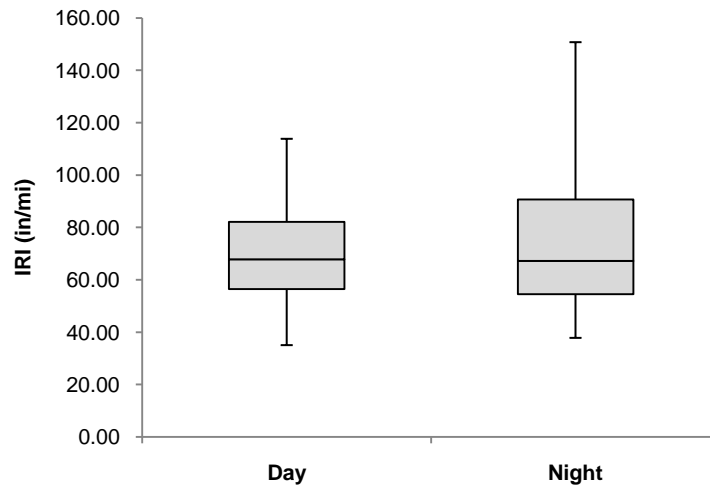
Figure 5-3. boxplot: all day and night project IRI values
