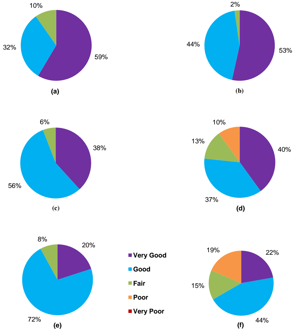
Figure 5-9 (a)-(f). pie charts: pavement condition frequencies for (a) day IRI values <30 months, (b) night IRI values <30 months, (c) day IRI values 31-60 months (d) night IRI values 31-60 months, (e) day IRI values 61-90 months (f) night IRI values 61-90 months
