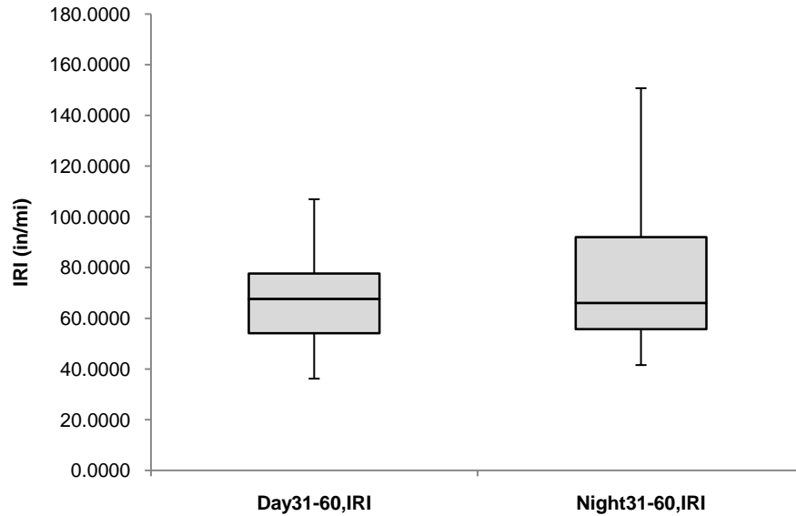
Figure 5-7. boxplot: day and night IRI values—interval 2
