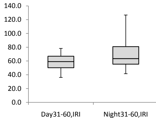
Figure L-2. \geq 3 IRI Projects' Day and Night IRI values calculated between 31 and 60 months after project completion
