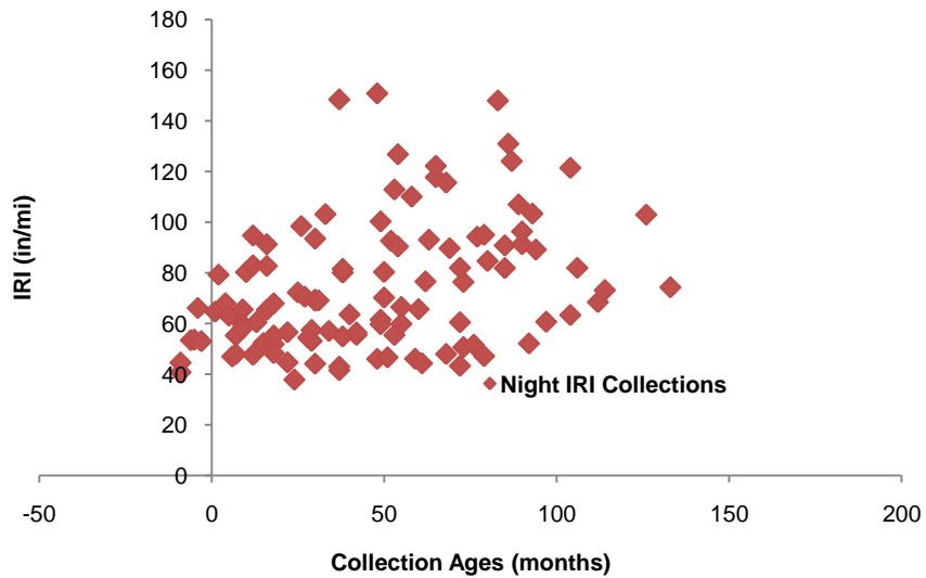
Figure 5-5. all nighttime IRI values over time
