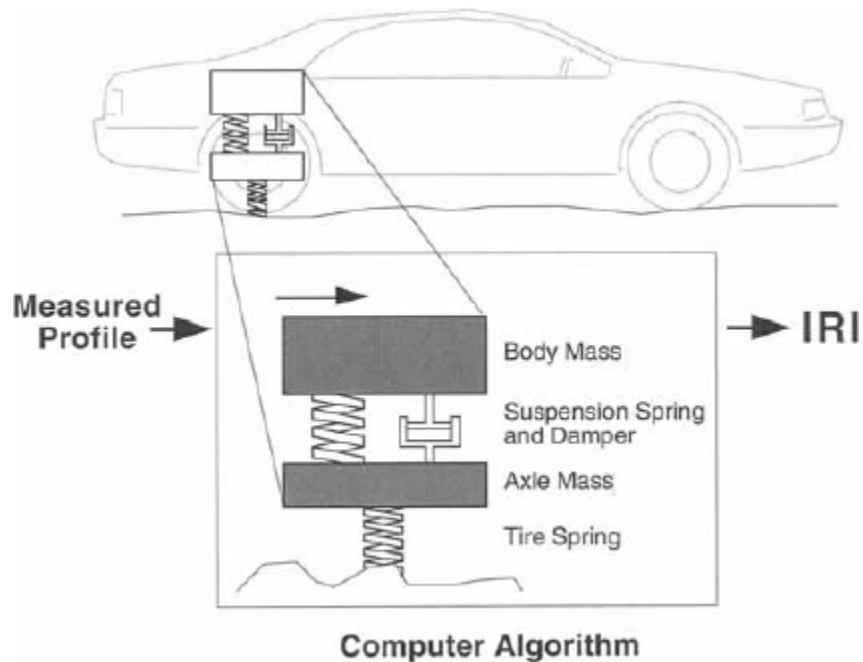
Figure 2-1. representation of IRI algorithm calculation (Sayers & Karamihas, 1998)
