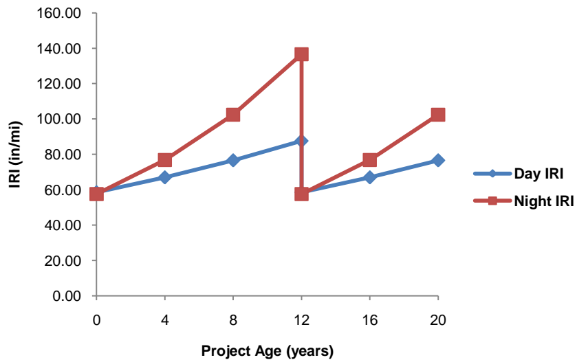
Figure 6-1. IRI progression for LCCA
