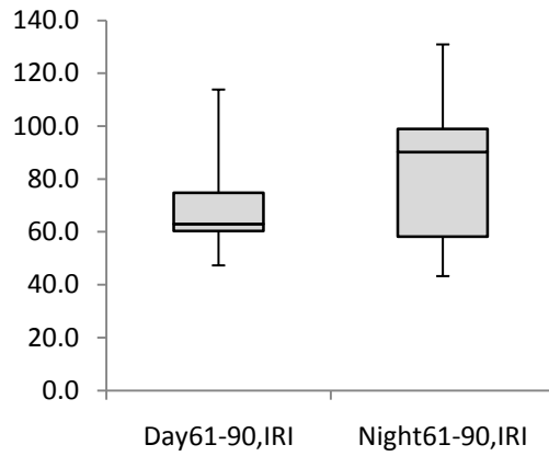
Figure L-3. \geq 3 IRI Projects' Day and Night IRI value collected between 61 and 90 months after project completion.
