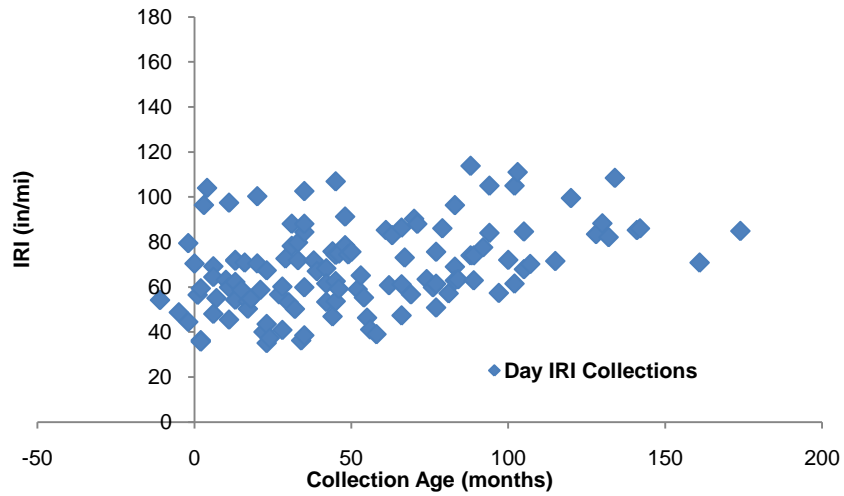
Figure 5-4. all daytime IRI values over time
