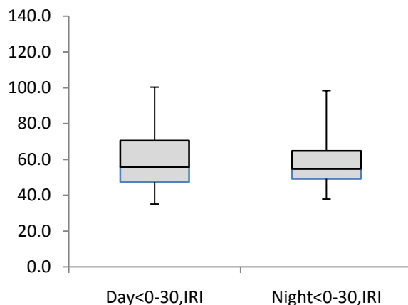
Figure L-1. ≥3 IRI Projects' Day and Night IRI values from collections within the first 30 months after project completion.
