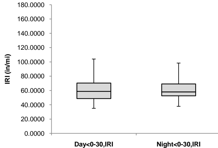
Figure 5-6. boxplot: day and night IRI values—interval 1
