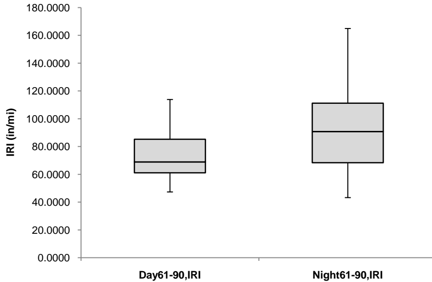
Figure 5-8. boxplot: day and night IRI values—interval 3
