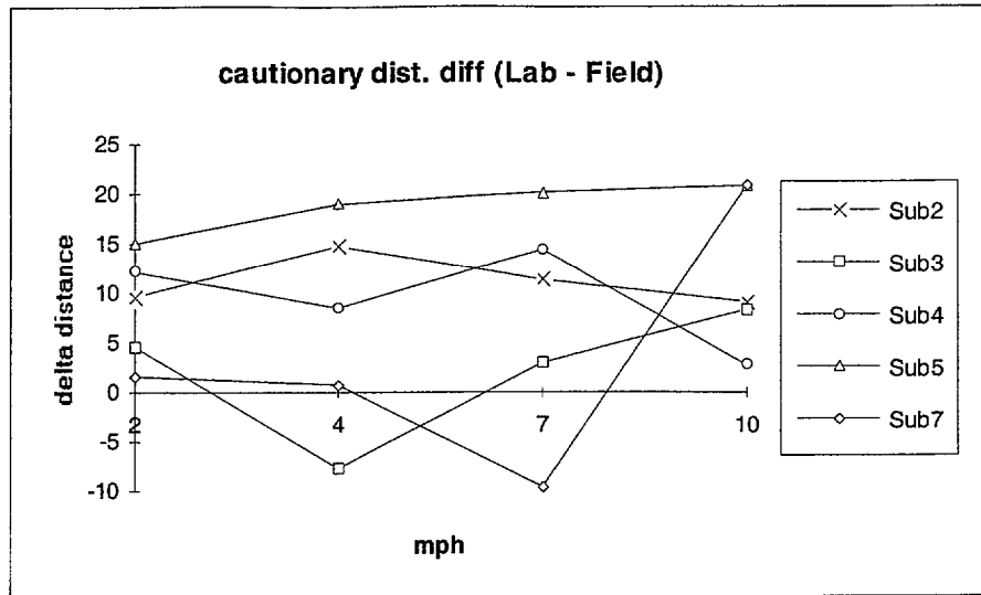
Figure 3-6 Cautionary distance difference between lab and field conditions for each participant.
