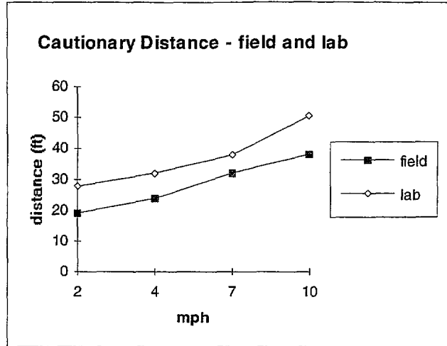
Figure 3-5 Cautionary warning zone distances for all participants in field and lab conditions.
