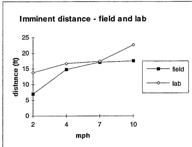
Figure 3-4 Cautionary warning zone distances for all participants in field and lab conditions.
