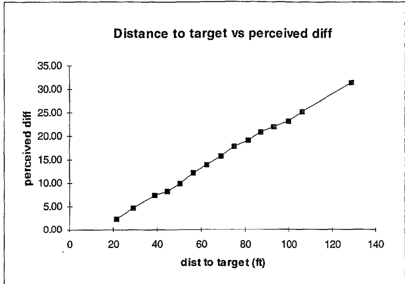
Figure 3-11 The perceived distance difference between the field and lab conditions for different distances from the target. (The target appeared closer in the lab) (ex. when the dummy was 100 feet away in the lab and the field it appeared 25 feet close in the lab).
