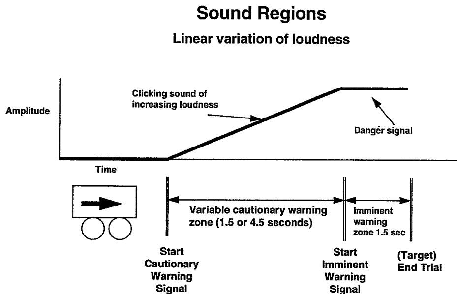
Figure 4-2 Example of linear variation of loudness.
