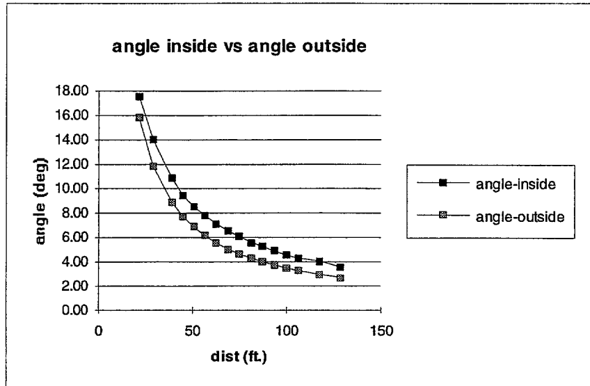
Figure 3-10 Visual angle comparison between lab and field conditions.
