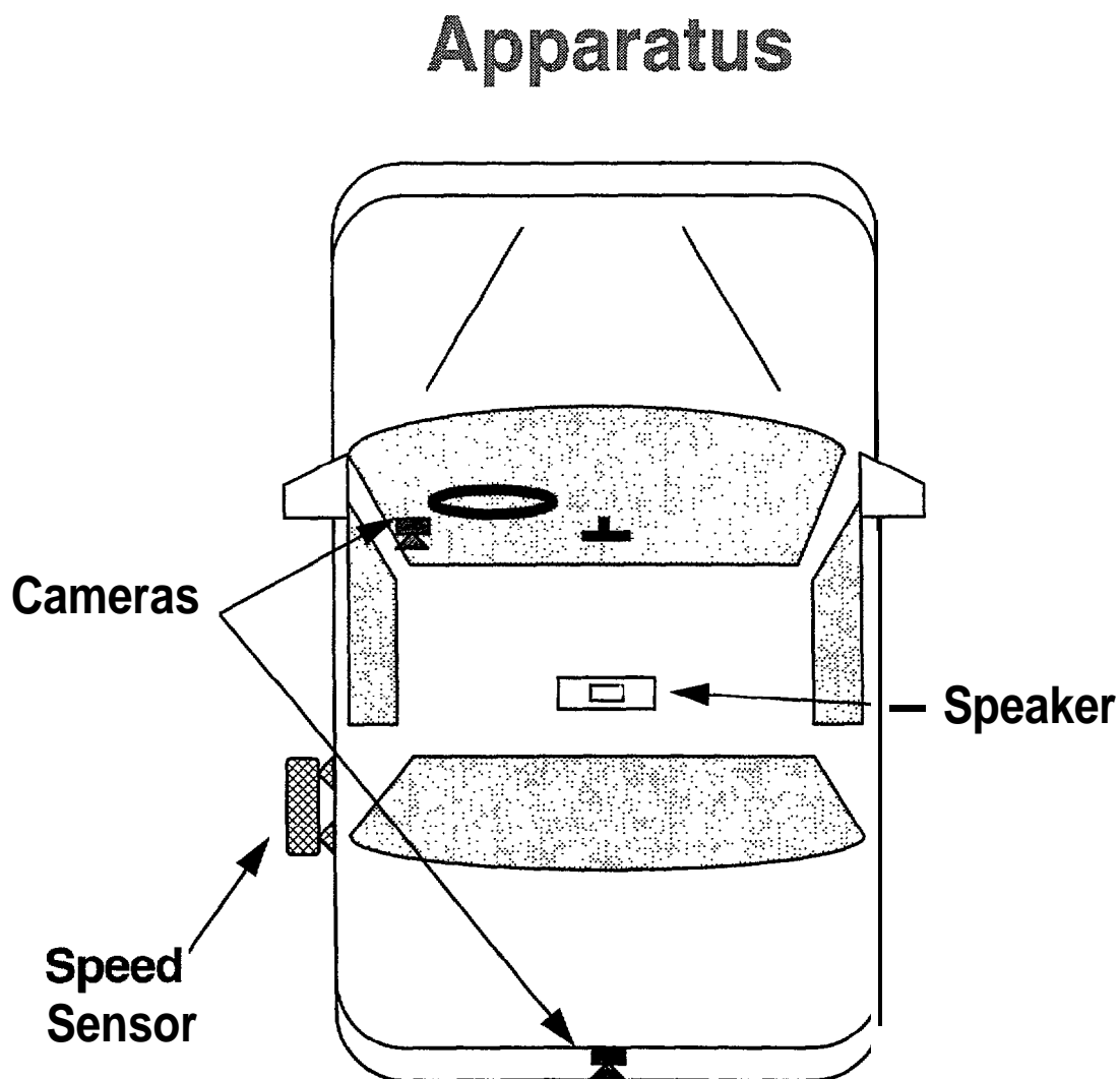
Figure 2-1 Location of equipment in vehicle
