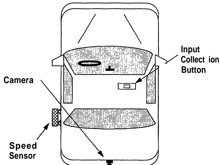
Figure 3-1 Location of equipment in vehicle
