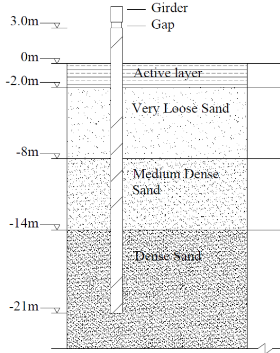
Figure 4.1. The soil-pile system of a typical bridge foundation system used in Alaska
