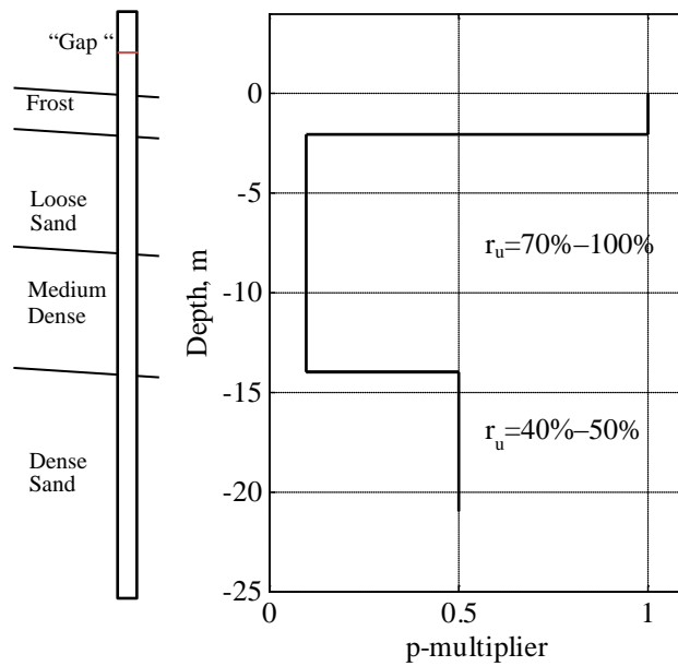
Figure 5.3. P-multipliers distribution along pile depth
