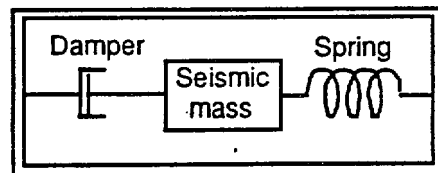
Figure 3-2 Acceleration Transducer
