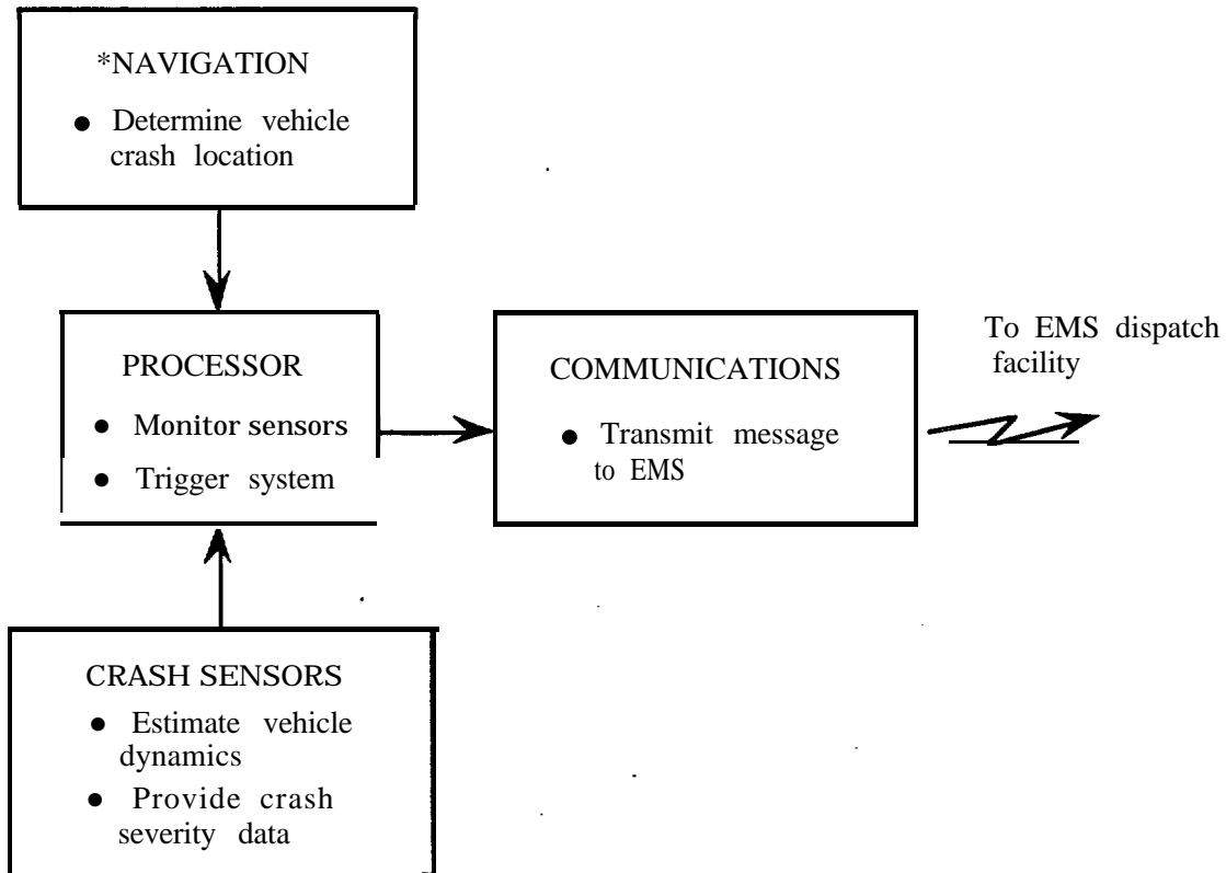
Figure 1-1 ACN In-Vehicle Component Functional Block Diagram
