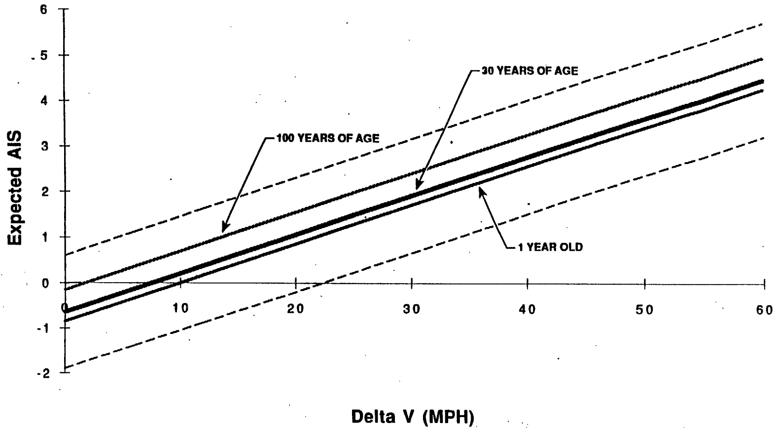
Figure C-5 Range of Expected Injury versus Age for a Frontal Impact
