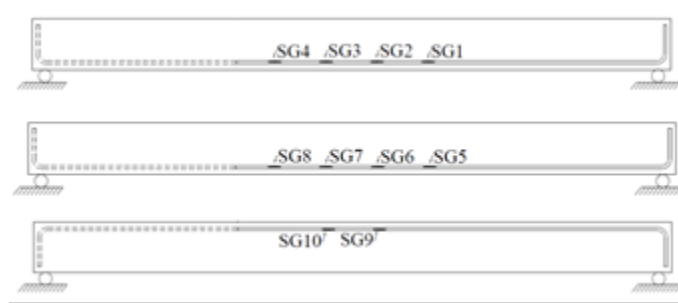
Figure 2-2. Longitudinal Strain Gage Locations.
