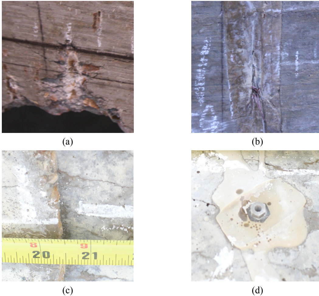
Figure 6-4. Examples of Surface Irregularities within the Testing Grid: (a) Damage from Lifting Chains, (b) Rough Surface, (c) Surface Discontinuity, and (d) Demountable Mechanical (DEMEC) Measurement Point.
