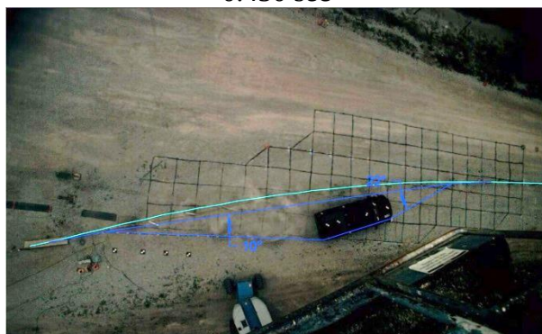
Figure 33. Cable Position and Vehicle Trajectory – Test No. NYCC-3
