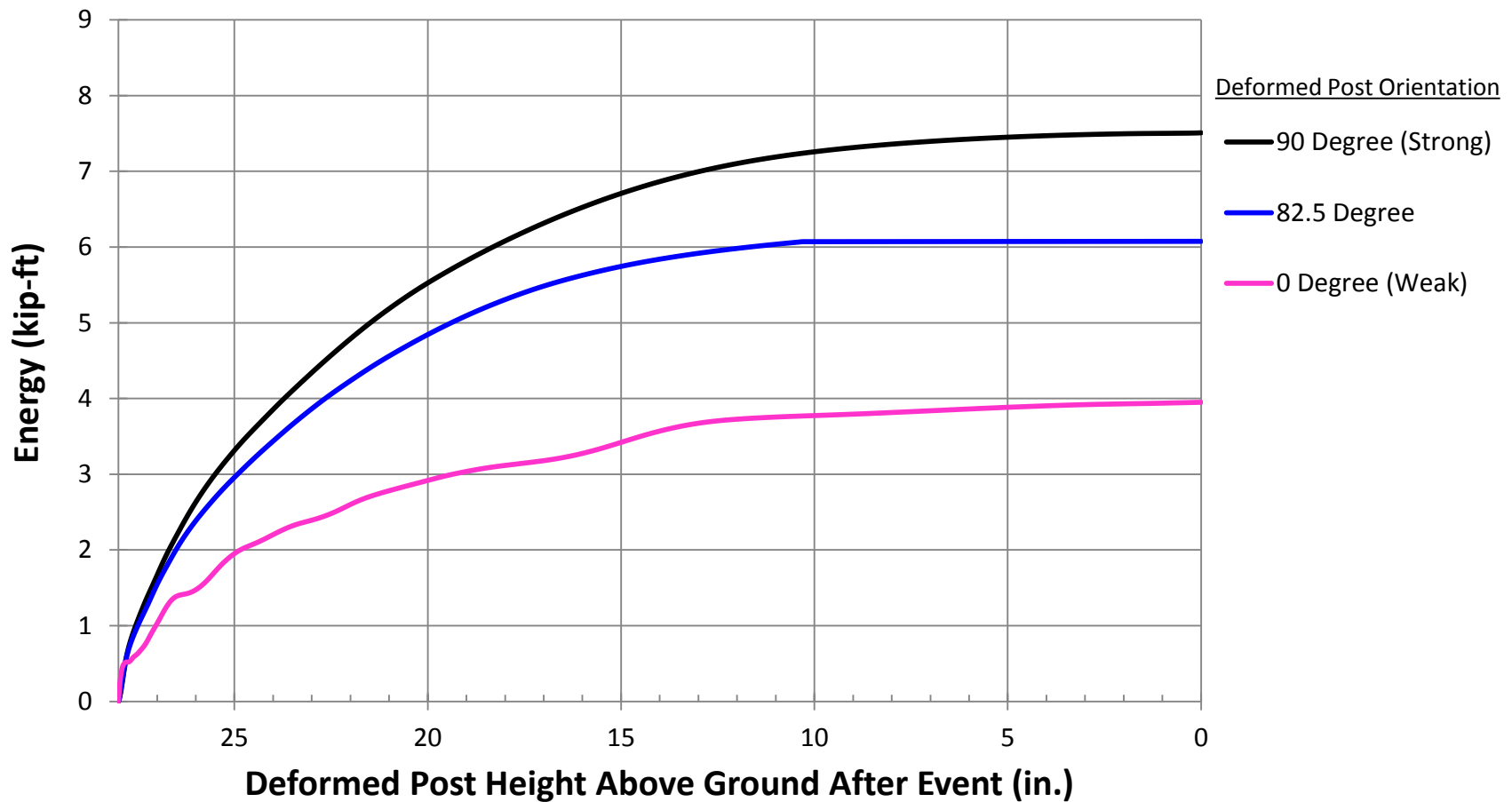
Figure 19. Energy vs. Deformed Post Height – S3x5.7 (S76x8.5) Posts in Soil - Post Height 28 in. (711 mm)
