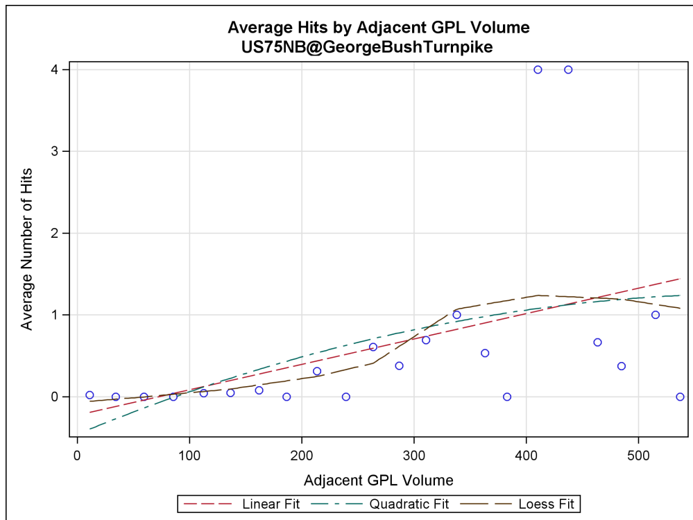
Figure H-19. Regression Trend between Hits vs. Adjacent GPL Volume for US 75 NB HOV Tangent at George Bush Turnpike.
