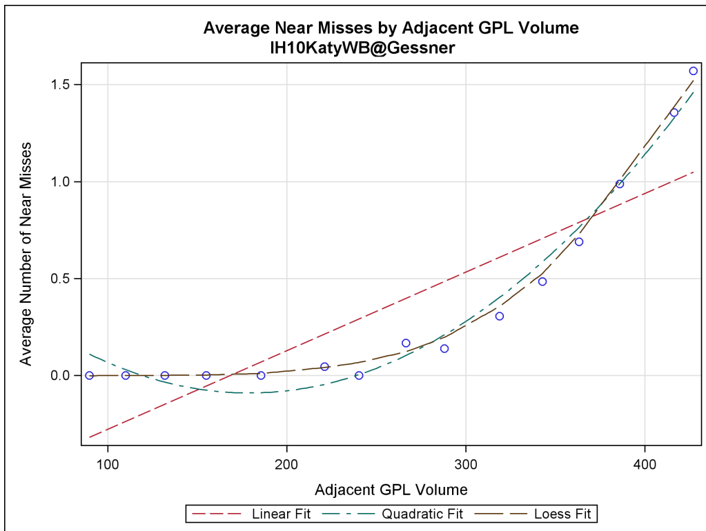
Figure H-7. Regression Trend between Near Misses vs. Adjacent GPL Volume for IH 10 WB Managed Lanes at Gessner.
