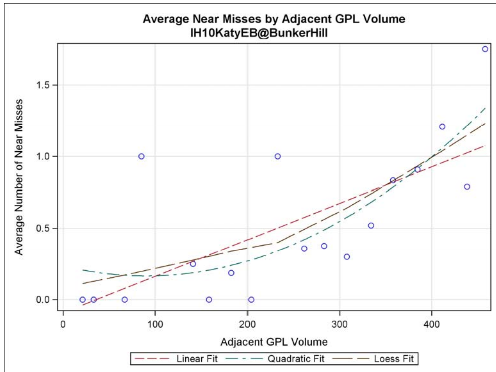
Figure H-5. Regression Trend between Near Misses vs. Adjacent GPL Volume for IH 10 EB Managed Lanes at Bunker Hill.
