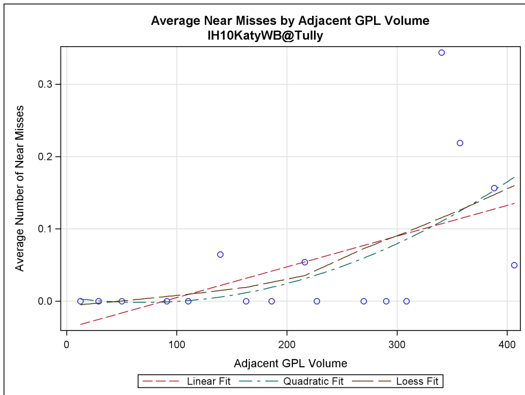
Figure H-15. Regression Trend between Near Misses vs. Adjacent GPL Volume for IH 10 WB Exit from Managed Lane at Tully.
