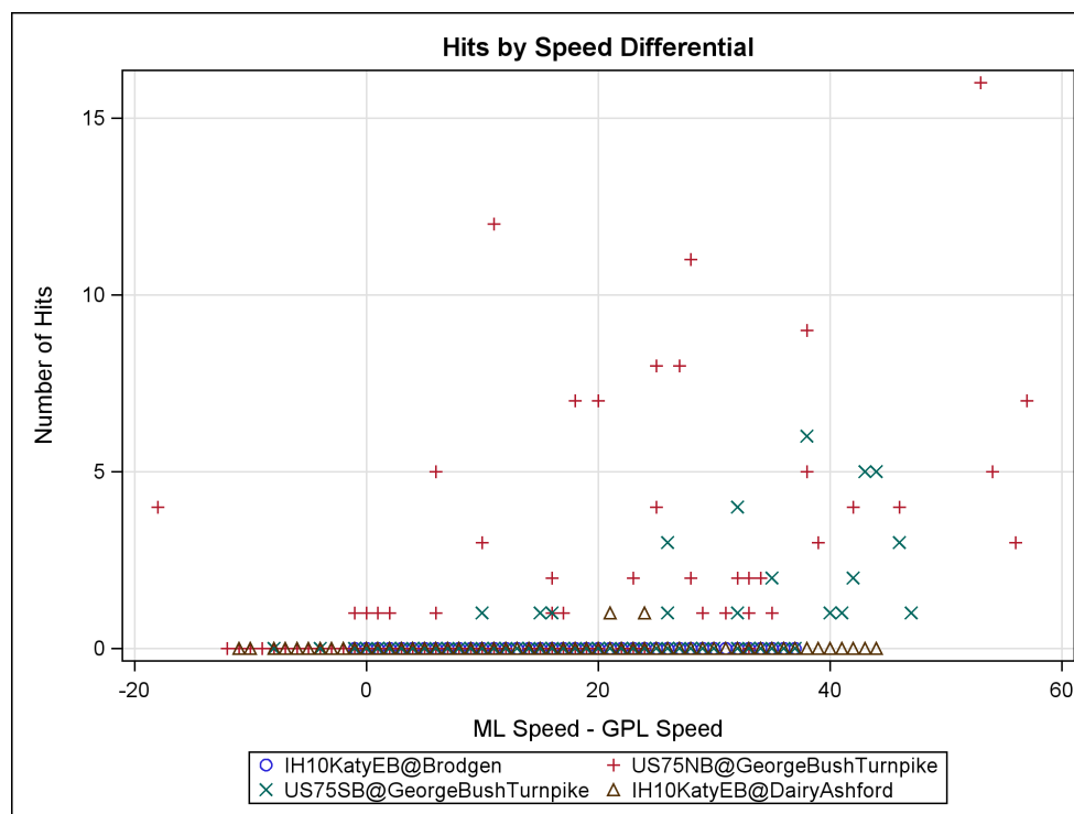
Figure I-4. Scatter Plot of Hits vs. Speed Differential between ML and GPL for Preferential Lane Tangent Locations.
