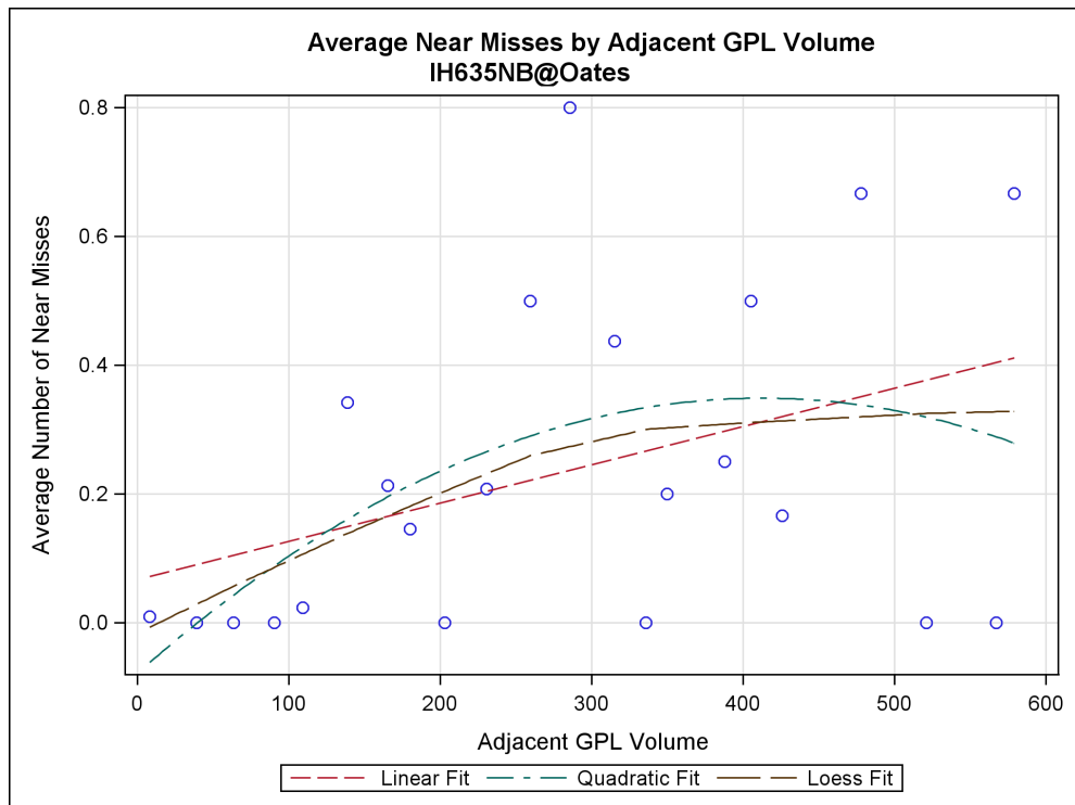
Figure H-3. Regression Trend between Near Misses vs. Adjacent GPL Volume for IH 635 NB HOV Entrance at Oates.
