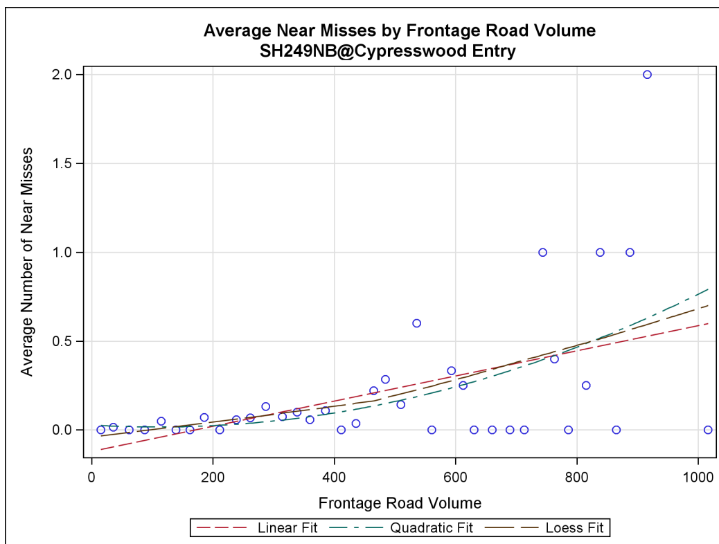
Figure H-24. Regression Trend between Near Misses vs. Frontage Volume for SH 249 NB Cypresswood Entrance Ramp.
