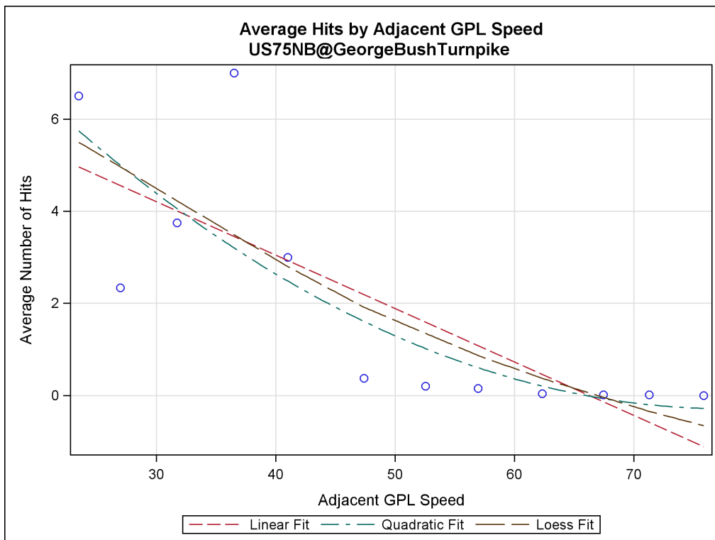
Figure H-20. Regression Trend between Hits vs. Adjacent GPL Speed for US 75 NB HOV Tangent at George Bush Turnpike.
