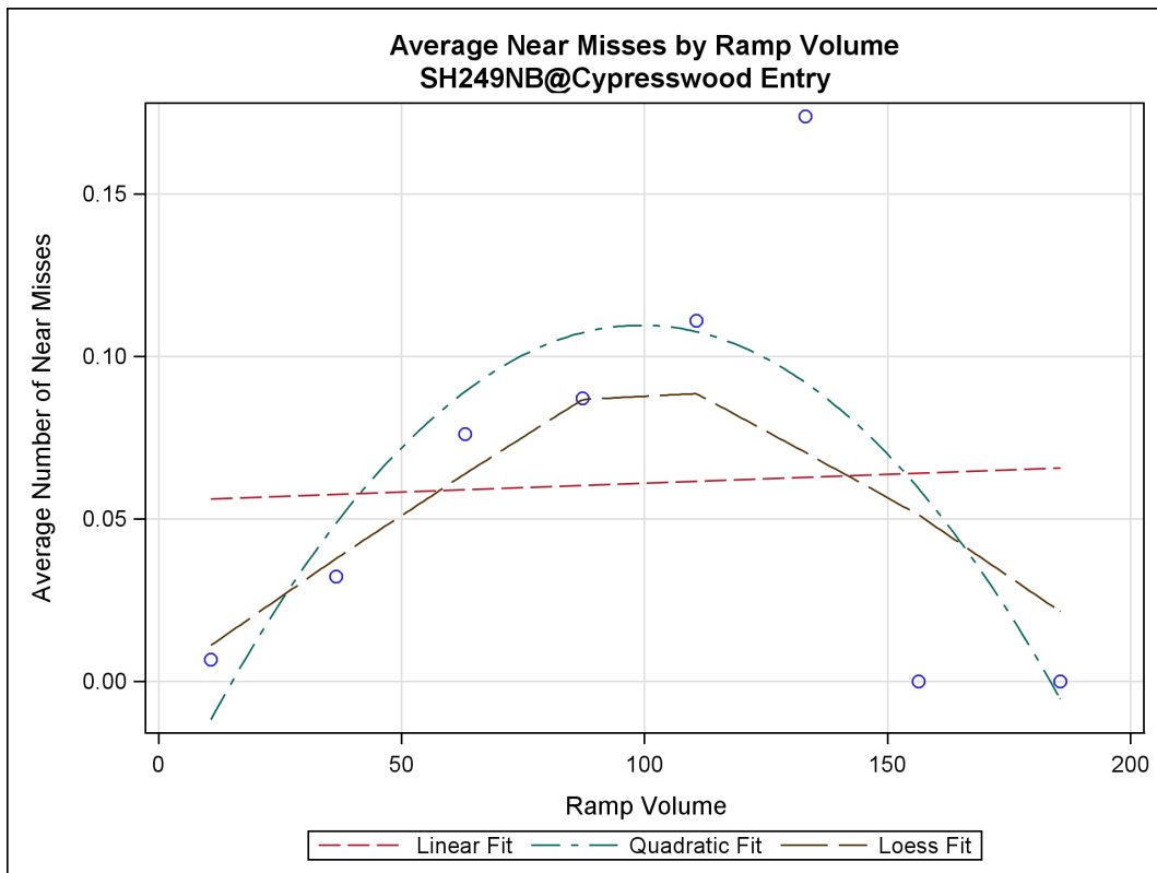
Figure H-23. Regression Trend between Near Misses vs. Ramp Volume for SH 249 NB Cypresswood Entrance Ramp.
