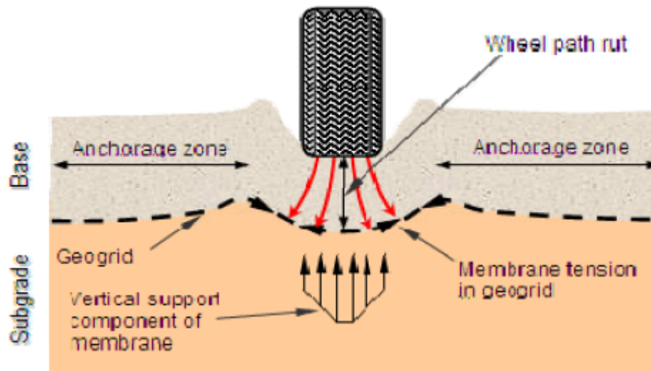
Figure 2.10. Tensioned membrane effect (Maubeuge and Klompmaker 2011).
