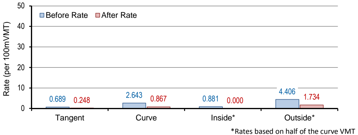
Figure 5.19 CLRS&SRS: ROTRR Rates by Horizontal Alignment – Fatal & Serious Injury
