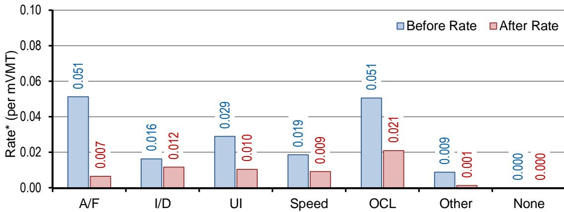
Figure 8.1 Composite: Crossover Rates by Contributing Category – All Injury Severities
