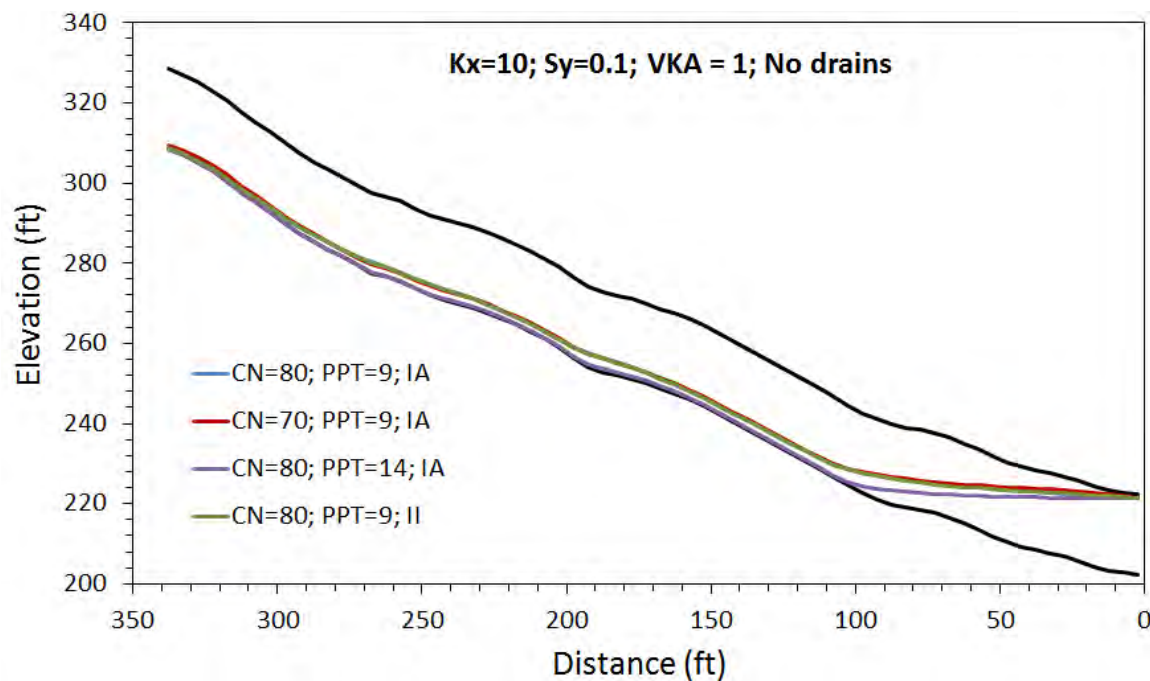
Figure 7.52: Sensitivity of water table elevations to recharge parameters for cross section d-d' given isotropic well sorted sands or gravels of higher storage. PPT = total precipitation (inches) during 24-hour event.
