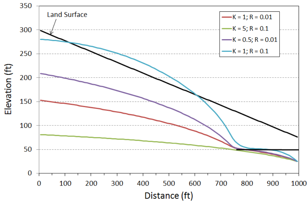
Figure 7.6: Water table profiles as a function of hydraulic conductivity (K) and recharge rate (R). Units are in feet per day. Drain length is 250 ft at an elevation of 50 ft. Drain is shown as a thick black line originating at the toe of slope.
