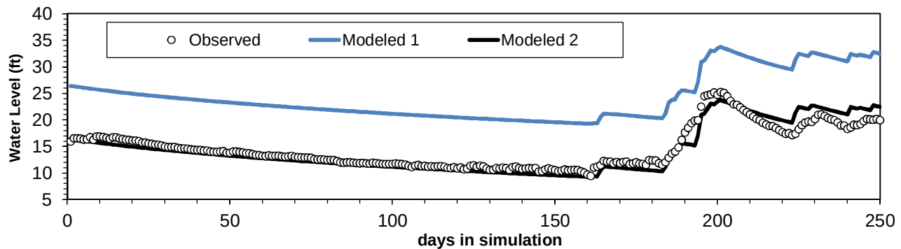
Figure 6.10: An example of transient water levels in an observation well and model results. Model 1 initial conditions are too high. Model 2, initial conditions are more realistic.
