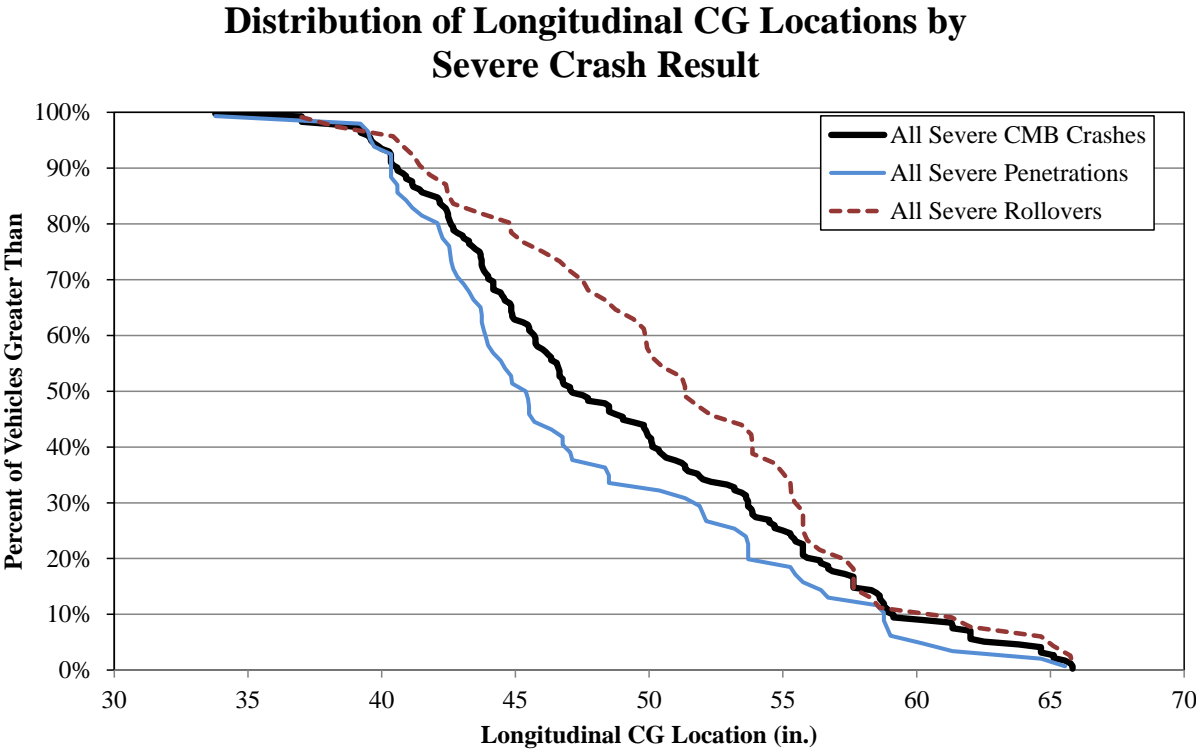
Figure 14. Distribution of Longitudinal CG Location in Severe CMB Impacts by Crash Result
