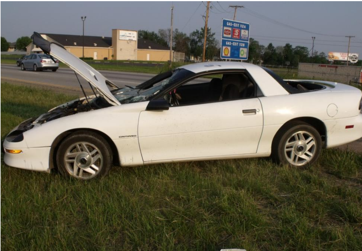
Figure 51. Prying Penetration Failure on Nucor NU-CABLE Barrier
