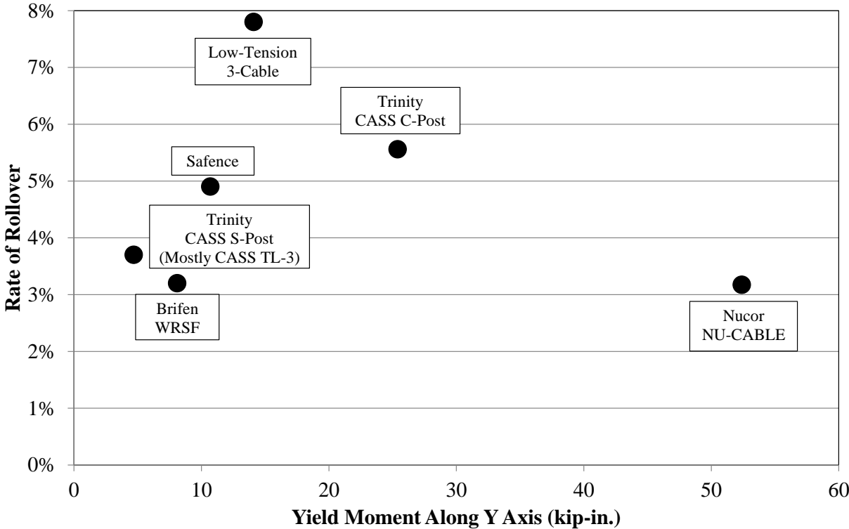
Figure 79. Y-Axis (Typ. Weak Axis) Yield Moment Relationship with Rollover Frequency
