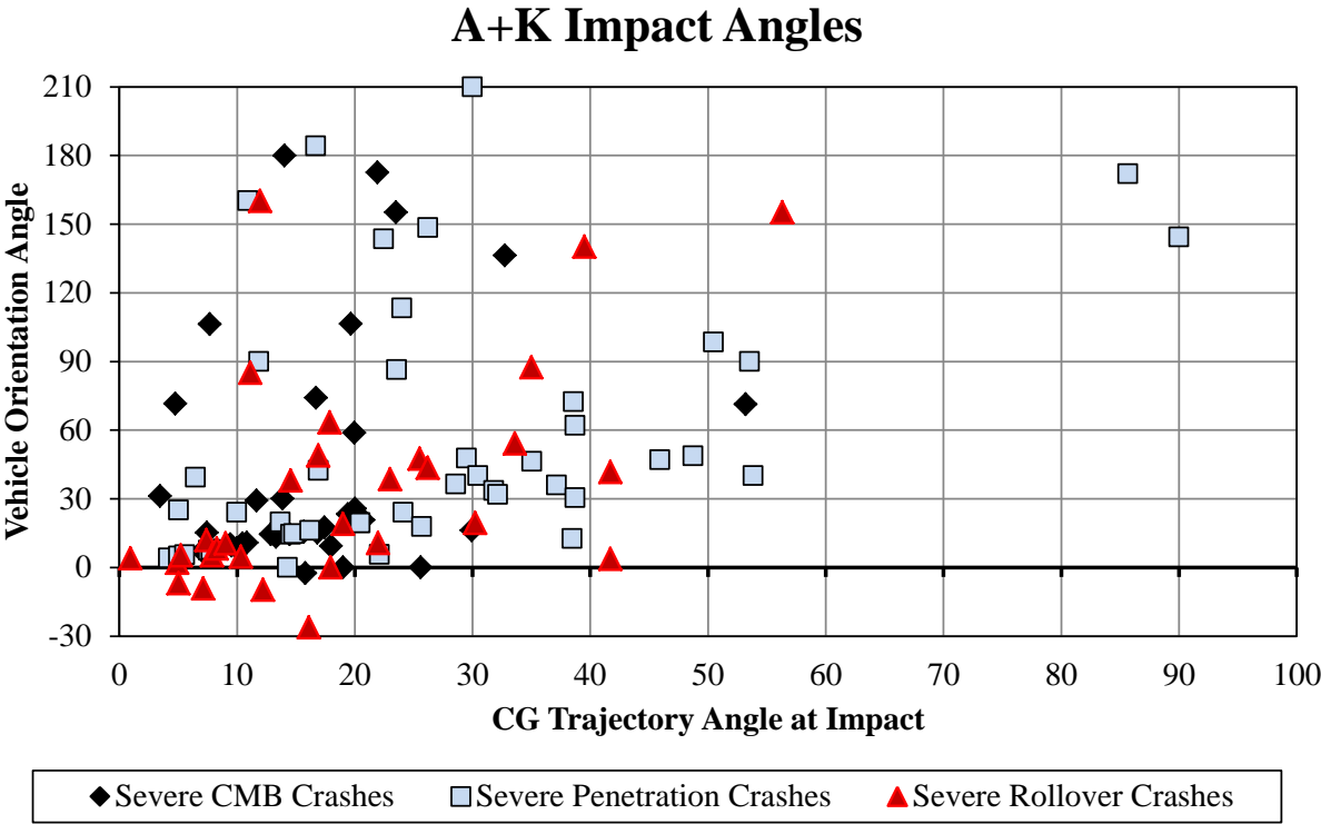
Figure 21. CG Trajectory and Orientation Angles by Crash Result
