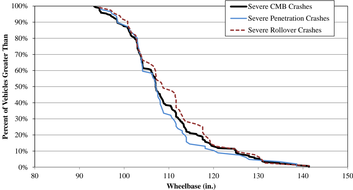
Figure 12. Distribution of Vehicle Wheelbase in Severe CMB Impacts by Crash Result
