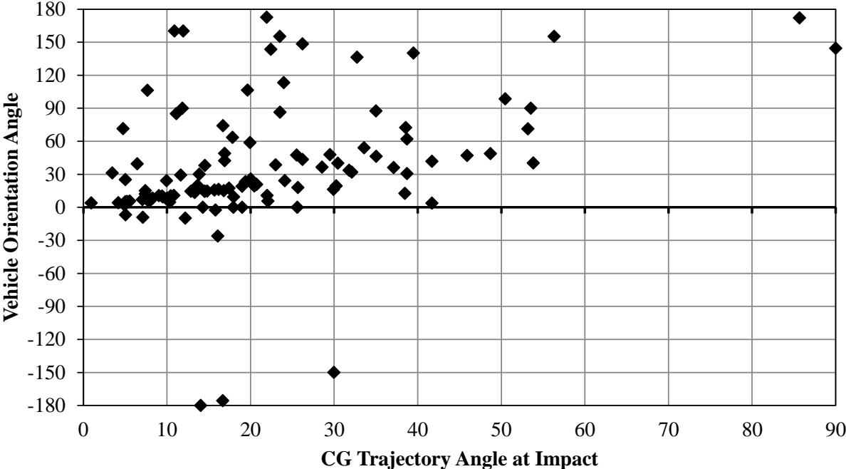
Figure 18. CG Trajectory and Orientation Angles in Severe Cable Median Barrier Crashes
