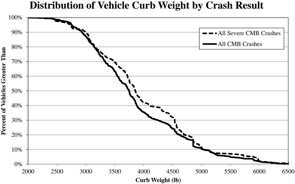
Figure 16. Distribution of Curb Weight in CMB Impacts, All Crashes
