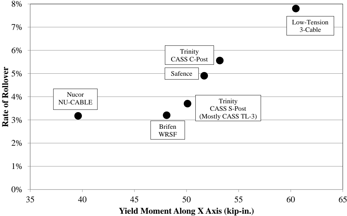
Figure 80. X-Axis (Typ. Strong Axis) Yield Moment Relationship with Rollover Frequency
