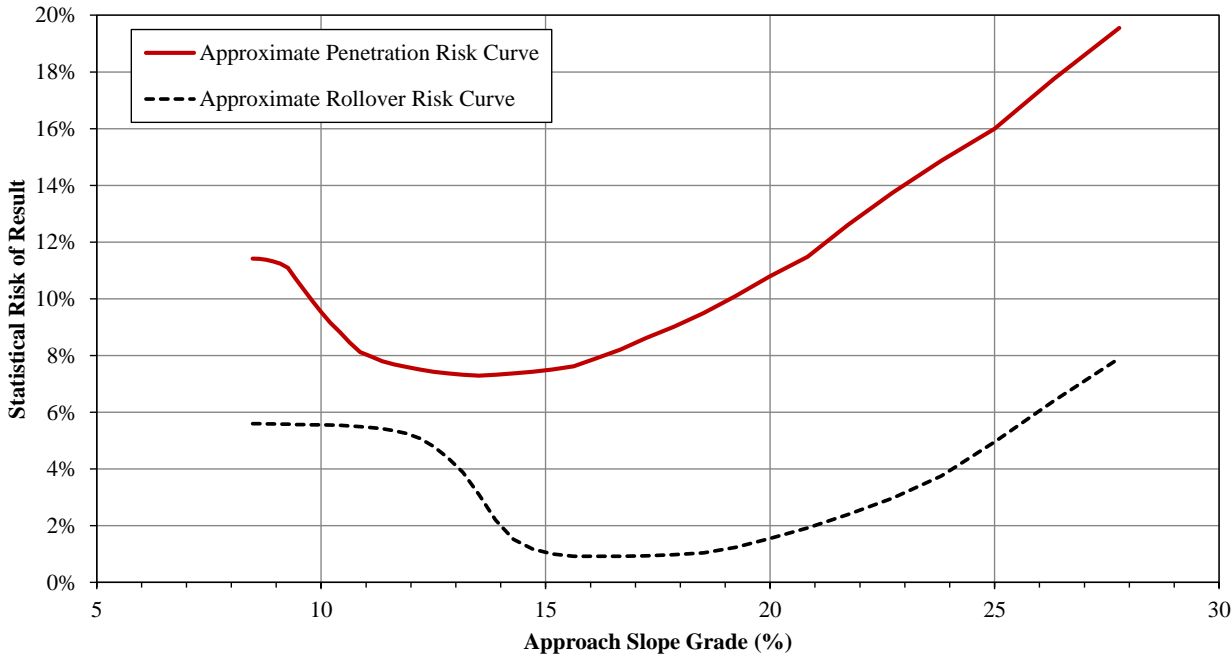
Figure 5. Estimated Median Approach Slope Risk Curves by Approach Slope Grade
