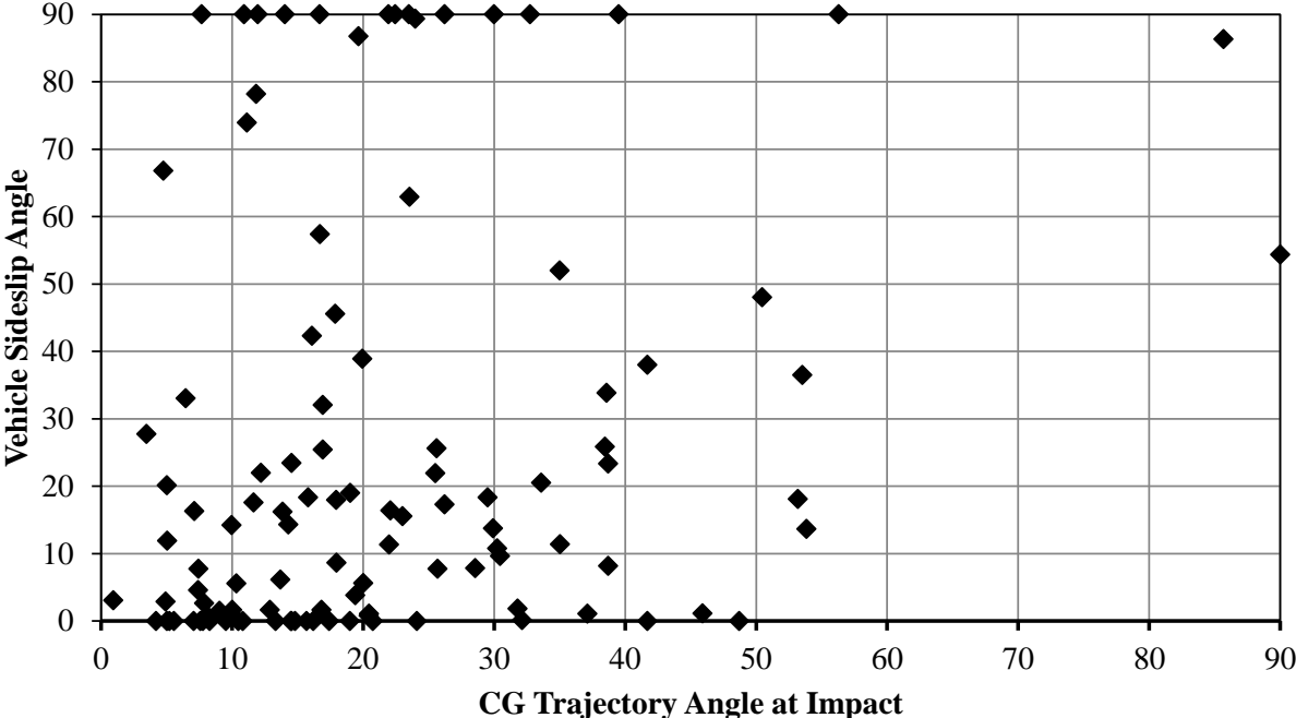
Figure 19. CG Trajectory and Sidelip Angles in Severe Cable Median Barrier Crashes
