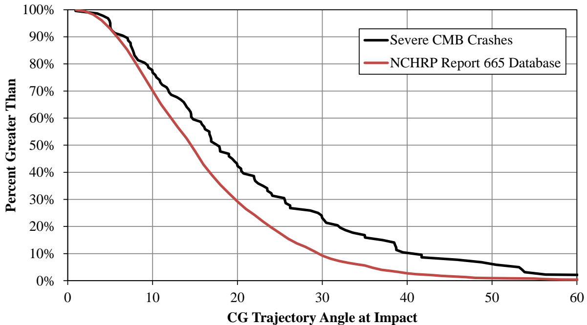
Figure 20. Comparison of Trajectory Angle Distributions
