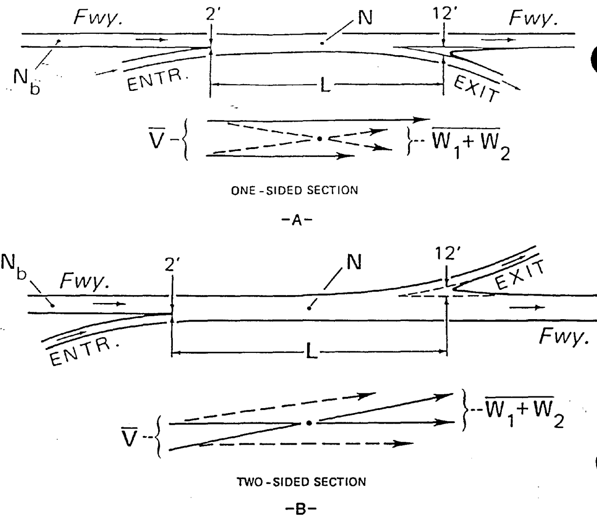
Figure 2. NOMENCLATURE OF ONE-SIDED AND TWO-SIDED WEAVING SECTIONS
