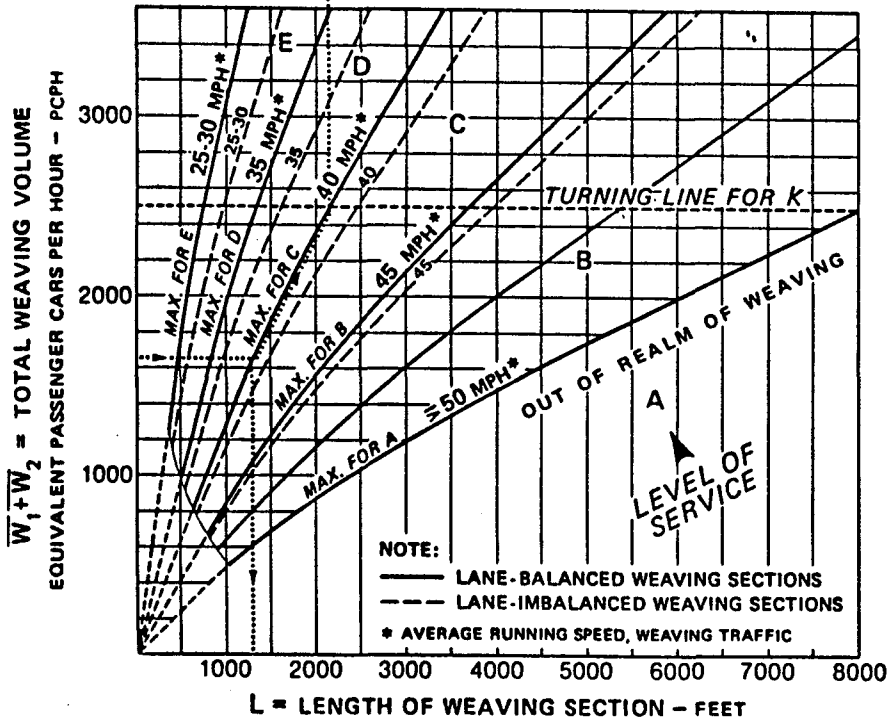
NOMOGRAPH FOR DESIGN AND ANALYSIS OF WEAVING SECTIONS - ONE-SIDED CONFIGURATIONS
