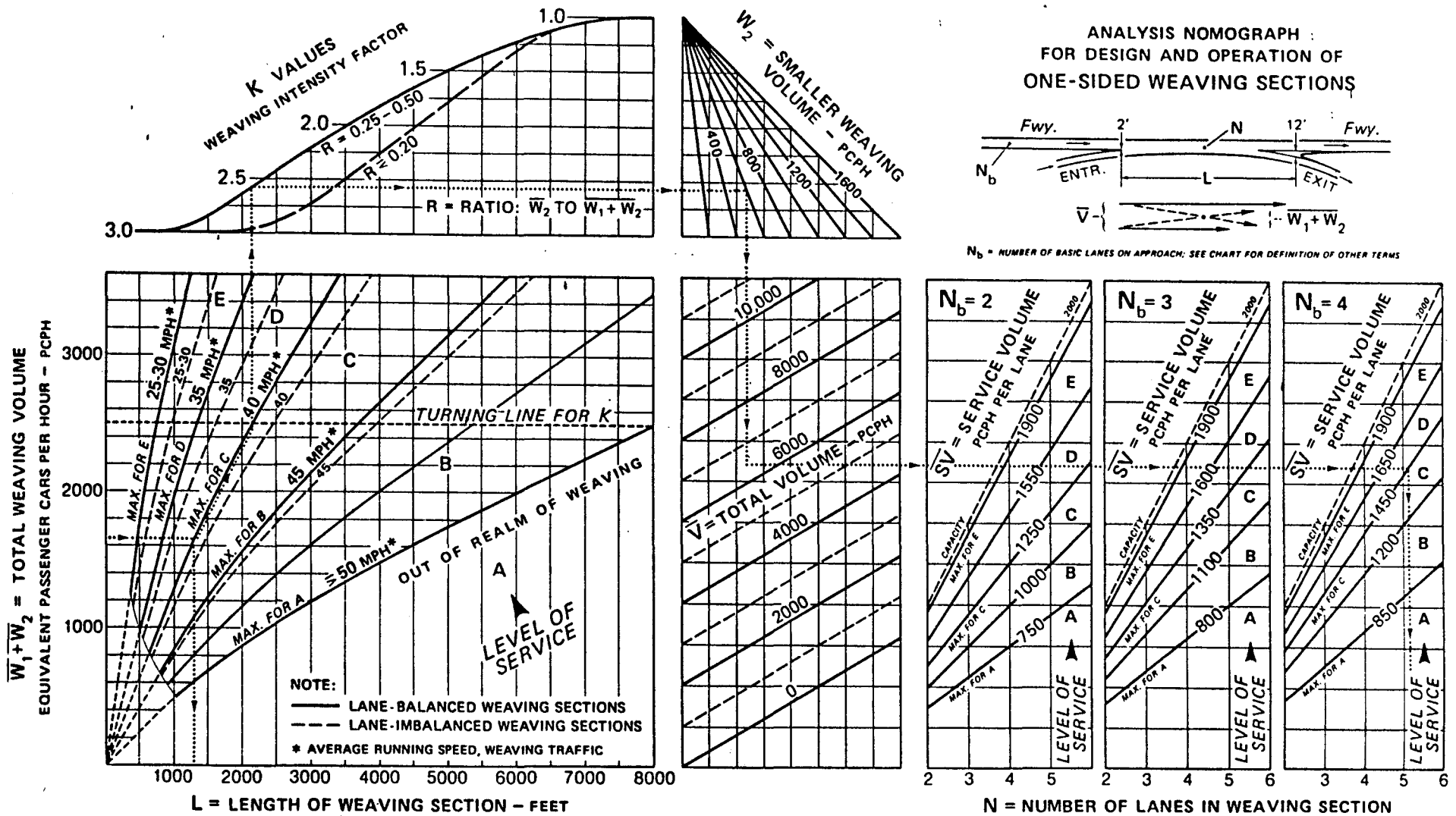
Figure 5. NOMOGRAPH FOR DESIGN AND ANALYSIS OF WEAVING SECTIONS — ONE-SIDED CONFIGURATIONS
