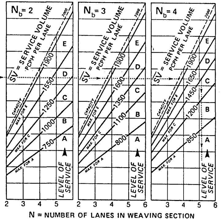
NOMOGRAPH FOR DESIGN AND ANALYSIS OF WEAVING SECTIONS - ONE-SIDED CONFIGURATIONS
