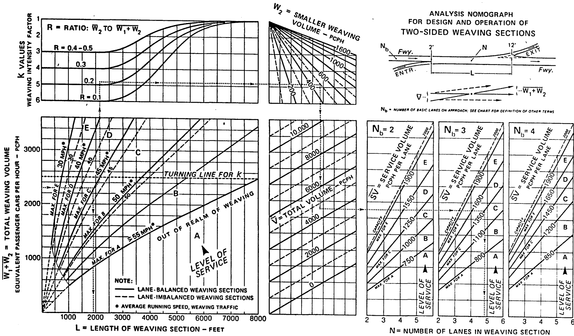
Figure 6. NOMOGRAPH FOR DESIGN AND ANALYSIS OF WEAVING SECTIONS - TWO-SIDED CONFIGURATIONS
