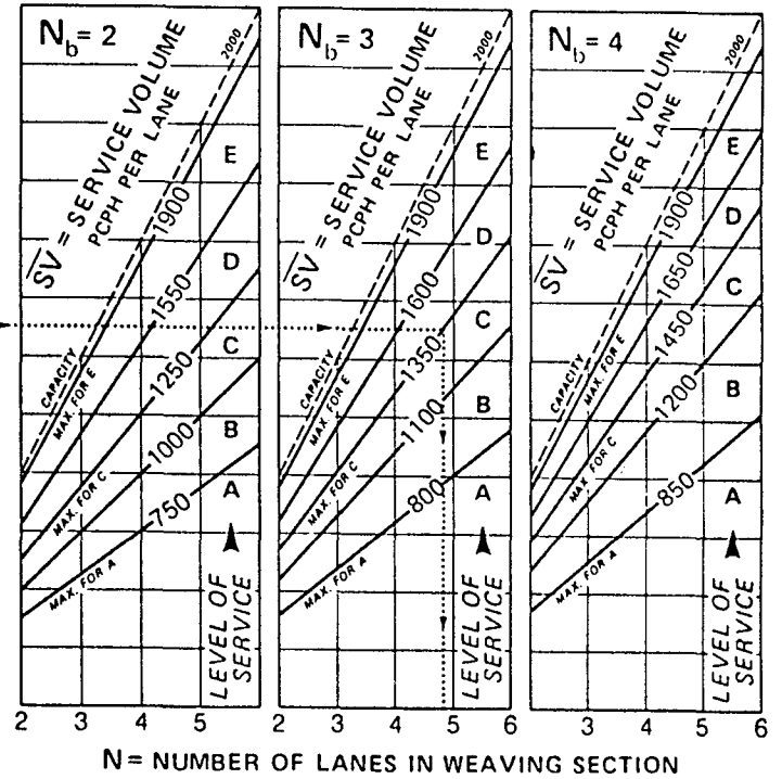
NOMOGRAPH FOR DESIGN AND ANALYSIS OF WEAVING SECTIONS - TWO-SIDED CONFIGURATIONS
