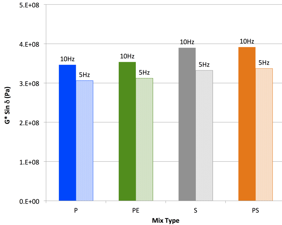
Figure 4.3. Fatigue parameter ( G^* \sin \delta ) for the four different mixes
