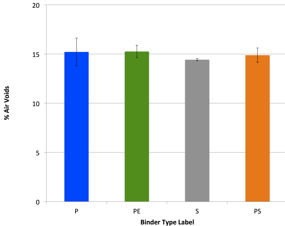
Figure 3.7. Average and standard deviation of air voids in the six specimens for each one of the four binder types
