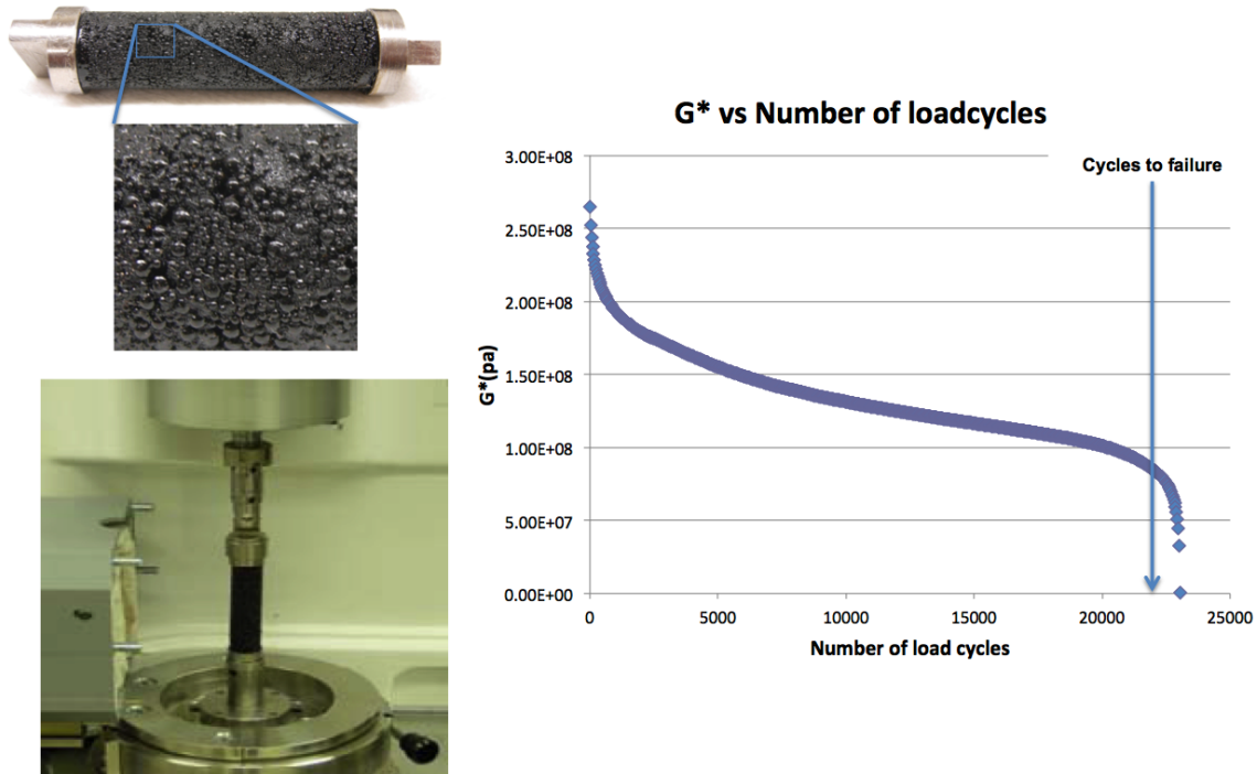
Figure 2.7. Mortar specimen with glass bead (top left) used in a DSR (bottom left), and typical loss in G^* or damage as a function of number of load cycles (right); the test can also be conducted by applying a constant rate of shear deformation to obtain stress-strain failure curve
