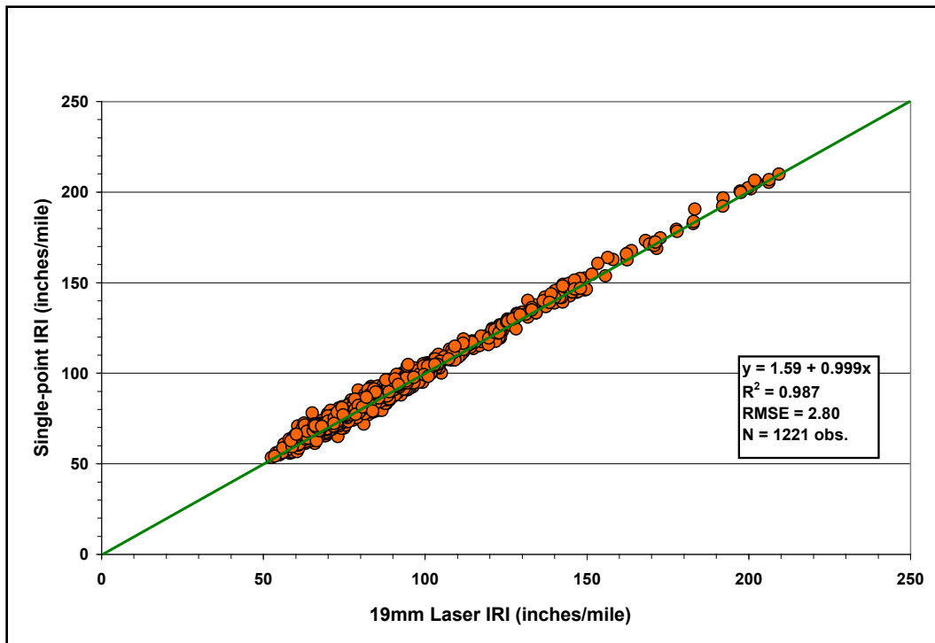
Figure A17. Comparison of Single-Point and 19mm Laser IRIs on SH21, US77, and US290 Grade 4 Sections.
