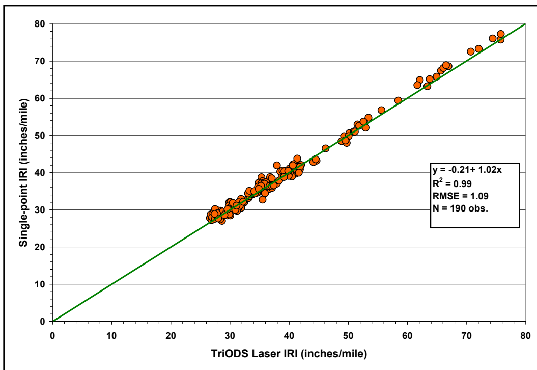
Figure A38. Comparison of Single-Point and TriODS Laser IRIs on US59 Type D Project.
