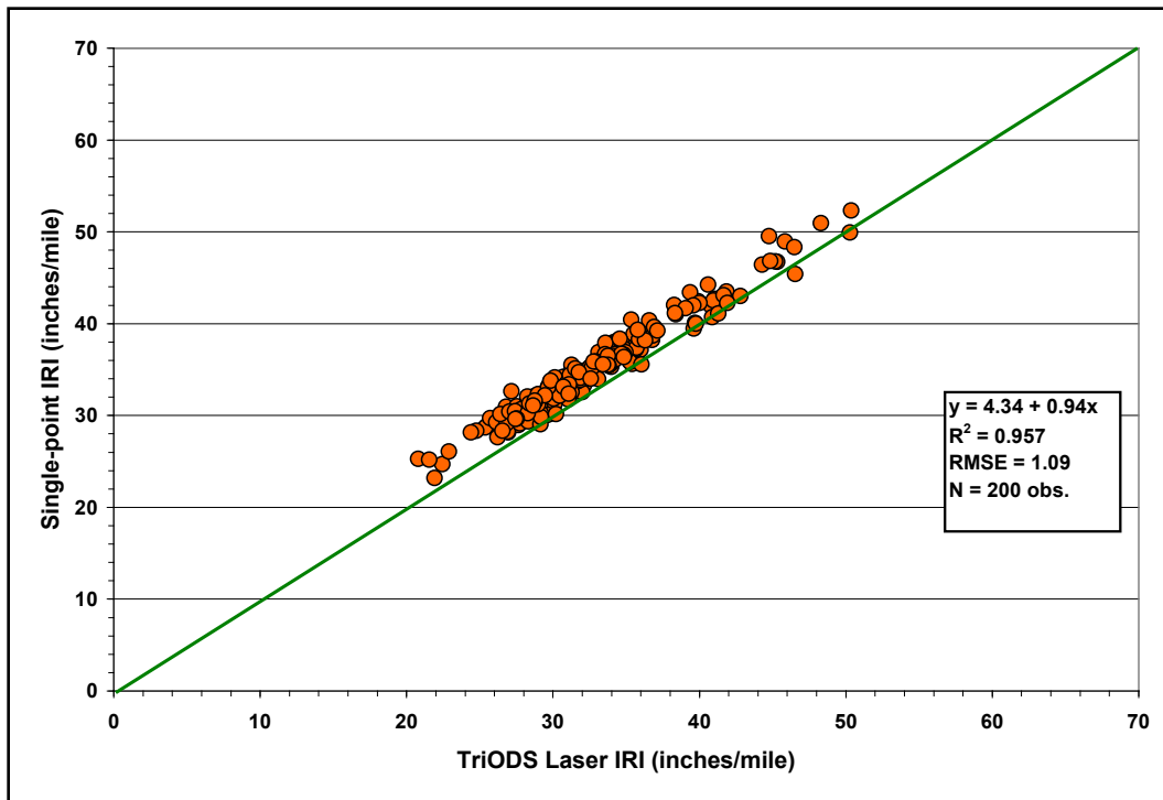
Figure A39. Comparison of Single-Point and TriODS Laser IRIs on US77 Type D Project.
