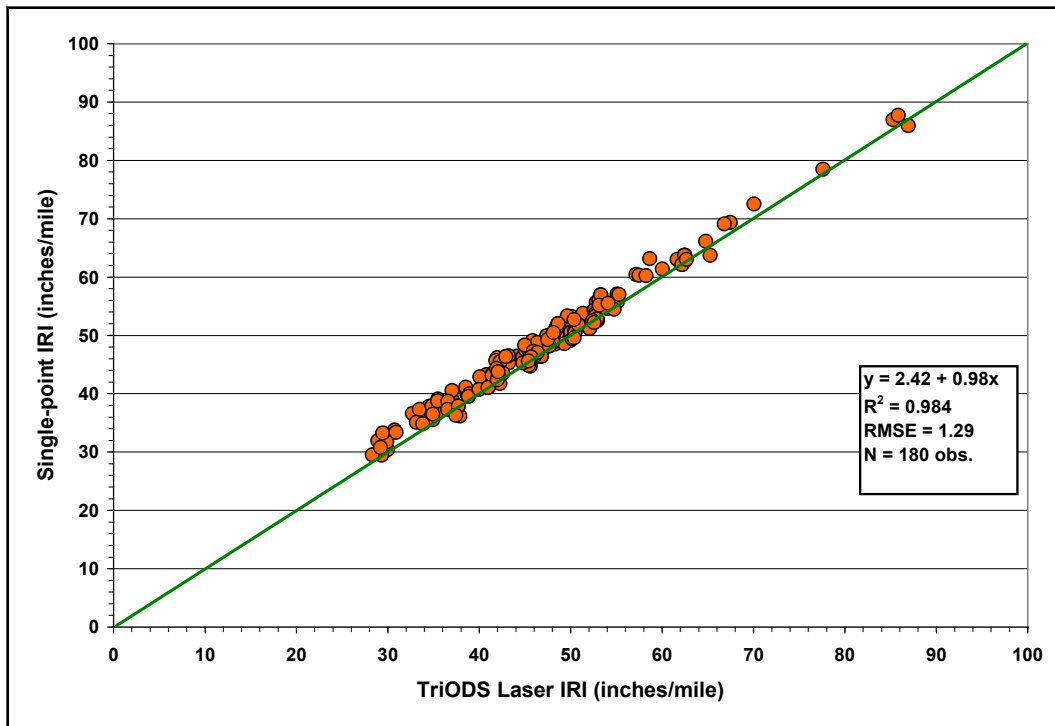
Figure A37. Comparison of Single-Point and TriODS Laser IRIs on Loop 463 Type C Project.
