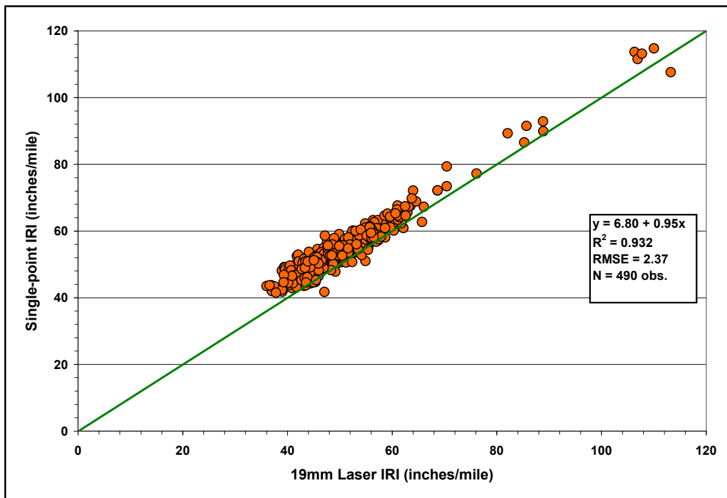
Figure A16. Comparison of Single-Point and 19mm Laser IRIs on SH6 PFC Project.
