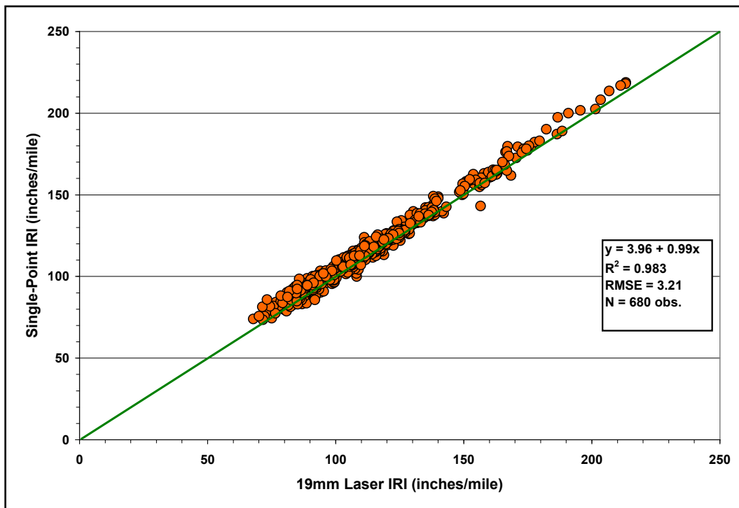
Figure A18. Comparison of Single-Point and 19mm Laser IRIs on US90A, and FM50 Grade 3 Sections.
