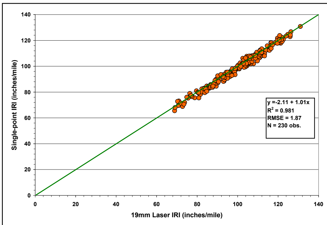
Figure A26. Comparison of Single-Point and 19mm Laser IRIs on US287 CRCP Skidabrader Section.
