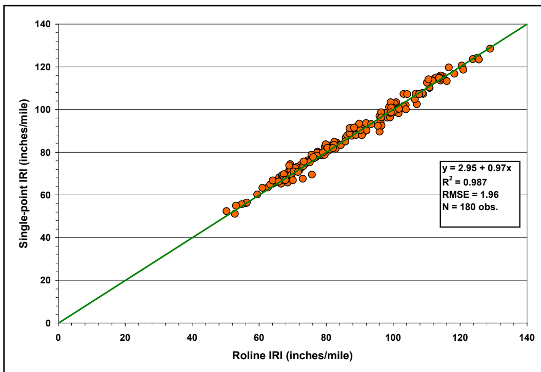
Figure A12. Comparison of Single-Point and Roline Laser IRIs on US287 CRCP Section with Deep Transverse Tines.
