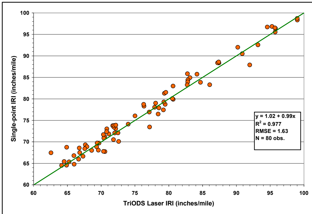
Figure A35. Comparison of Single-Point and TriODS Laser IRIs on FM734 SMA-D Project.
