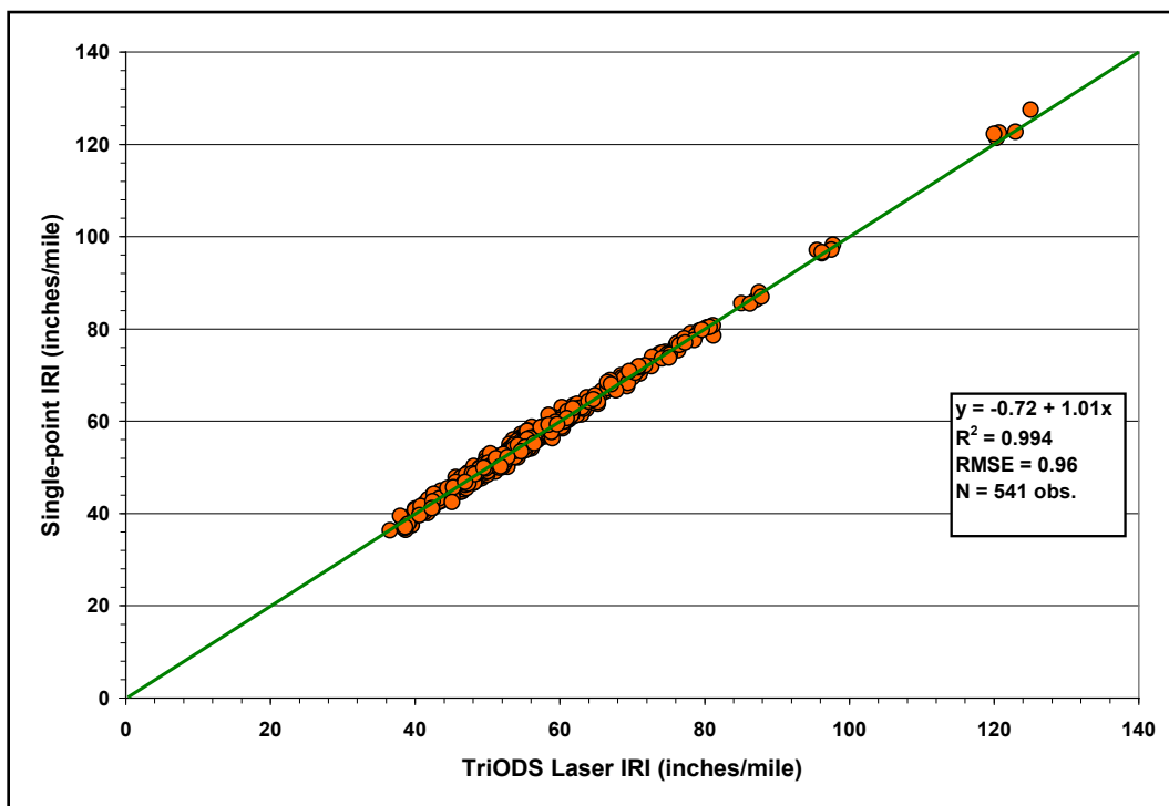
Figure A36. Comparison of Single-Point and TriODS Laser IRIs on FM2440 Type C Project.
