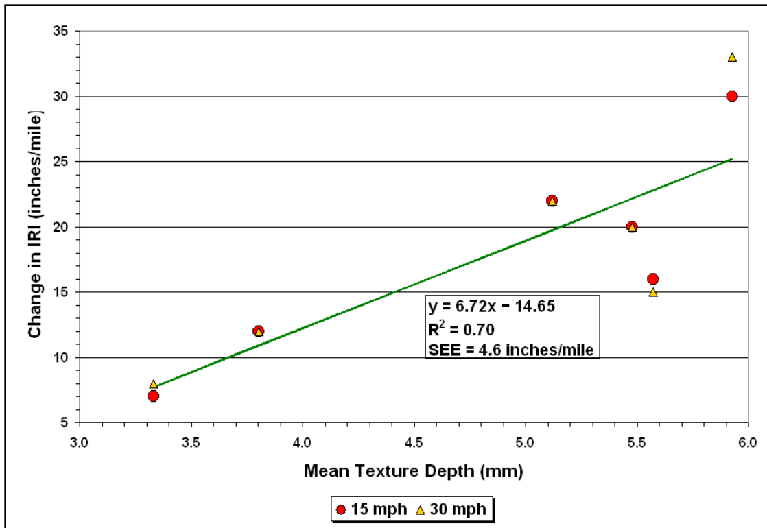
Figure 2.2. Relationship between IRI and Texture from Laboratory Tests (Fernando, Walker, Estakhri, 2008).
