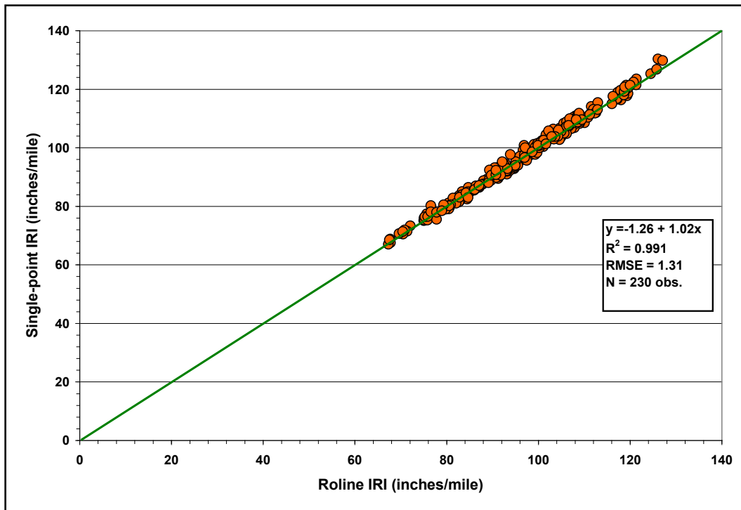
Figure A11. Comparison of Single-Point and Roline Laser IRIs on US287 CRCP Skidabrader Section.
