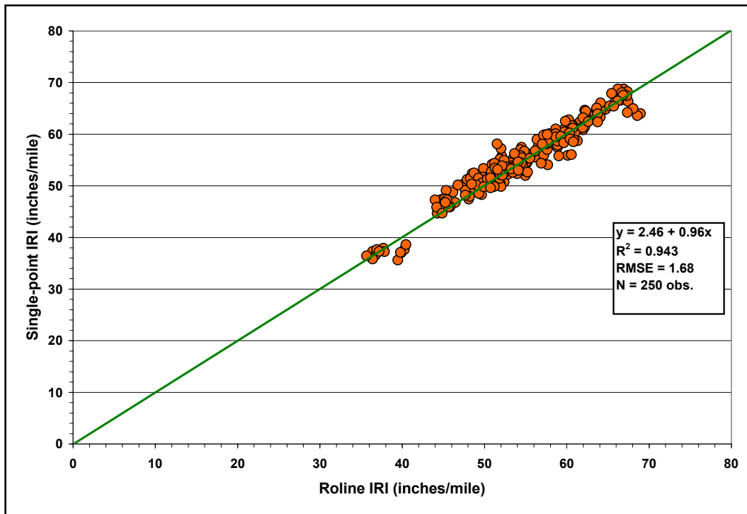
Figure A13. Comparison of Single-Point and Roline Laser IRIs on SH6 and SH36 CRCP Sections with Conventional Transverse Tines.
