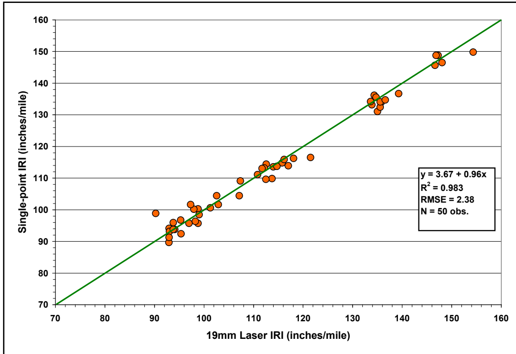
Figure A29. Comparison of Single-Point and 19mm Laser IRIs on IH35 and SH36 CRCP Sections with Carpet Dragged Surface.
