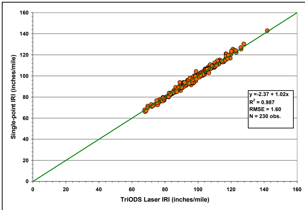
Figure A41. Comparison of Single-Point and TriODS Laser IRIs on US287 CRCP Skidabrader Section.
