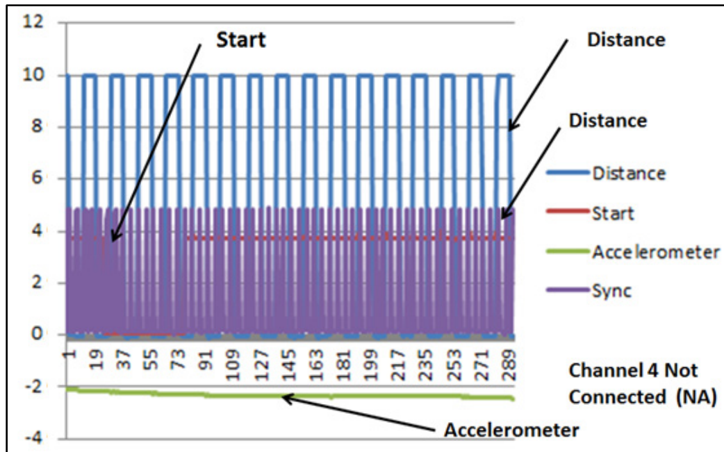
Figure 4.4. Illustration of the Analog Signals Collected by Roline Profiling System.
