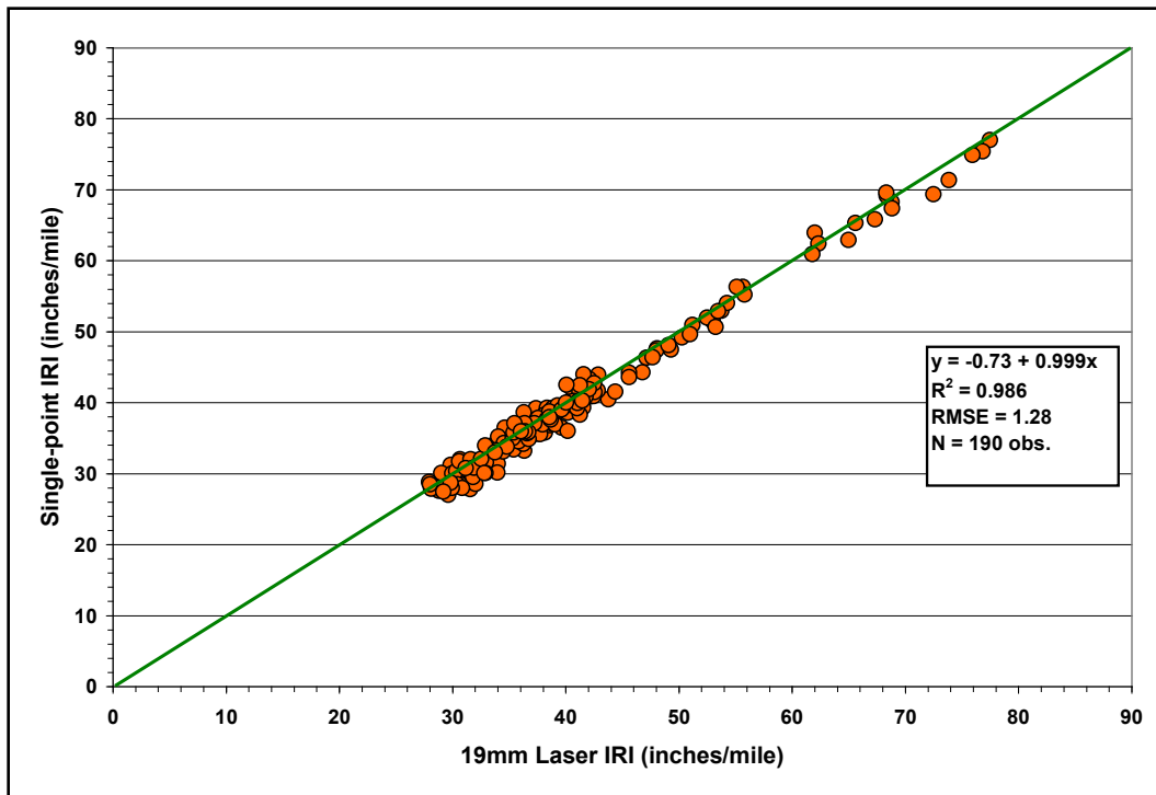
Figure A23. Comparison of Single-Point and 19mm Laser IRIs on US59 Type D Project.
