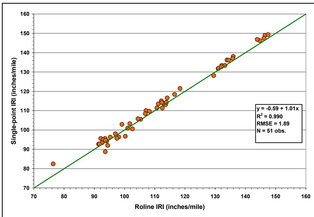
Figure A14. Comparison of Single-Point and Roline Laser IRIs on IH35 and SH36 CRCP Sections with Carpet Dragged Surface.
