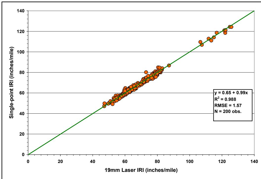
Figure A19. Comparison of Single-Point and 19mm Laser IRIs on Loop 1 SMA-C Project.
