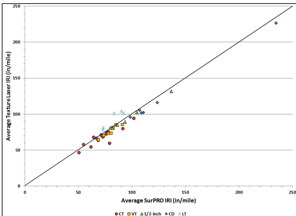
Figure 5.4. Comparison of Texture Laser and SurPRO IRIs on CRCP Sections.
