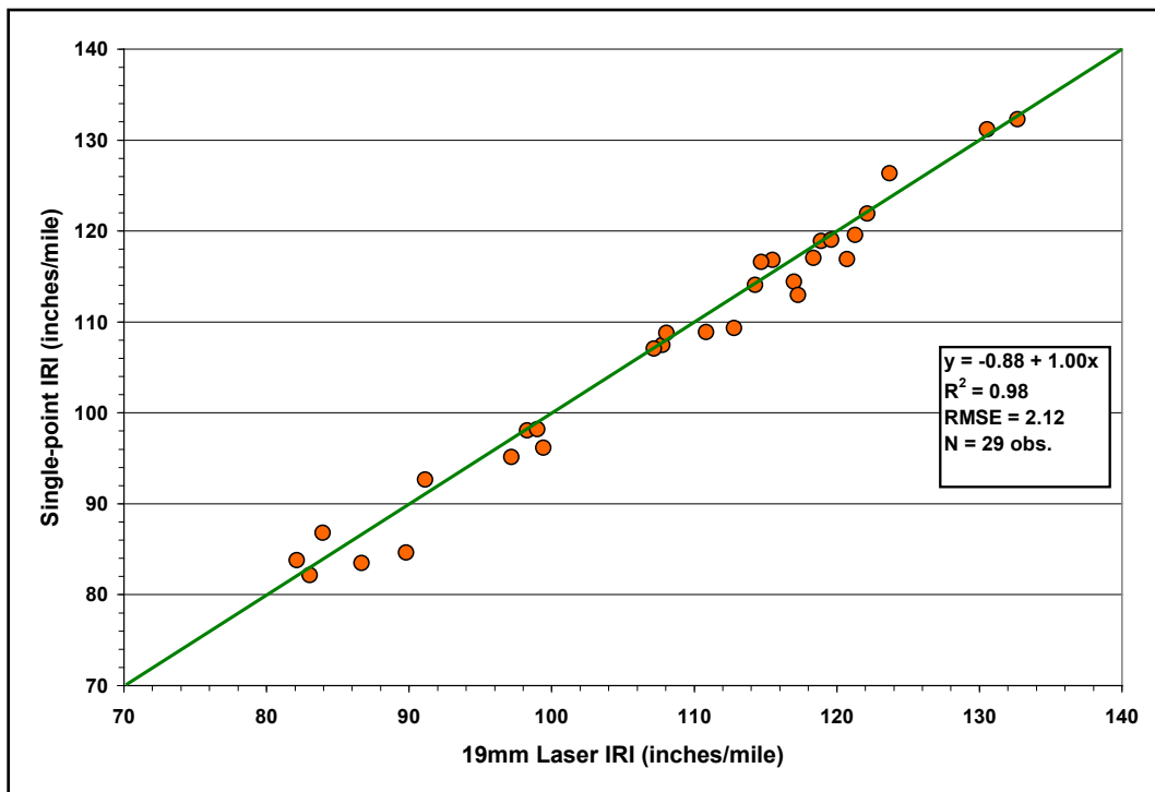
Figure A30. Comparison of Single-Point and 19mm Laser IRIs on IH35 CRCP Section with Belt Dragged Surface.
