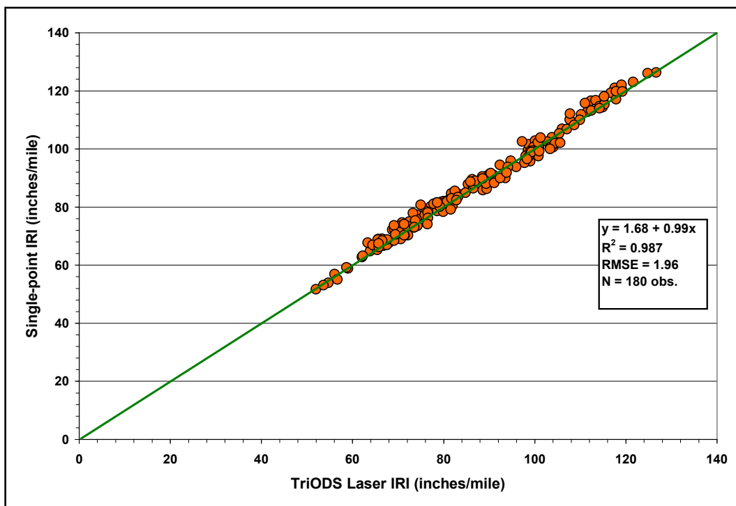
Figure A42. Comparison of Single-Point and TriODS Laser IRIs on US287 CRCP Section with Deep Transverse Tines.
