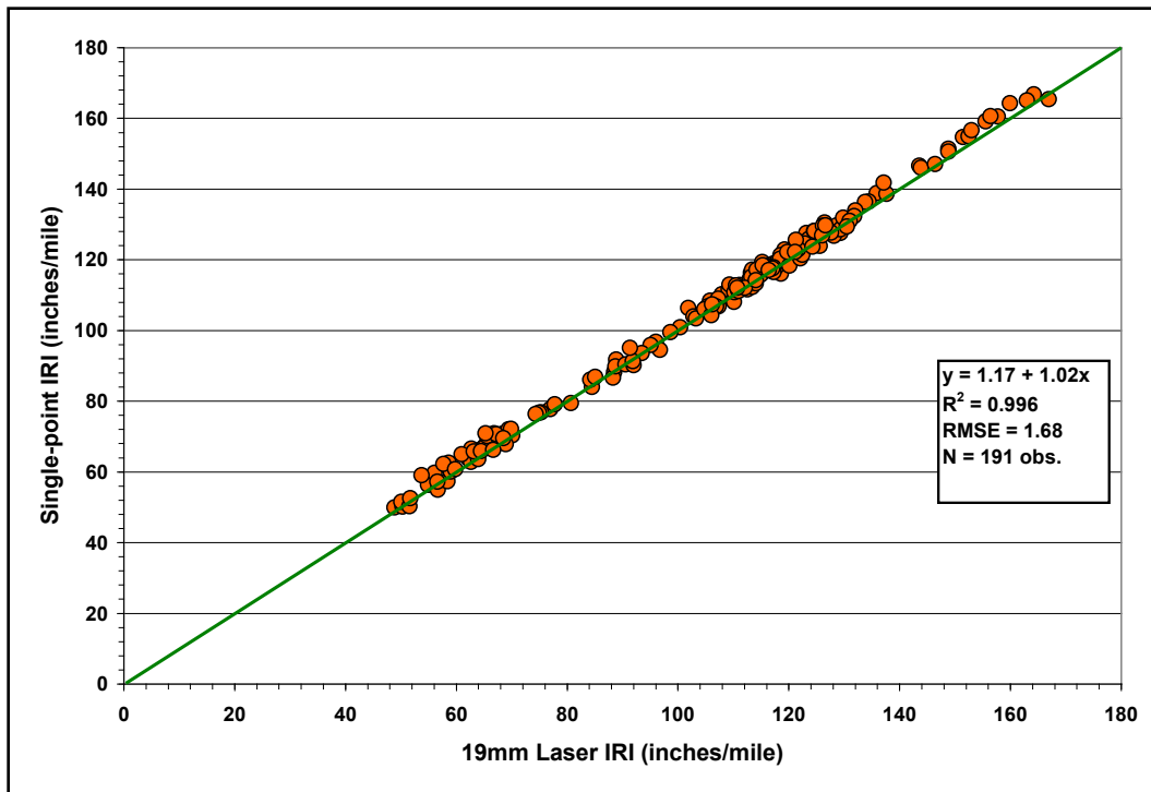
Figure A25. Comparison of Single-Point and 19mm Laser IRIs on IH820 and SH36 CRCP Sections with Variable Transverse Tines.
