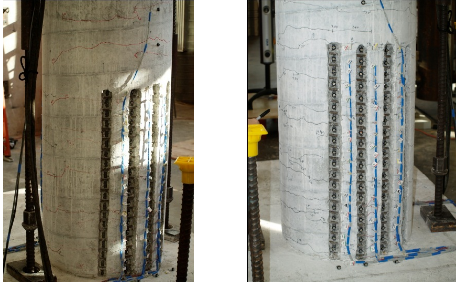
Figure 2-45. Test 8 – Crack Patterns on the (Left) South Side at ( \mu_{-1.2}^{8.12 \text{ sec}} = -1.00'' ) and (Right) North Side at ( \mu_{1.6}^{8.40 \text{ sec}} = 1.35'' )
