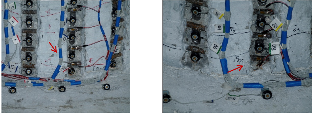
Figure 2-8. Test 9 – First Signs of Cover Concrete Flaking which Precedes Crushing (Left) South Side during ( \mu_2^{+2} = 1.69'' ) and (Right) North Side during ( \mu_2^{-2} = -1.67'' )
