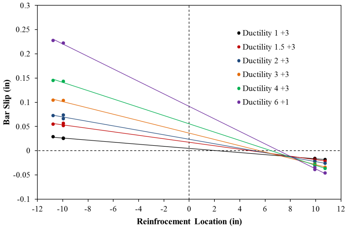
Figure 2-264. Test 15 - Base Rotation due to Strain Penetration during Push Cycles
