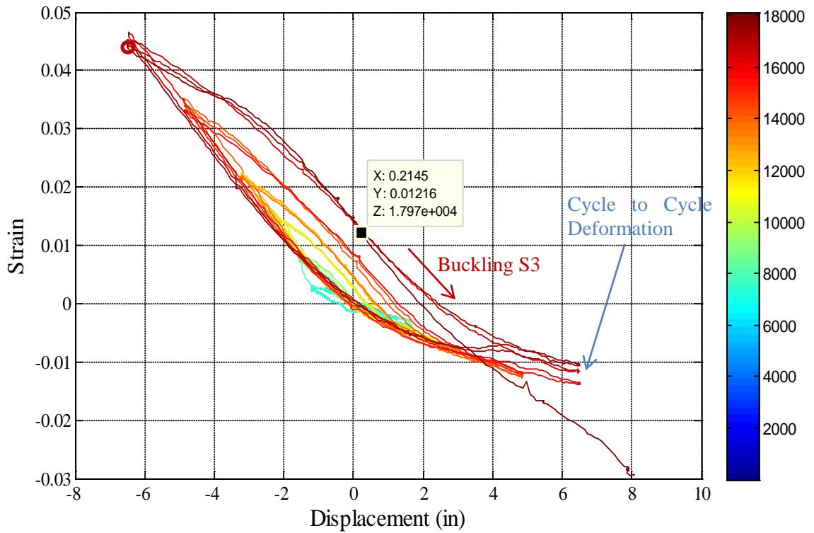
Figure 2-183. Test 13 – Bar S3 Strain Hysteresis (Buckled Region 4.41" Above the Footing)
