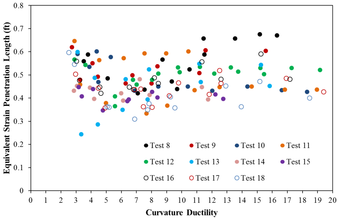
Figure 4-40. Equivalent Strain Penetration Length (Equivalent L_{sp} = \text{Fixed End Rotation} / \text{Base Curvature} )
