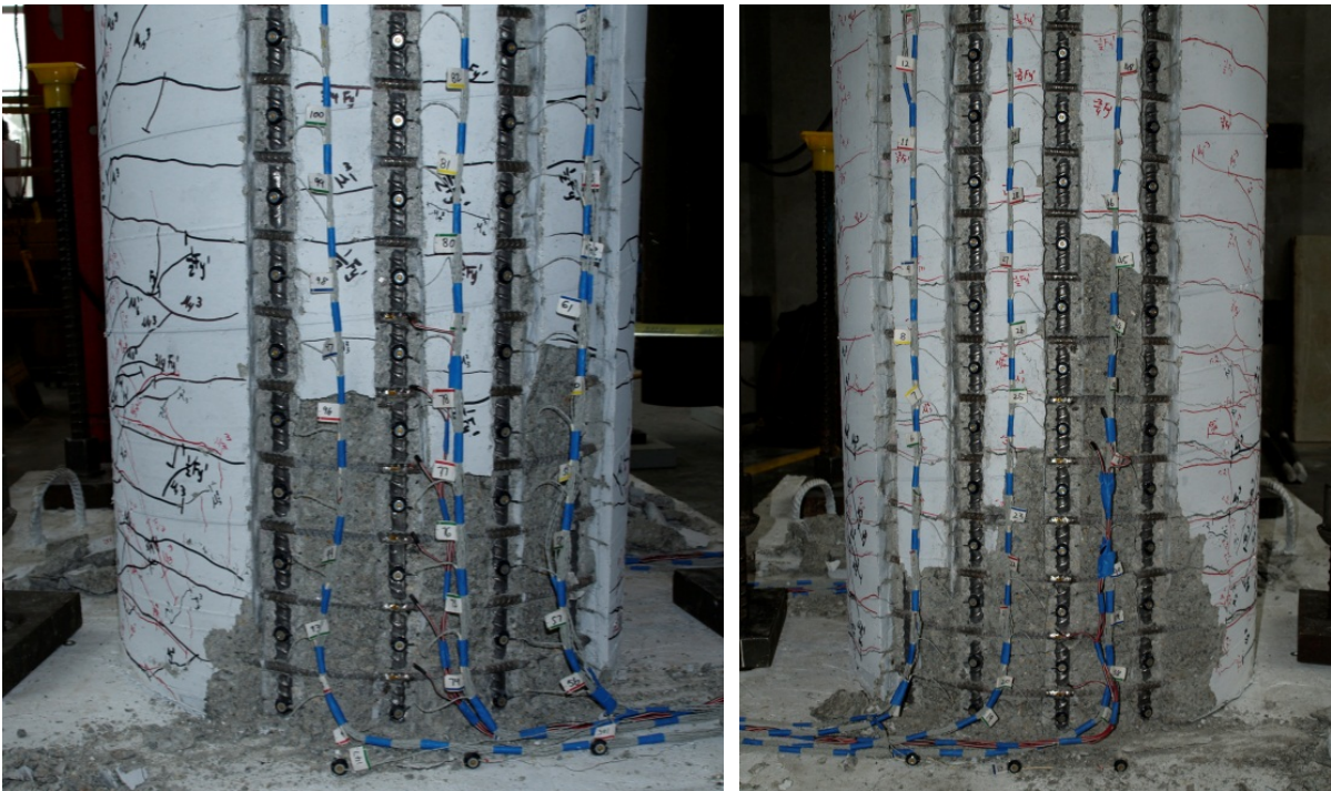
Figure 2-238. Test 15 – (Left) Extent of Crushing on the North Side of the Specimen during ( \mu_6^- = -5.00'' ) and (Right) Crushing on the South Side during ( \mu_6^+ = 5.01'' ) (Both Prior to Buckling)
