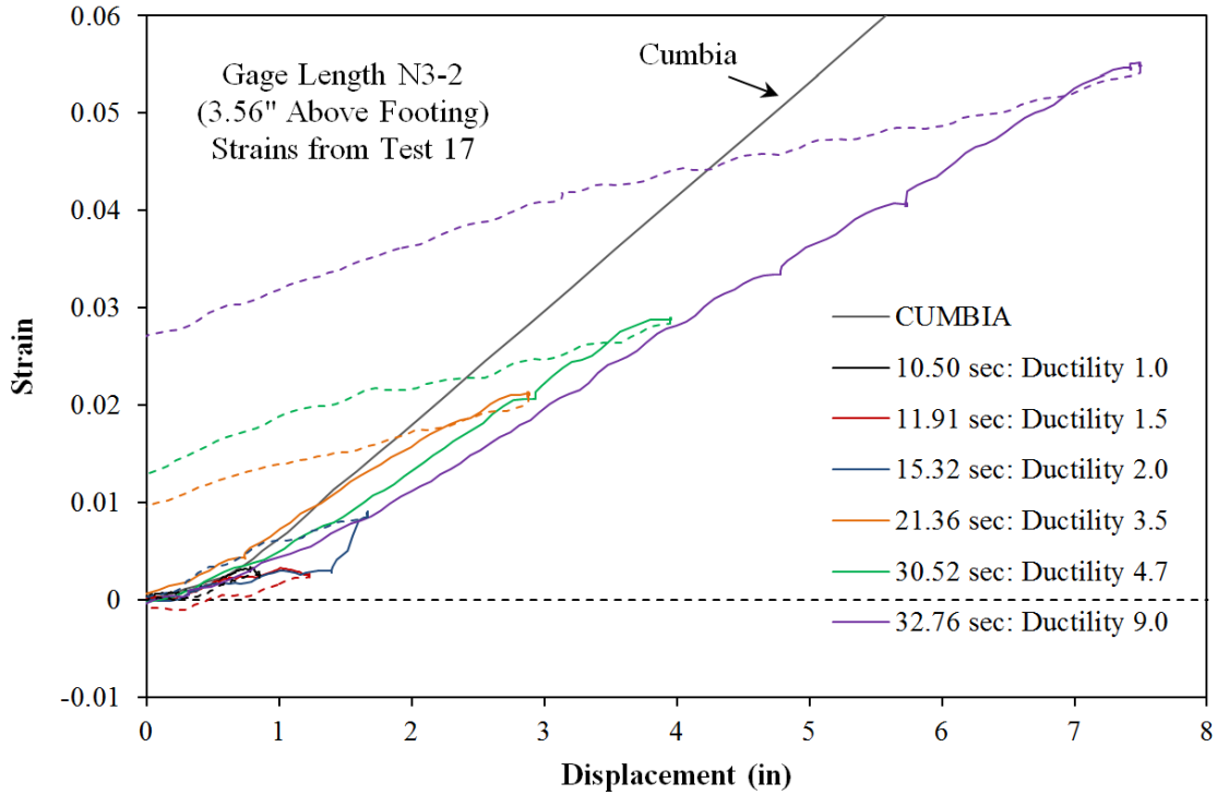
Figure 2-321. Test 17 – Tensile Strain and Disp. during Push Cycles (Bar N3, 3.56'' Above)
