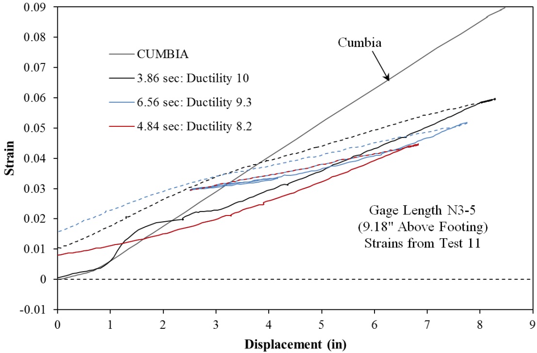
Figure 2-114. Test 11 – Transverse Steel Strains for Lowest Six Spiral Layers on the North
