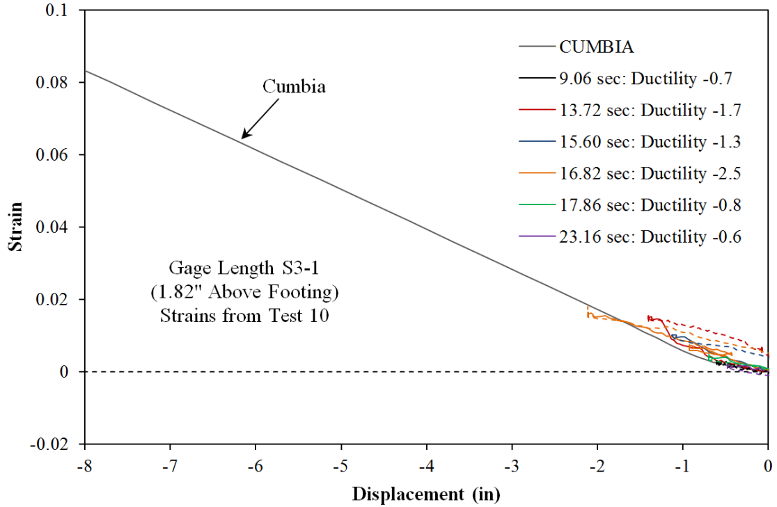
Figure 2-84. Test 10 – Strain and Displacement for Bar S3 during Pull Cycles
