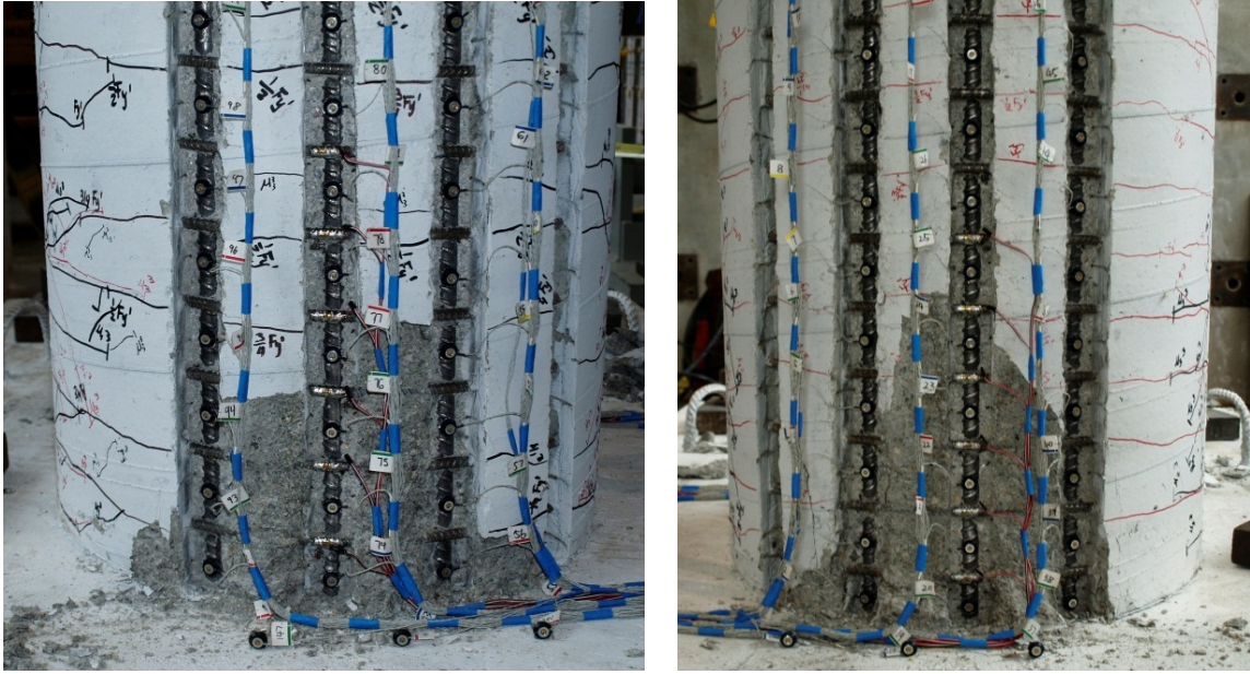
Figure 2-237. Test 15 – (Left) Crushing on the North Side of the Specimen during ( \mu_3^- = -2.51'' ) and (Left) Crushing on the South Side during ( \mu_3^+ = 2.49'' )
