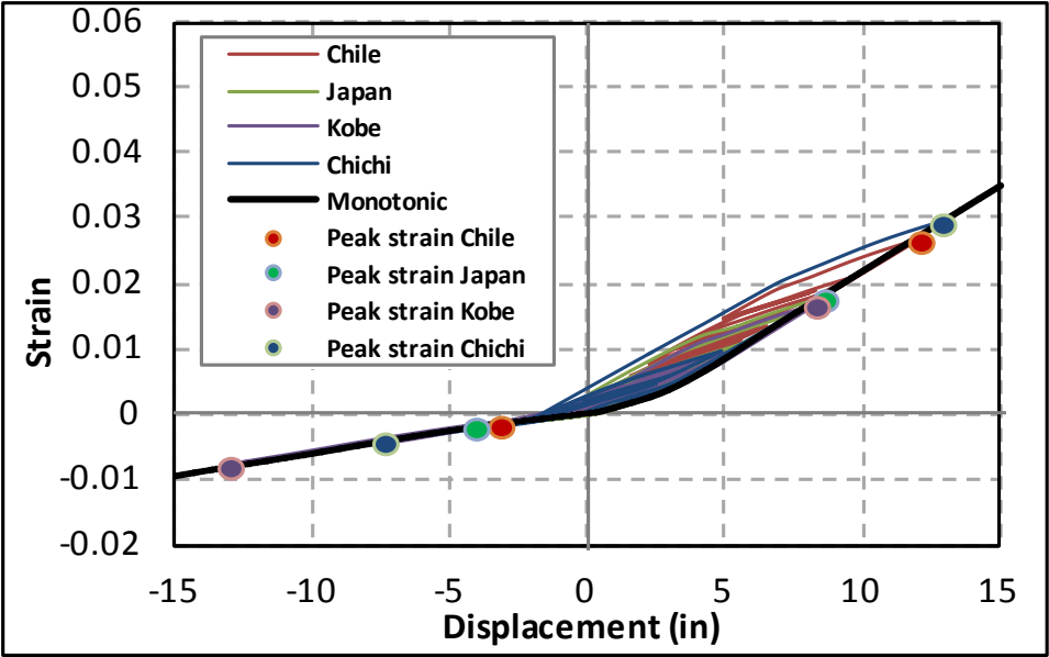
Figure 3-20. Strain Hysteretic Responses with 16 ft Column
