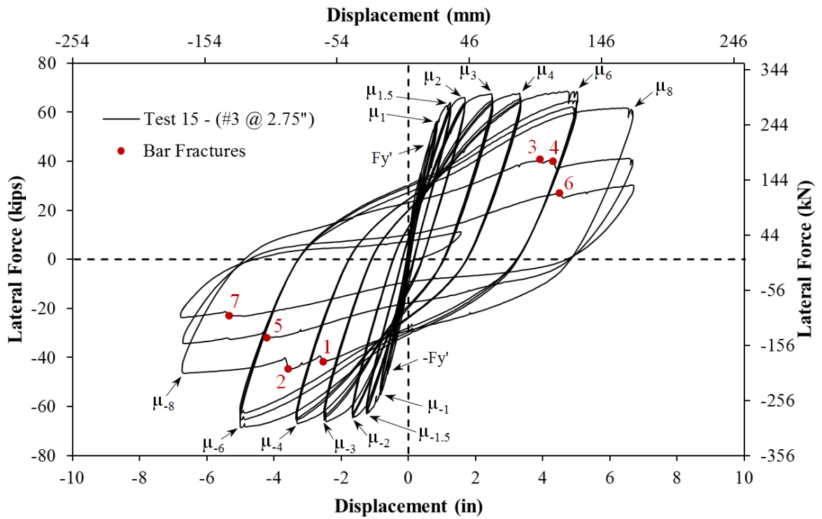
Figure 2-233. Test 15 - Rupture History of Previously Buckled Reinforcement
