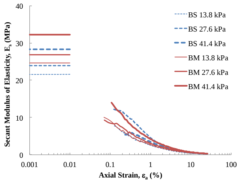
Figure 8. Variation of secant modulus of elasticity with axial strain in undrained triaxial compression – stiffness values at very small strains were determined from bender element tests
