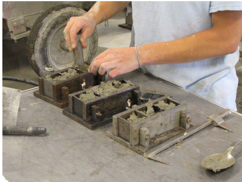
Figure 3.9 – Mortar Cubes
