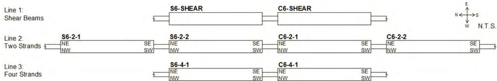
Figure 4.6 – C6 and S6 Prestressing Bed Layout
