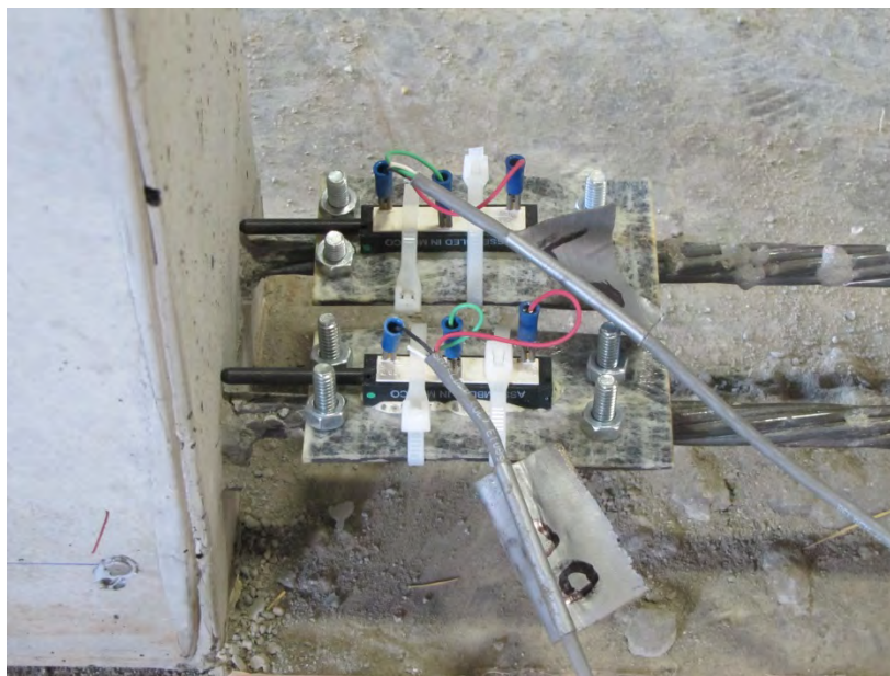
Figure 4.21 – Improved Potentiometer-FRP Assemblies with Zip Ties and Plastic Epoxy (Top) and Gorilla Glue Expanding Foam (Bottom)
