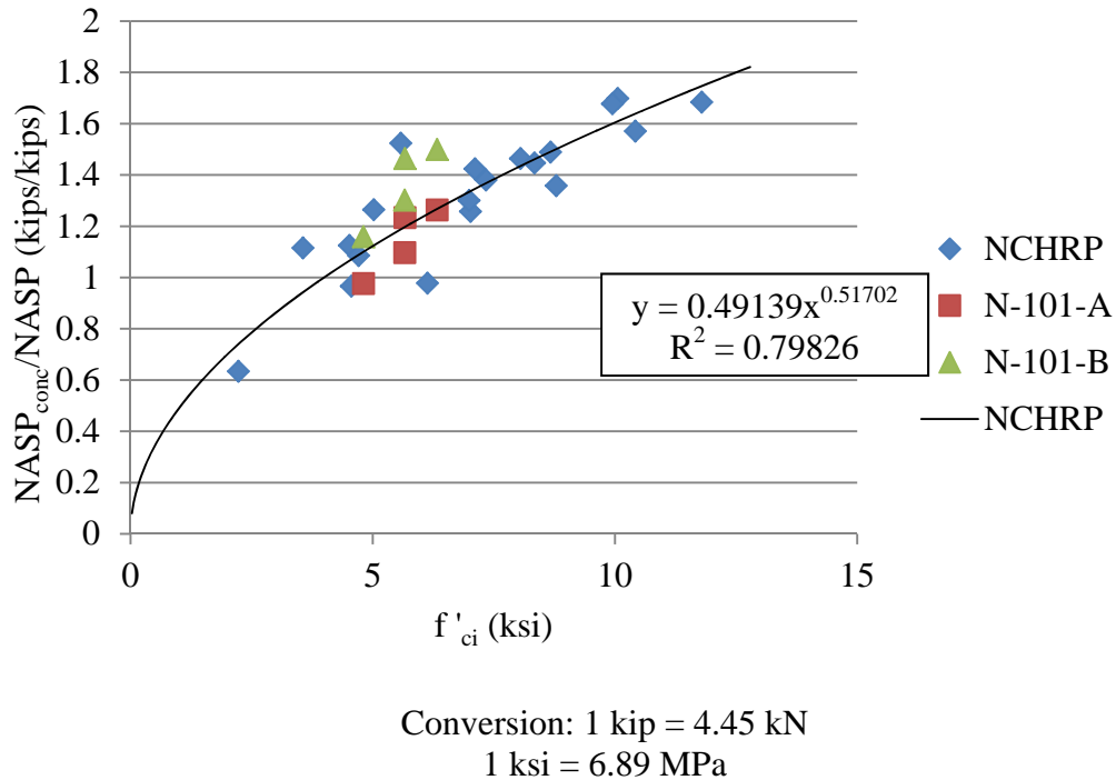
Figure 5.38 – Normalized NASP in Concrete Pullout Values vs. Concrete Strength (NCHRP and Missouri S&T)
