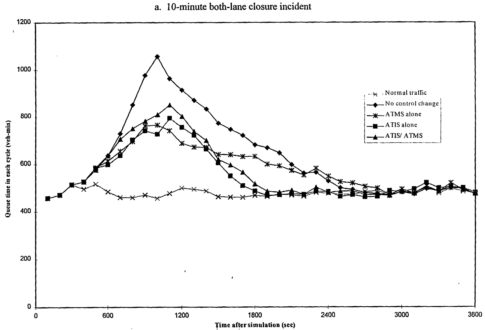
Figure 5-5 Congestion duration: different control strategies
