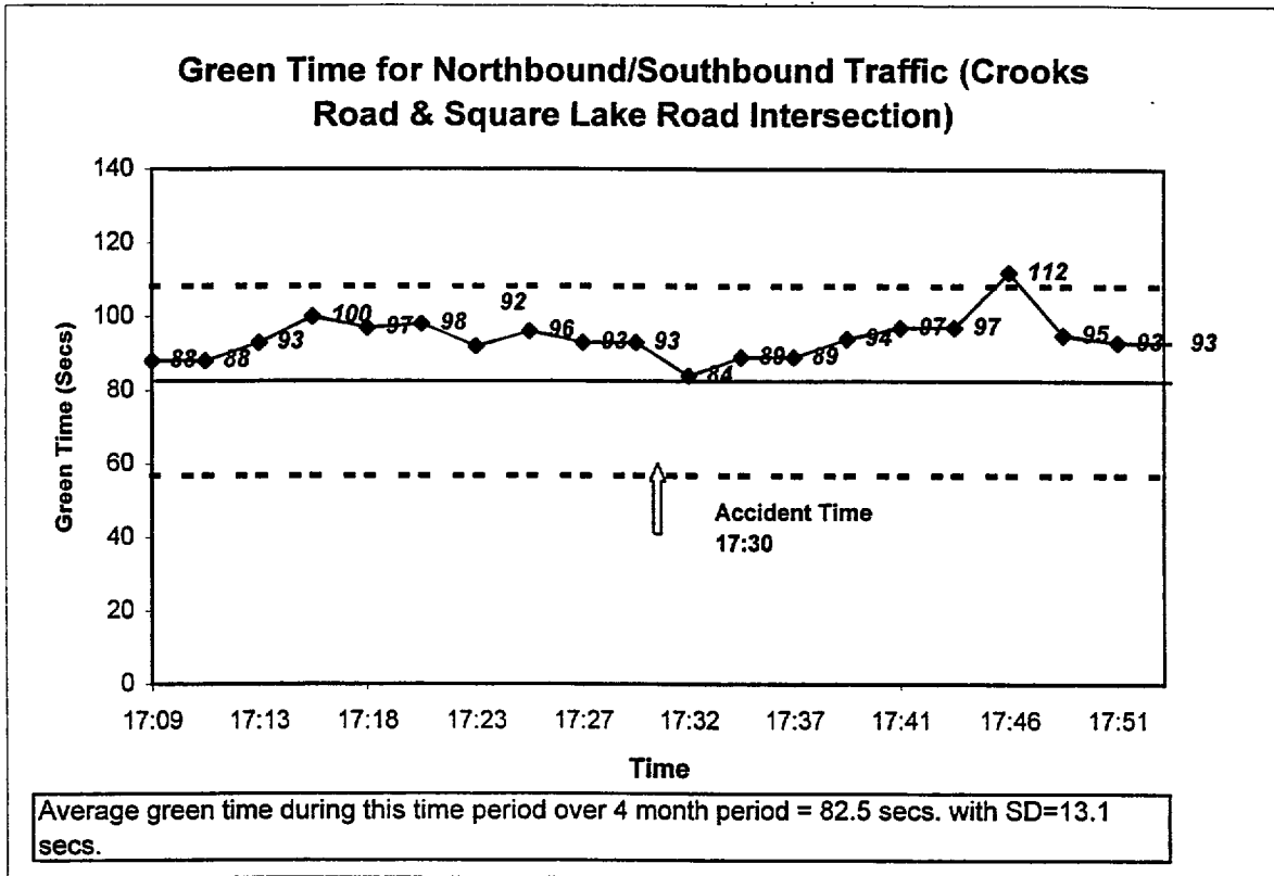
Figure 6-8 (Cont.) Green Time Response for Crash # 7.
