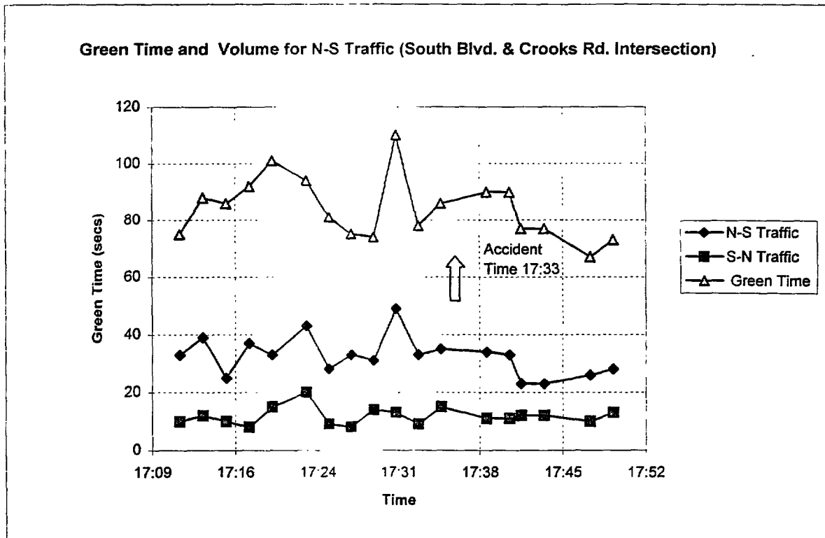
Figure 6-10 (Cont.) Volumes For Crash #2
