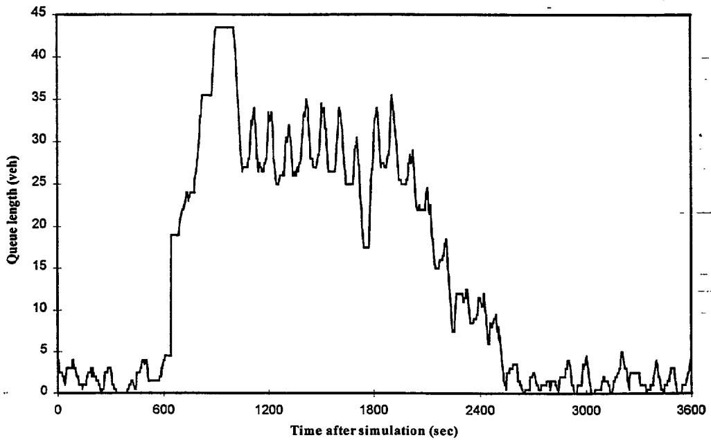
Figure 5-2 Queue length obtained every four seconds
