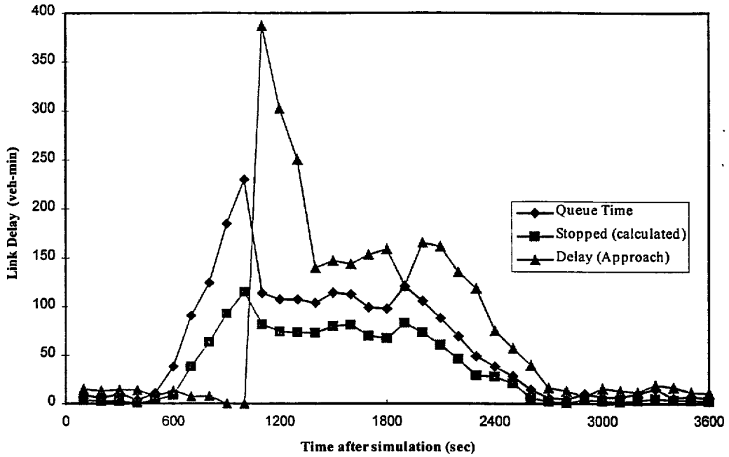
Link (9,10), Through traffic, 10-minute both-lane closure incident
