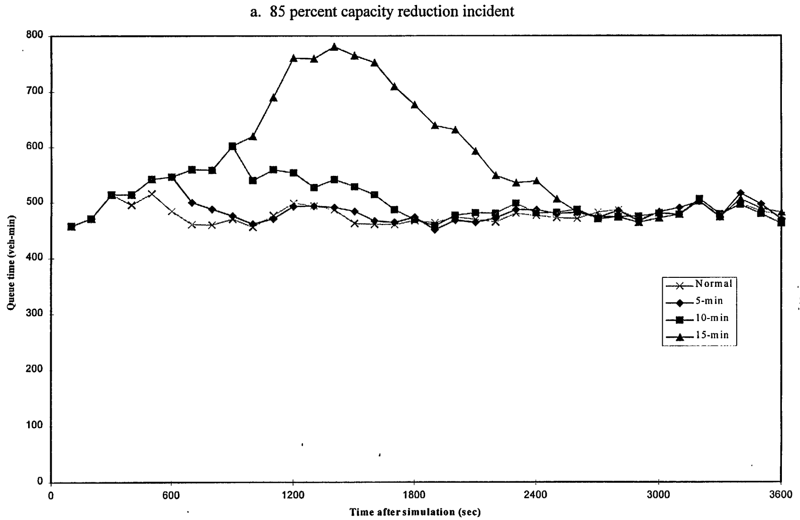
Figure 5-3 Congestion duration: no control change
