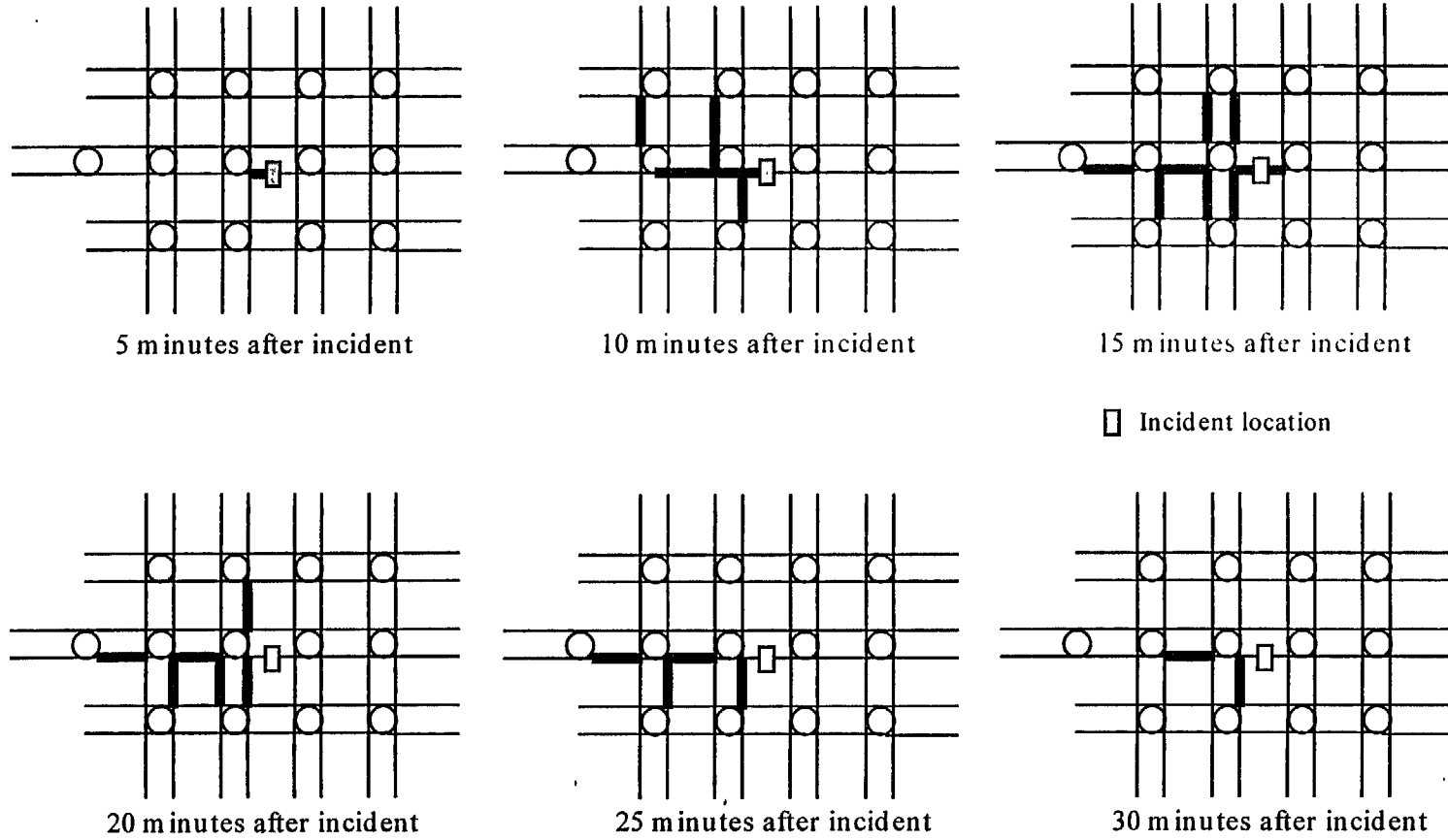
Figure 5-4 (a) Affected links and duration of congestion: no control change
