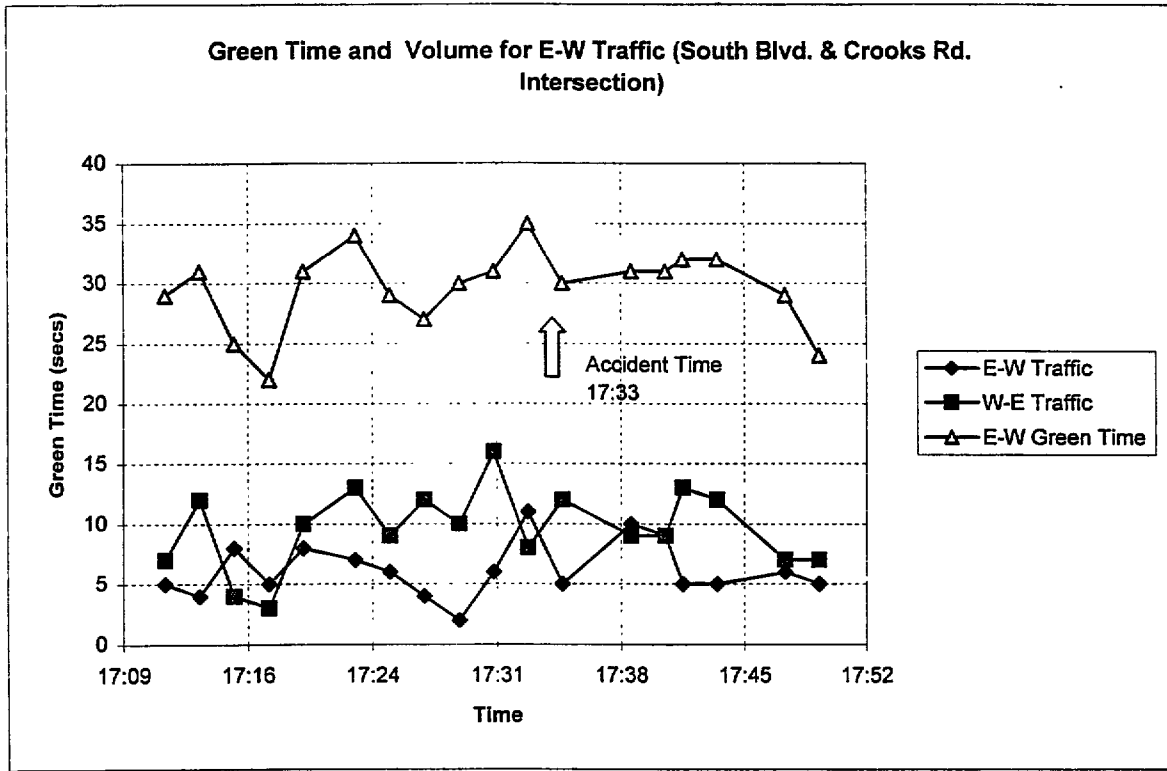
Figure 6-10 Volumes For Crash #2
