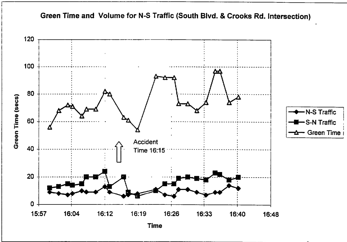
Figure 6-11 Volumes For Crash #4
