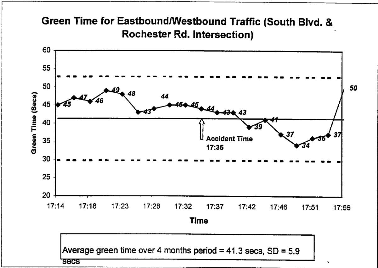
Figure 6-4 Green Time Response for Crash #3
