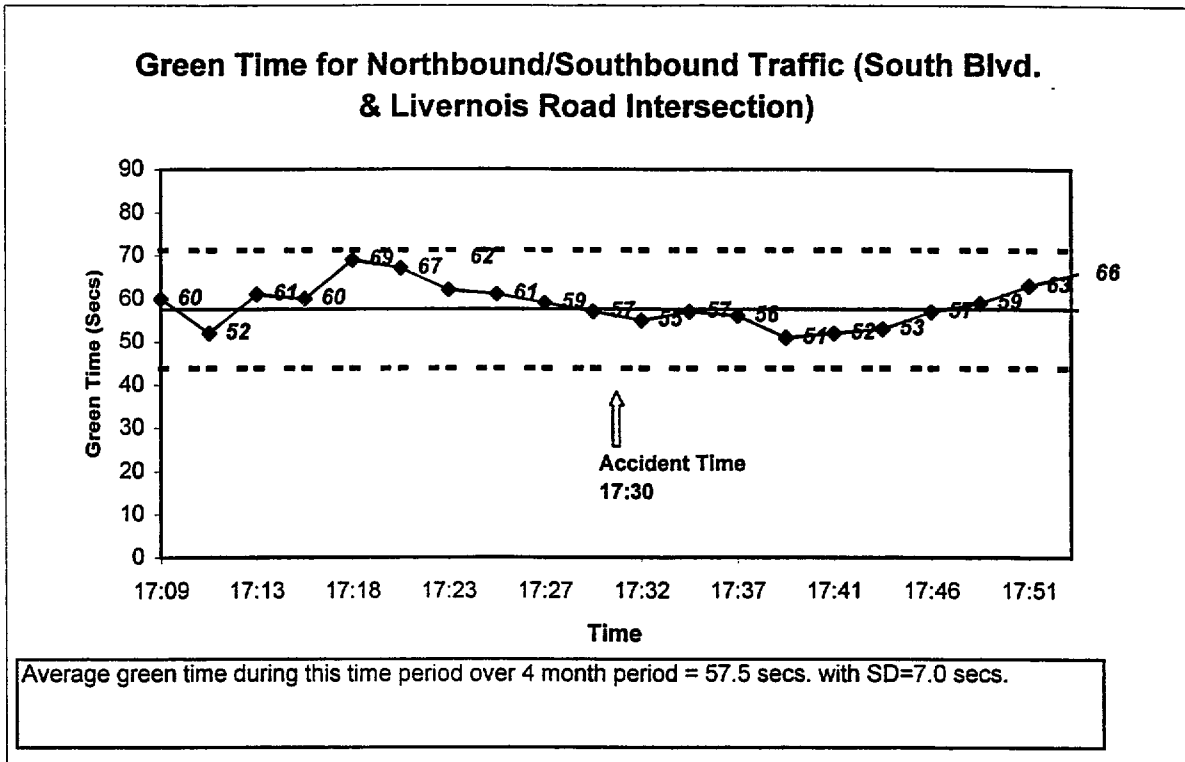
Figure 6-8 (Cont.) Green Time Response for Crash #.7
