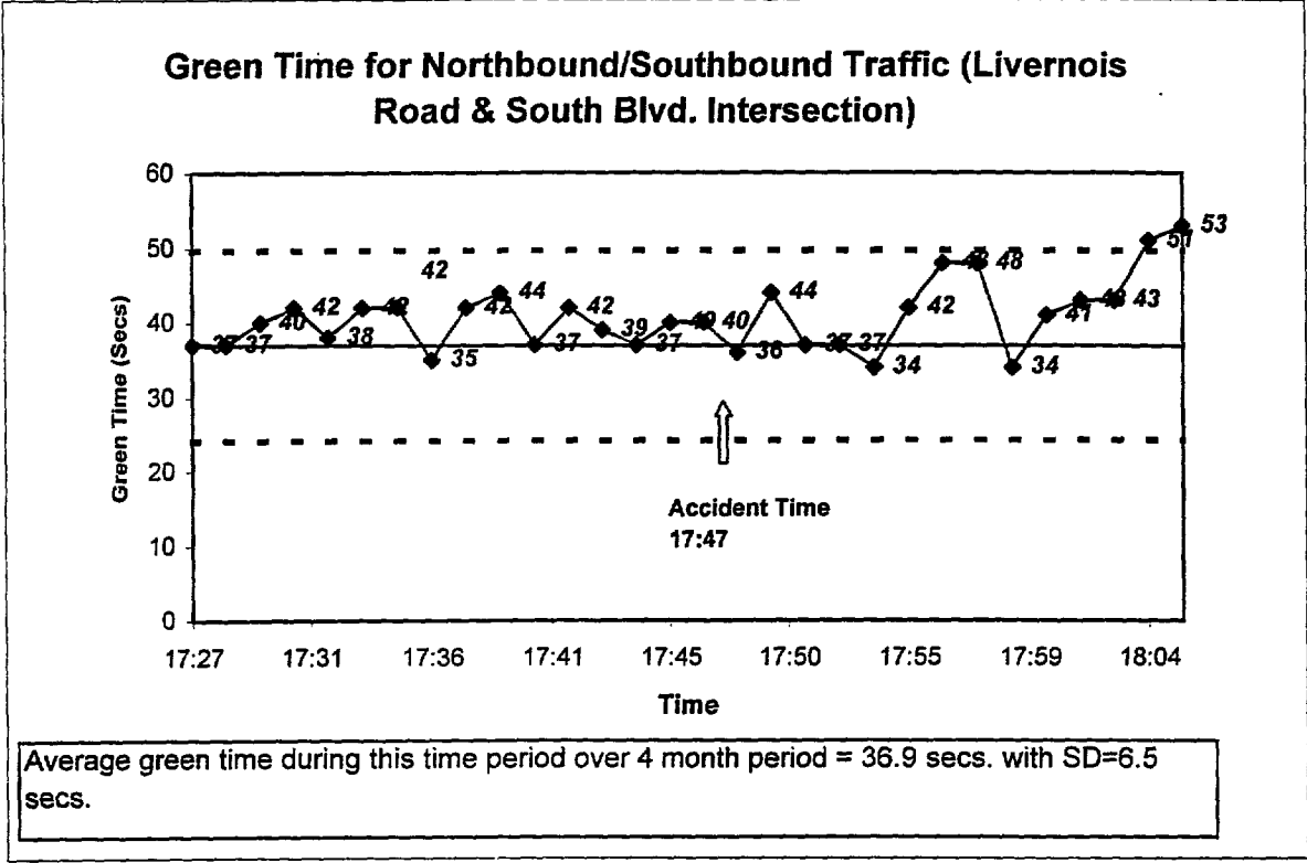
Figure 6-7 Green Time Response for Crash # 6
