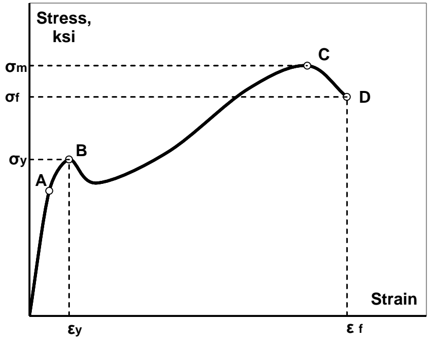
Figure 4.6 Tensile stress-strain curve for steel (a = elastic limit, b = upper yield stress, c = ultimate stress, d = breaking stress)
