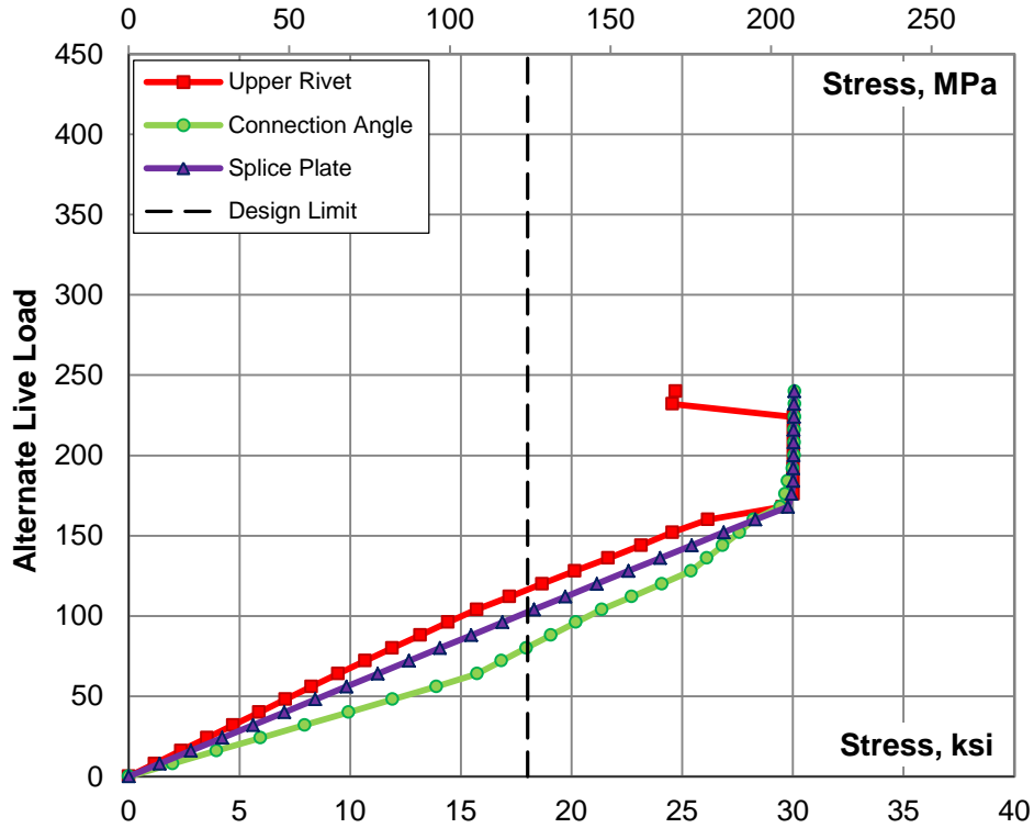
Figure 4.53 Stresses due to gradually increased Cooper E loading, bridge #2
