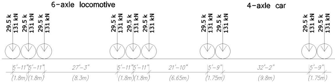
Figure 4.15 Axle configuration of the calibration train
