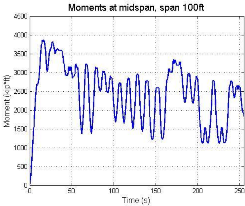
Figure 3.9 Moment at mid span for 100 ft span length
