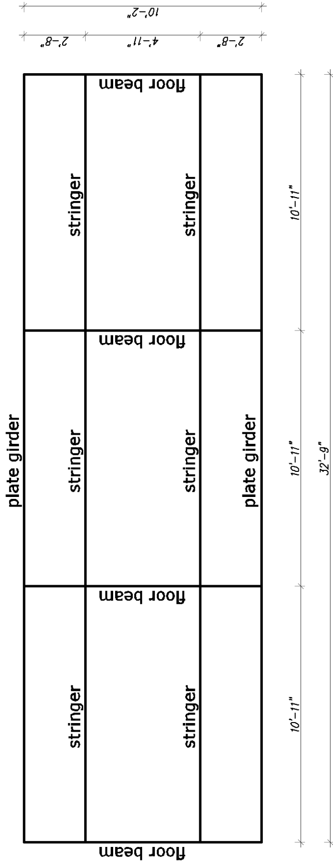
Figure 4.9 Floor system of bridge #1
