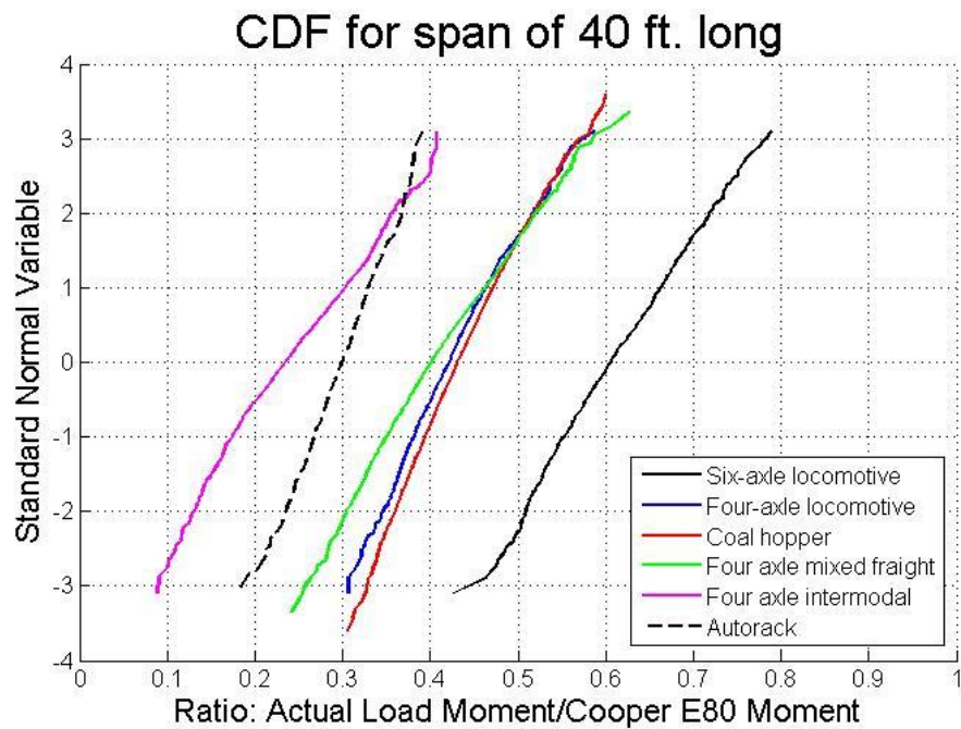
Figure 3.14 CDF of ratio of actual load moment to Cooper E80 Moment for 40 ft span, each type of car plotted separately
