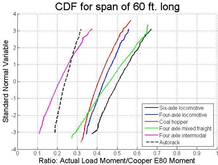
Figure 3.16 CDF of ratio of actual load moment to Cooper E80 Moment for 60 ft span, each type of car plotted separately
