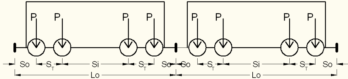
Figure 3.6 Dimensions used for analysis
