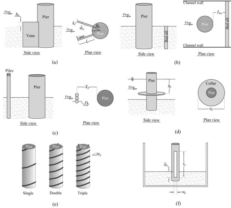
Figure 3.6 Flow-altering countermeasures: (a) submerged vanes; (b) bed sill; (c) sacrificial piles; (d) collar; (e) threading; (f) pier slot. From Tafarojnoruz et al. (2012)
