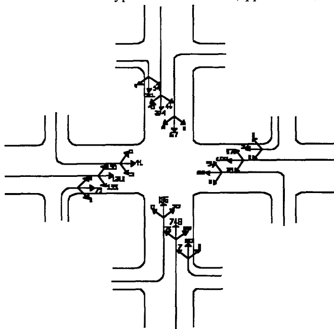
Figure 3.2 Intersection geometry and volume
