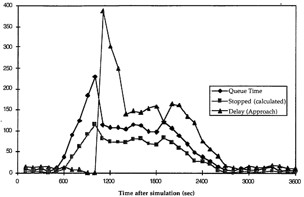
Figure 4.1 Statistics from NETSIM for determining congestion period
