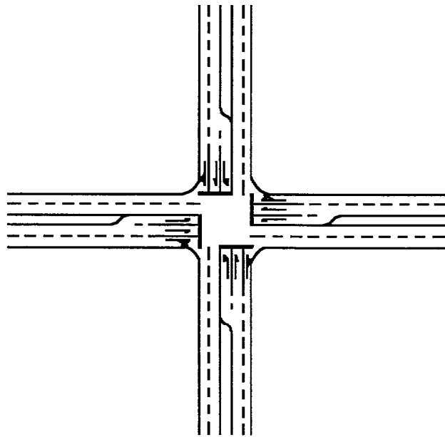
Figure 3.2 Intersection geometry and volume
