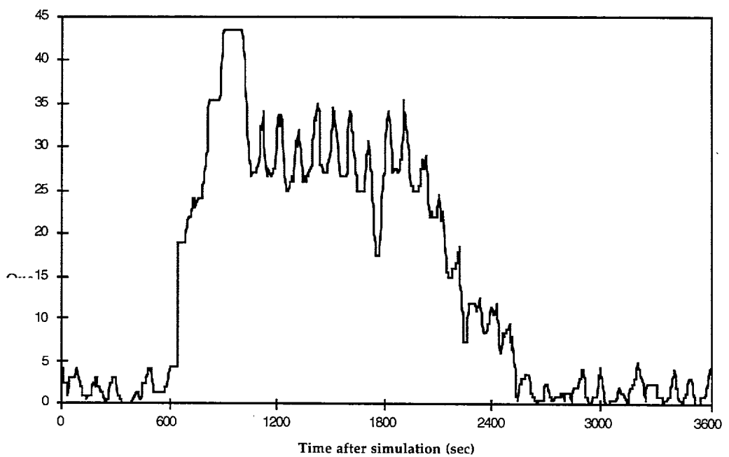
Figure 4.2 Queue length obtained every four seconds
