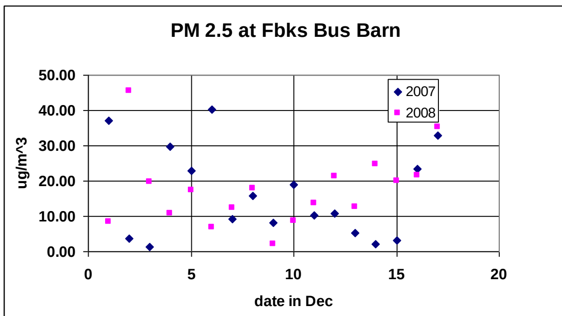
Fig. 14 Comparison of PM vls at the Bus Barn for December
