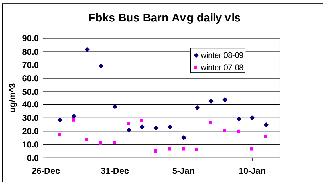
Fig. 12 Avg Daily PM 2.5 vls at FNSB Bus Barn from Dec 27 – Jan 11
