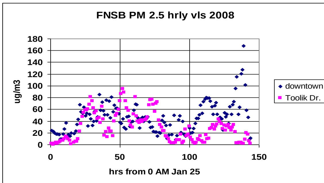
Figure 13 Jan 25 - 30 RAMs hourly PM vs time Jan 25 is Fri [ < -30 Jan 25 8 PM till 2 PM 27 th ]
