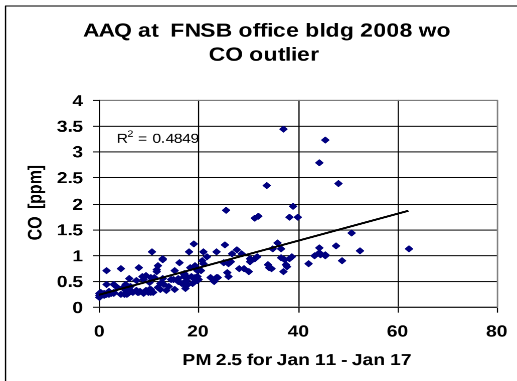
Fig. 14 Jan 11- 17 CO vs PM
