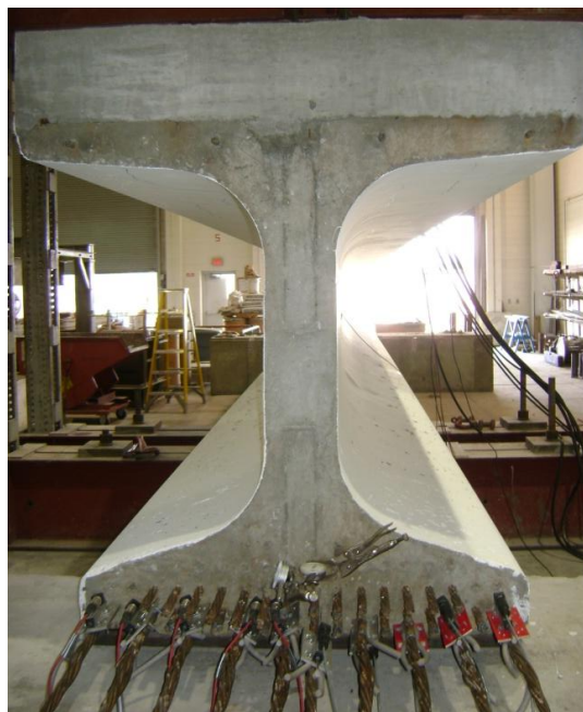
Figure 50 Shear Test Strand Instrumentation
