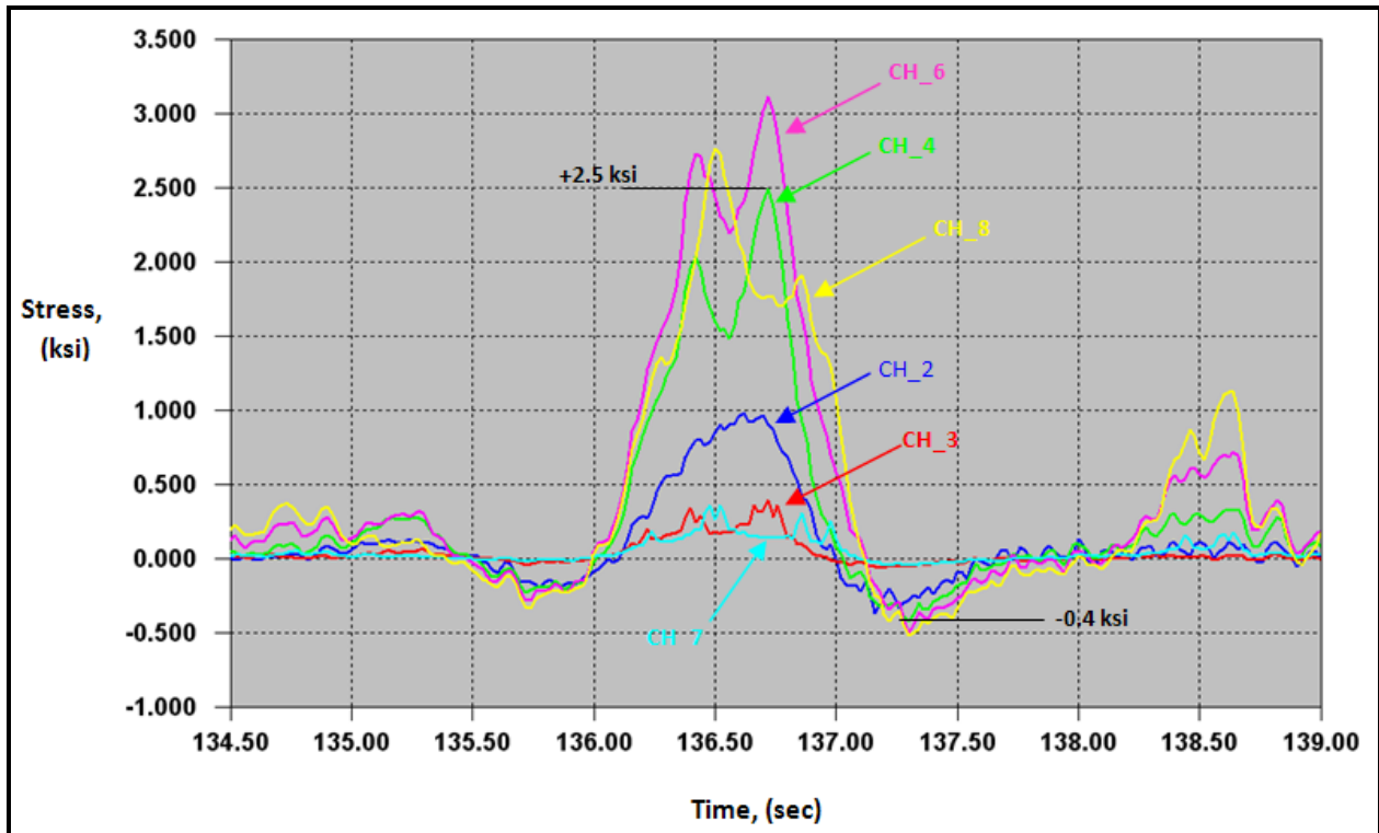
Figure D.1 Maximum stress range recorded in CH_4 from triggered data.
