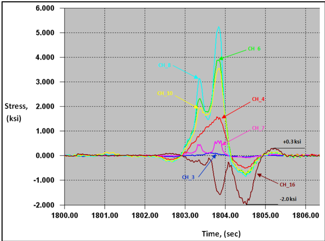
Figure D.7 Maximum stress range recorded in CH_16 from triggered data.
