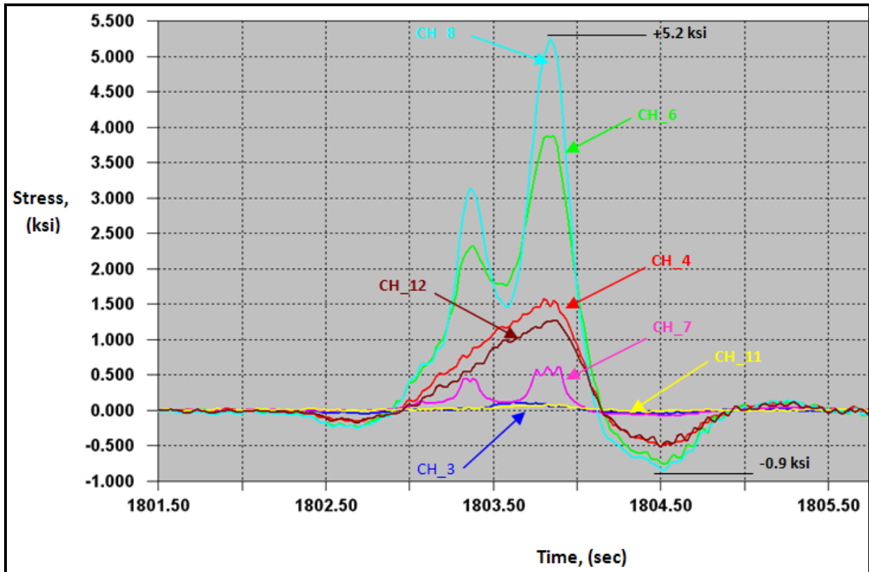
Figure D.3 Maximum stress range recorded in CH_8 from triggered data.
