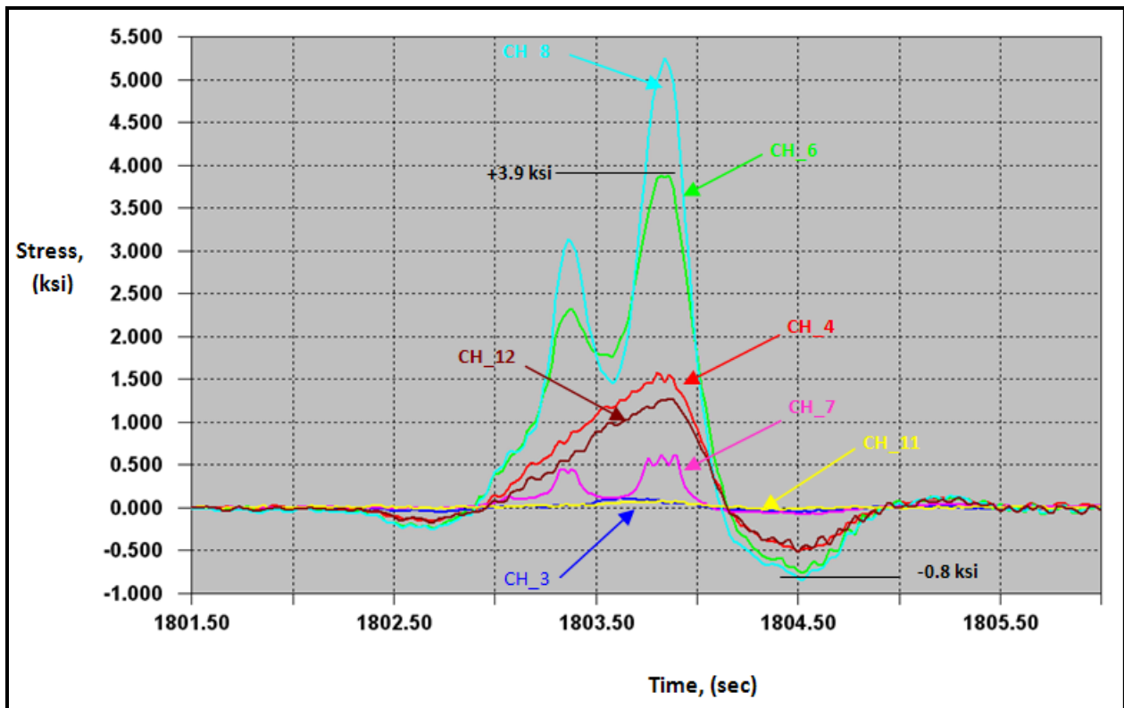
Figure D.2 Maximum stress range recorded in CH_6 from triggered data.
