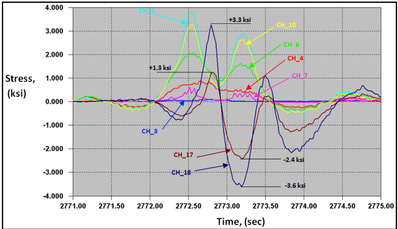
Figure D.8 Maximum stress range recorded in CH_17 & CH_18 from triggered data.
