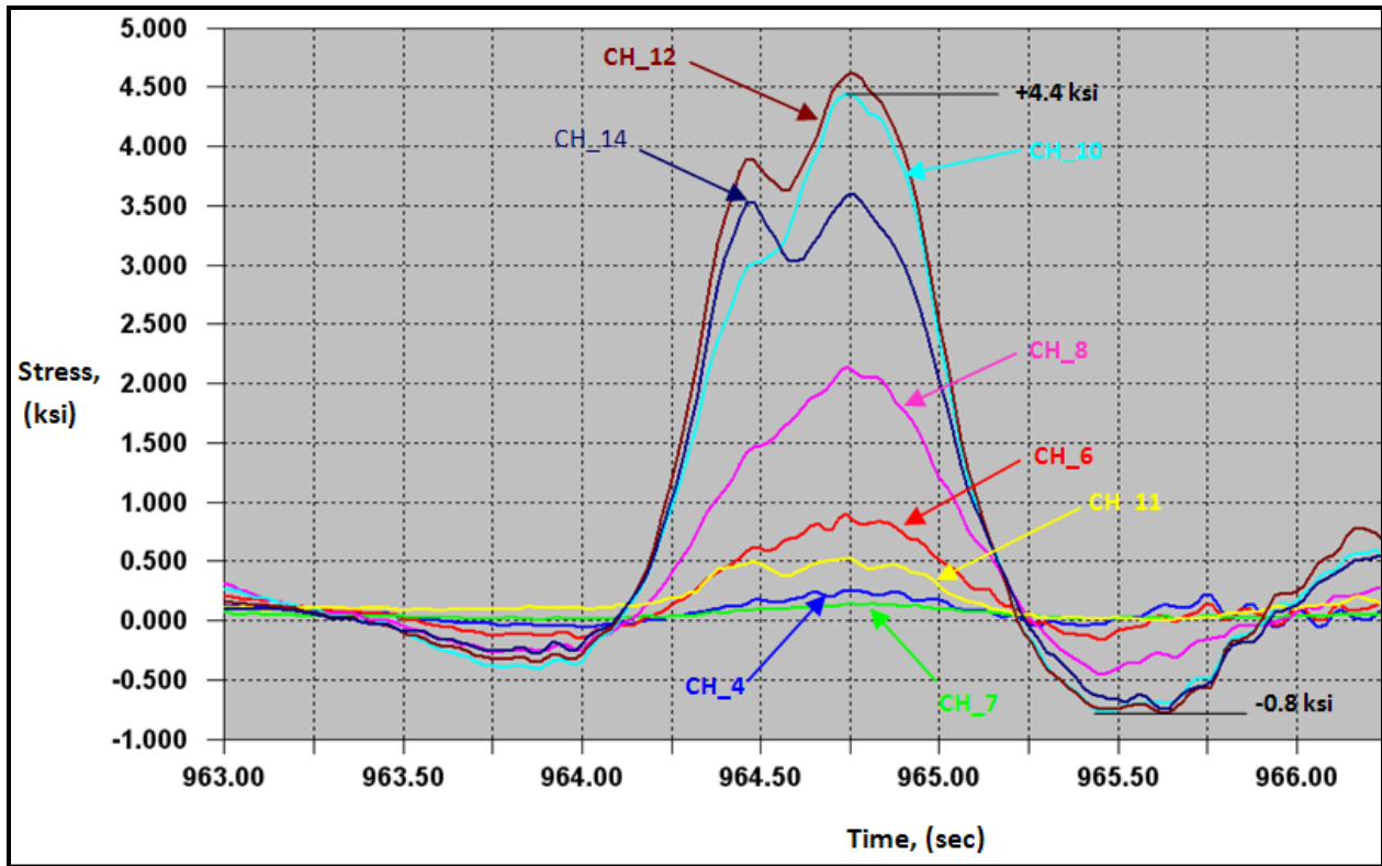
Figure D.4 Maximum stress range recorded in CH_10 from triggered data.
