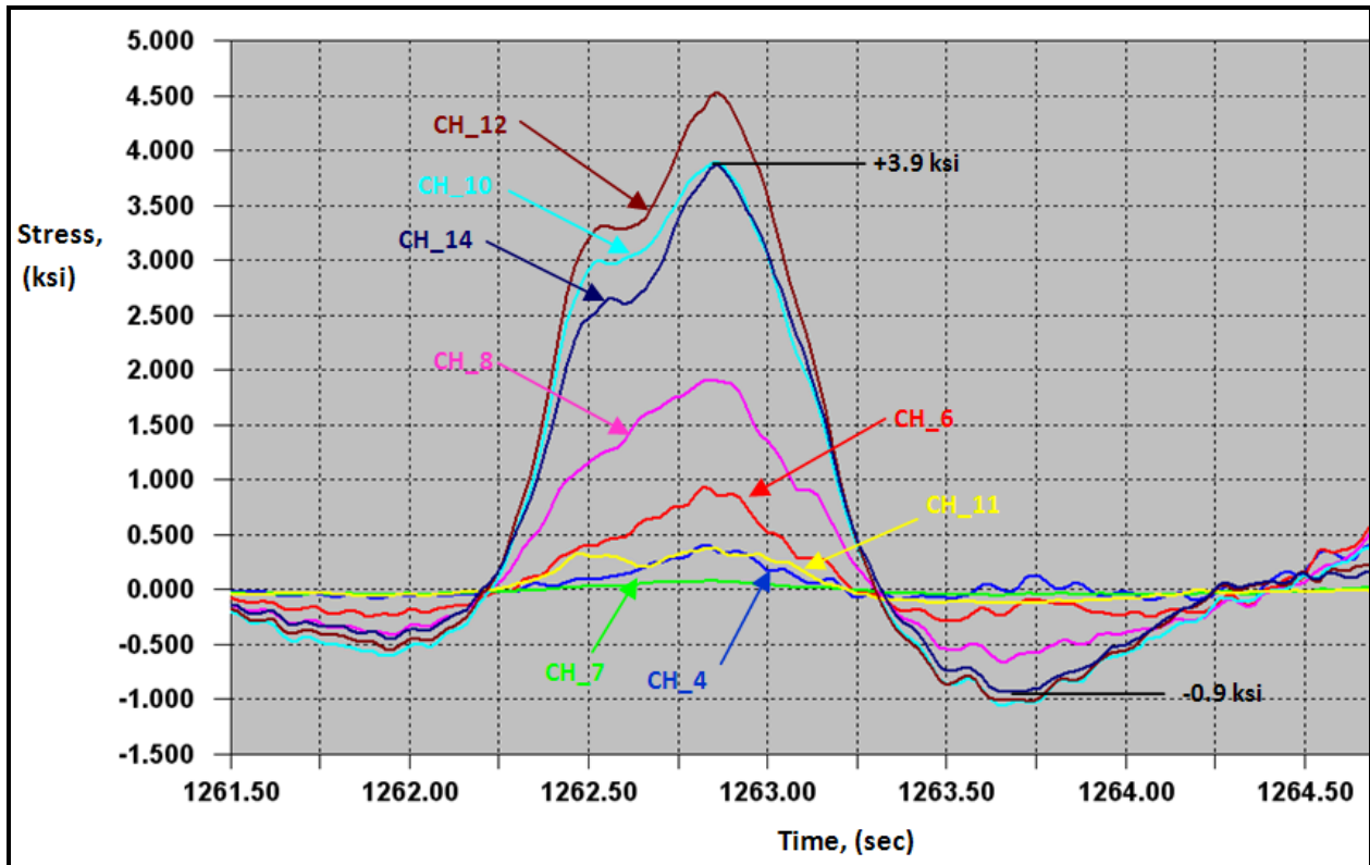
Figure D.6 Maximum stress range recorded in CH_14 from triggered data.
