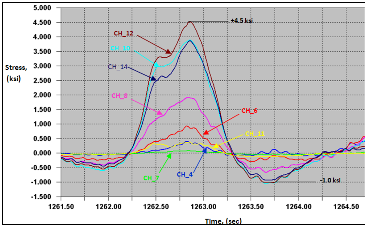
Figure D.5 Maximum stress range recorded in CH_12 from triggered data.
