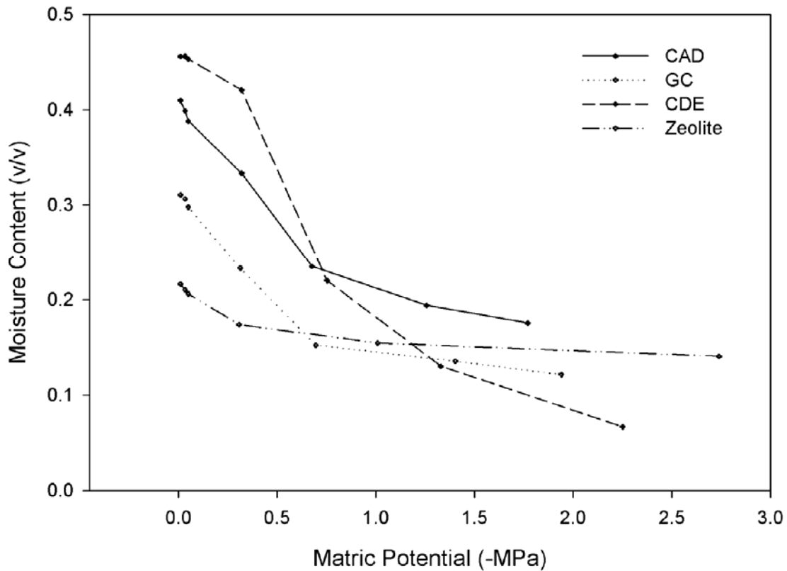
Figure 1. Water release curves for four inorganic amendments
