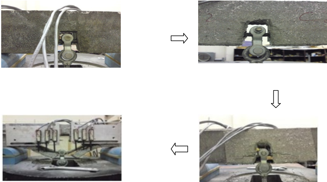
Figure 3.10 Test Procedure and Progression
