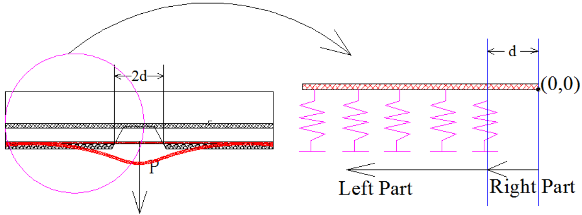
Figure 3.16 Model Explanation
