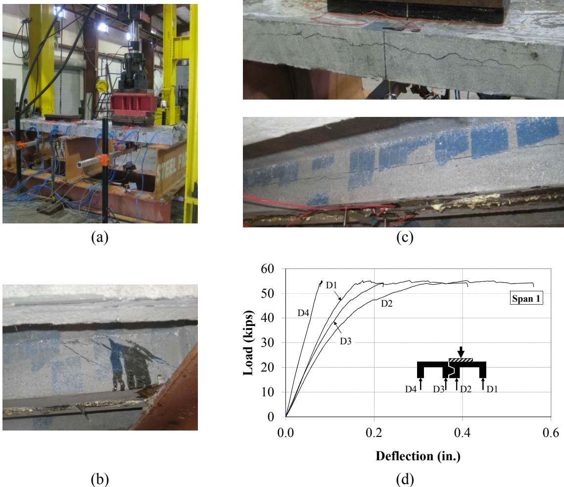
Figure 2.10 Residual Strength Test with Load on Edge of Deck-to-Deck Connection: (a) Test Setup; (b) Shear Cracks; (c) Longitudinal Cracks; and (d) Load-Deflection Responses
