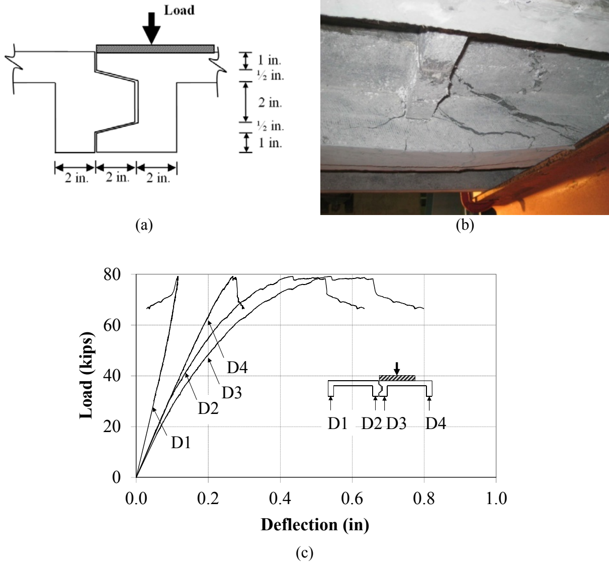
Figure 2.5 Testing of Deck-to-Deck Connection: (a) Schematics of the Connection; (b) Mode of Failure; and (c) Load-Deflection Responses
