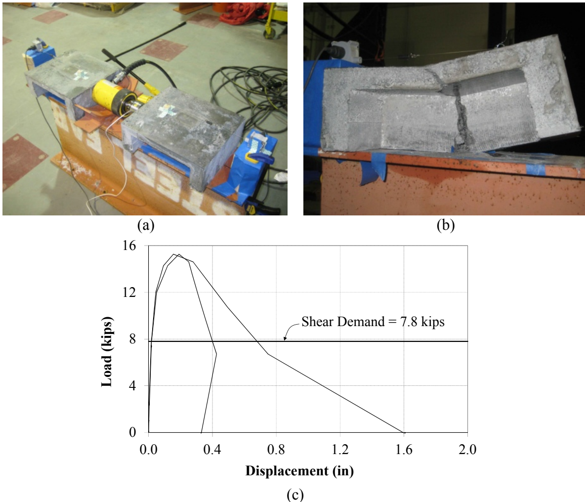
Figure 2.2 Testing of Deck-to-Girder Connection for Shear: (a) Test Setup; (b) Mode of Failure; and (c) Load-Displacement Responses
