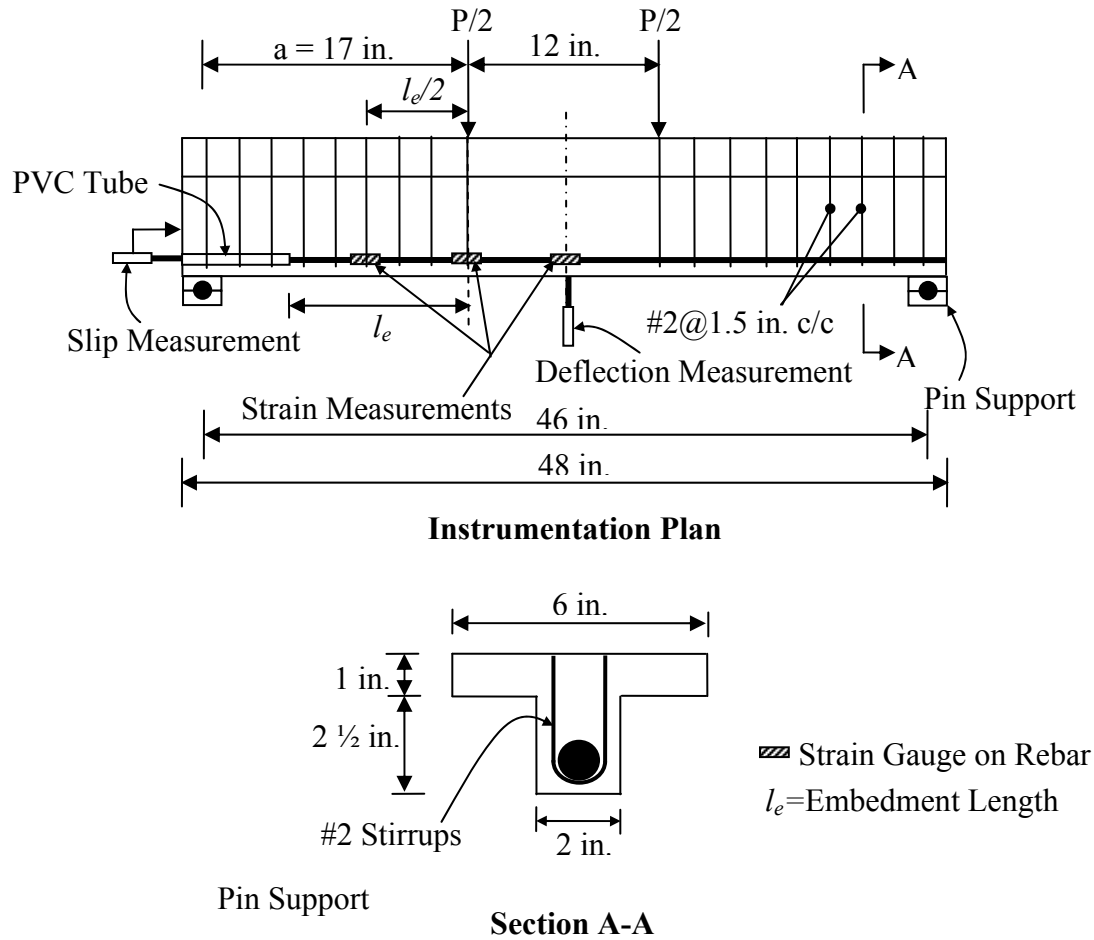
Figure 2.13 Schematics of Beam Specimens with Instrumentation
