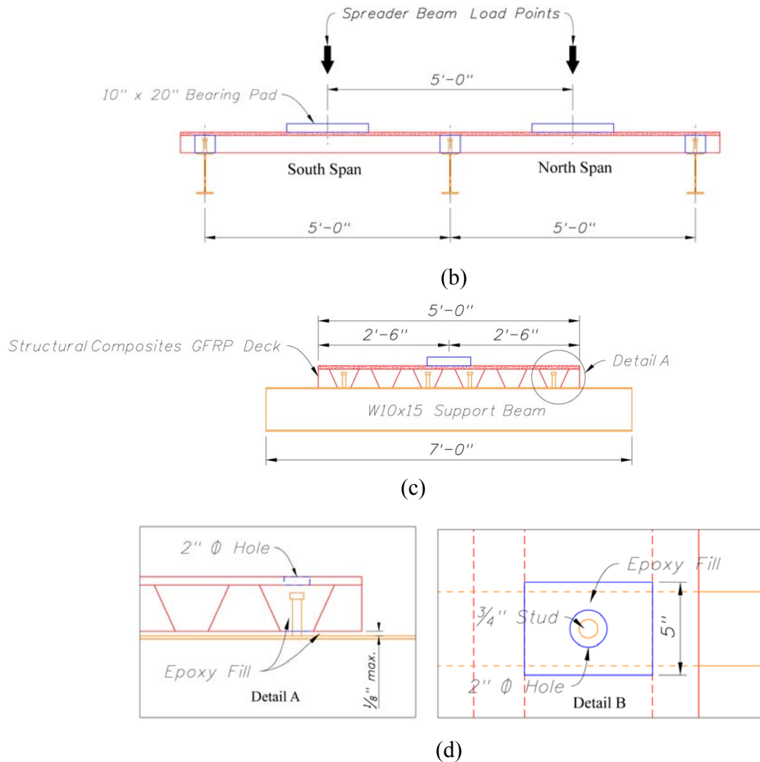
Figure 4.5 (Continued) Layout of the FRP Bridge Deck Specimen; (b) Elevation View; (c) Cross-Section; and (d) Connection Details
