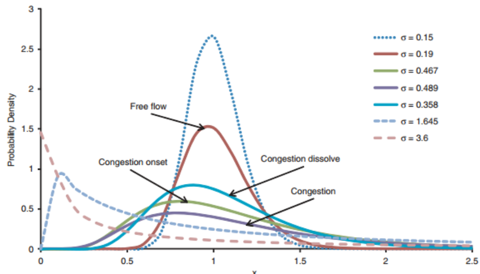
Figure 3.1 Probability density function of standard log-normal distribution
