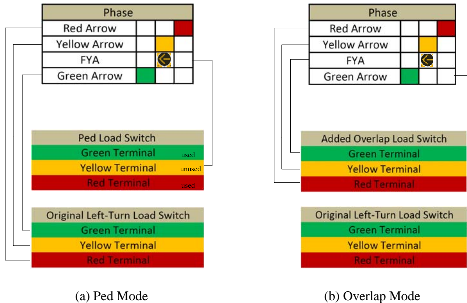
Figure 7: Typical Overlap Programming Methods for FYA PPLT
