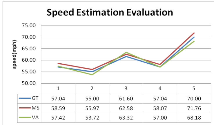
Figure 61 Speed Estimation Evaluation
