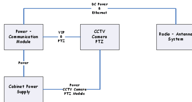
Figure 8 Function Diagram of CCTV Station (Leader 2005)
