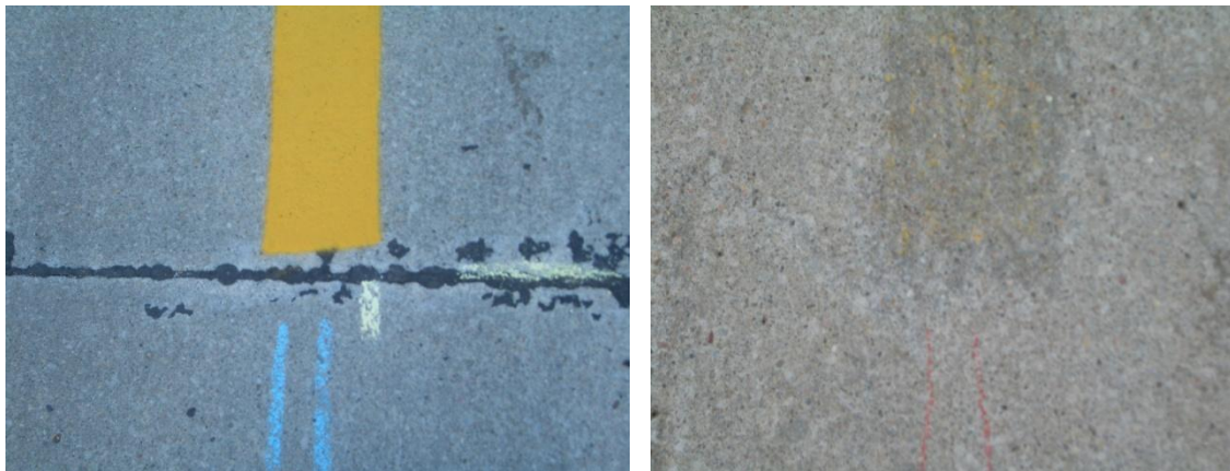
Figure 6.2 Concrete pavement condition before (left) and after (right) 10 mils oil-based paint has been removed by water blasting
