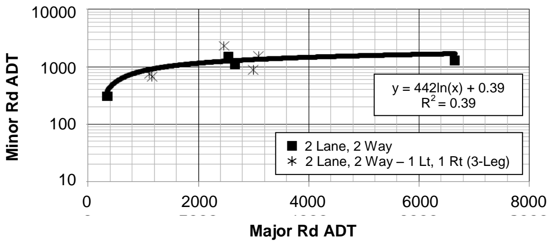
Figure 7.1 Results of Major ADT vs. Minor ADT Relationship at Intersections of 2-Lane, 2-Way Roadways with Below Average 3-yr Accident Rates, Major Rd Speed Limit = 60 mph
