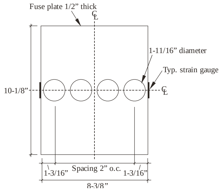
Figure 10-19. Strain gauge locations on fuse plate
