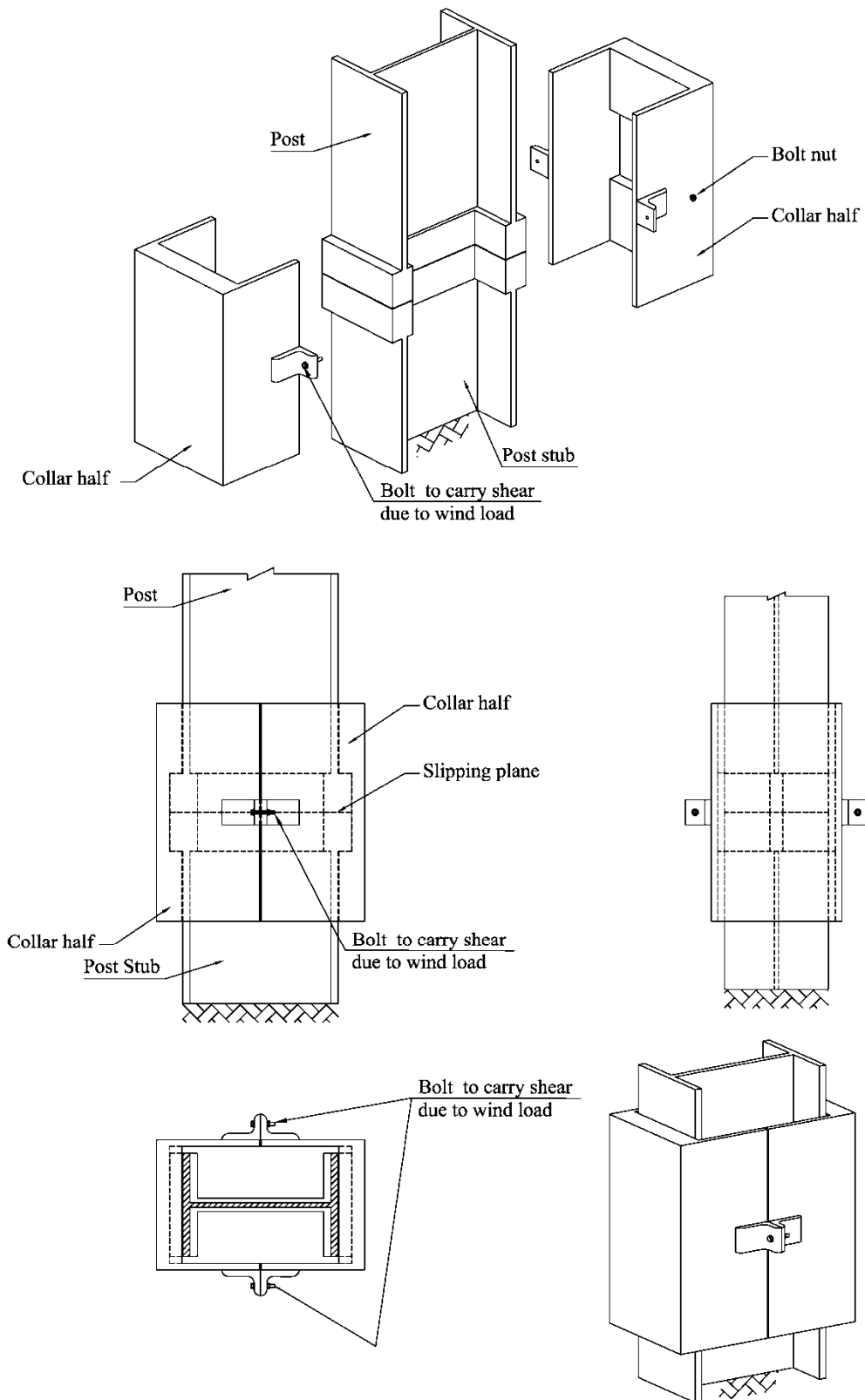
Figure 6-1. Preliminary concept of the shear-controlled moment collar connection
