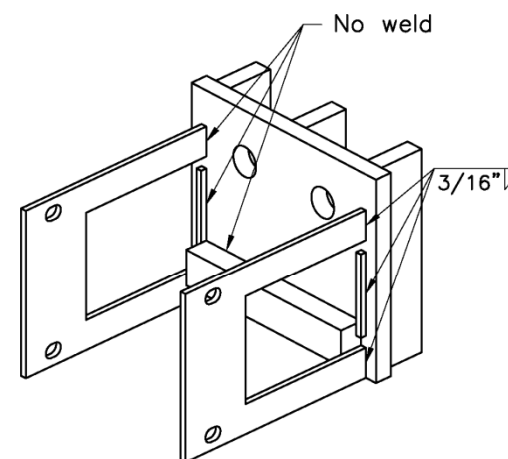
ISOMETRIC VIEW 1
