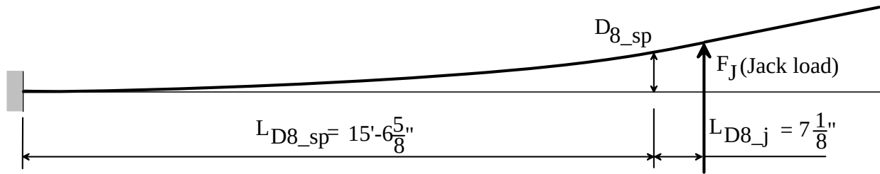
Figure 7-52. Post elastic deflection
