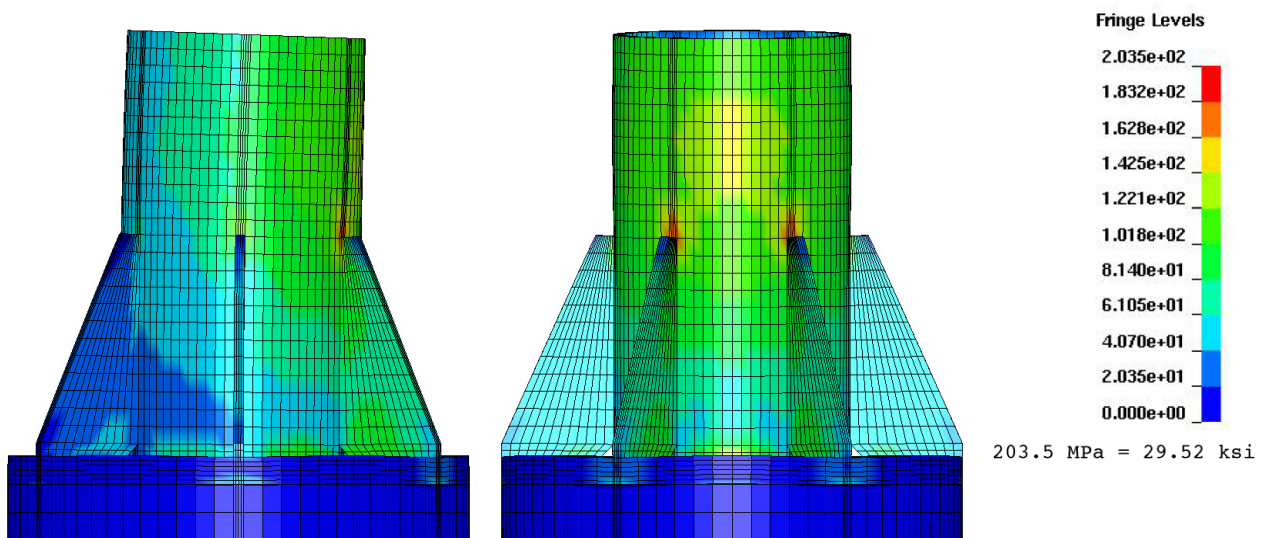
Figure 4-14. Von Mises stress contour plot under the loading condition shown in Figure 4-11B
