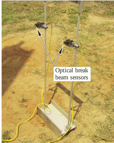
Figure 10-10. Optical break beams mounted on stand
