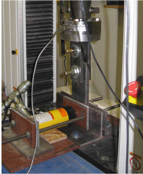
Figure 5-2. Experimental setup used to quantify static friction coefficients
