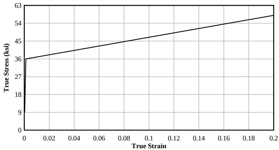
Figure 3-3. Steel material model of post and plates
