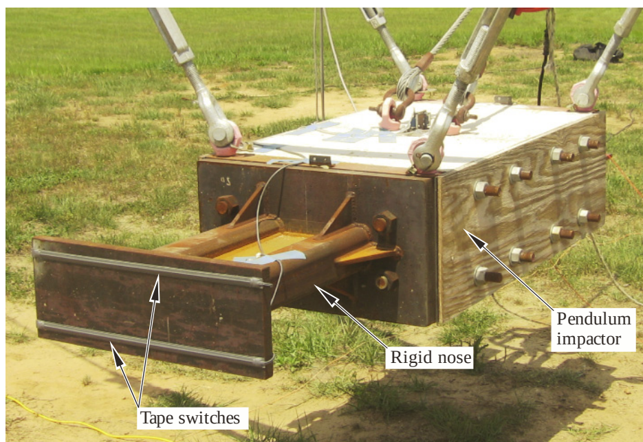
Figure 10-11. Tape switches mounted on rigid nose of impactor
