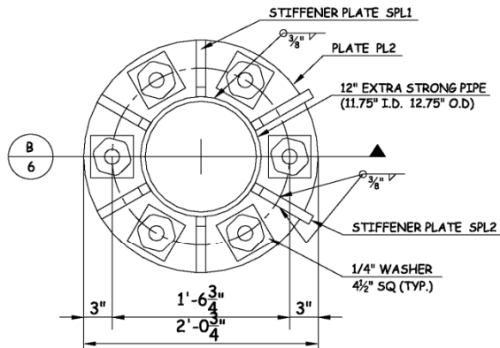
A 6 PLAN VIEW COLUMN JOINT
