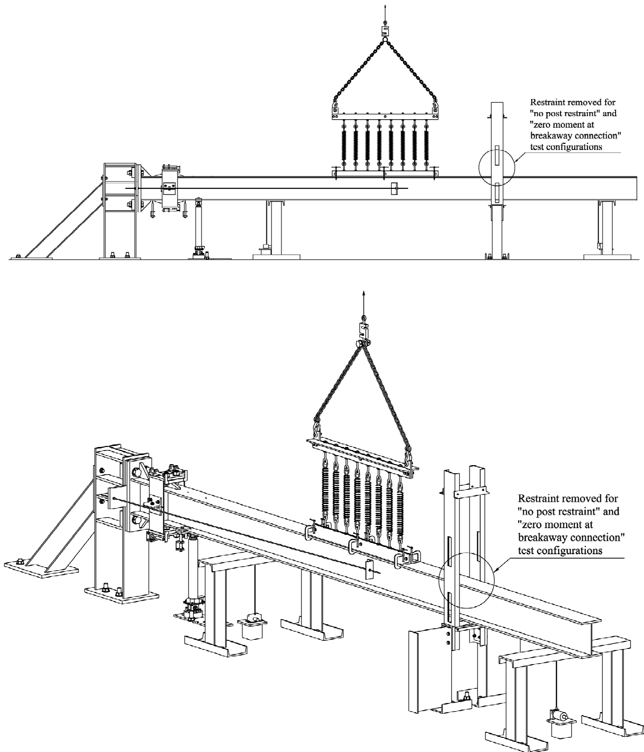
Figure 7-25. "No post restraint" and "zero moment at breakaway connection" shear test setup
