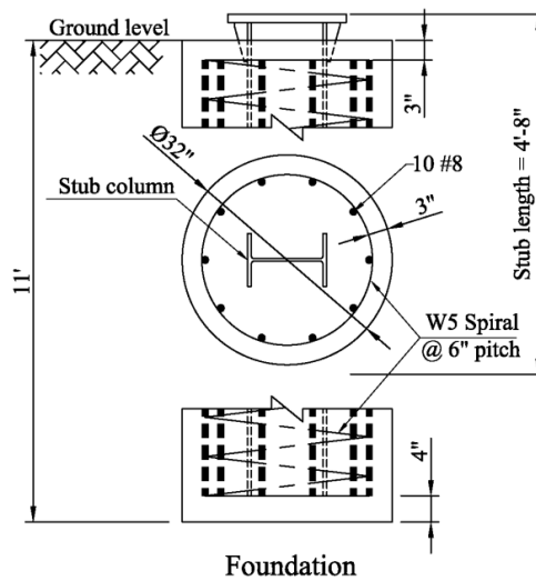
Figure 6-4. Sign support structures with shear-controlled moment collar connection: A) Elevation and plan views; B) Foundation
