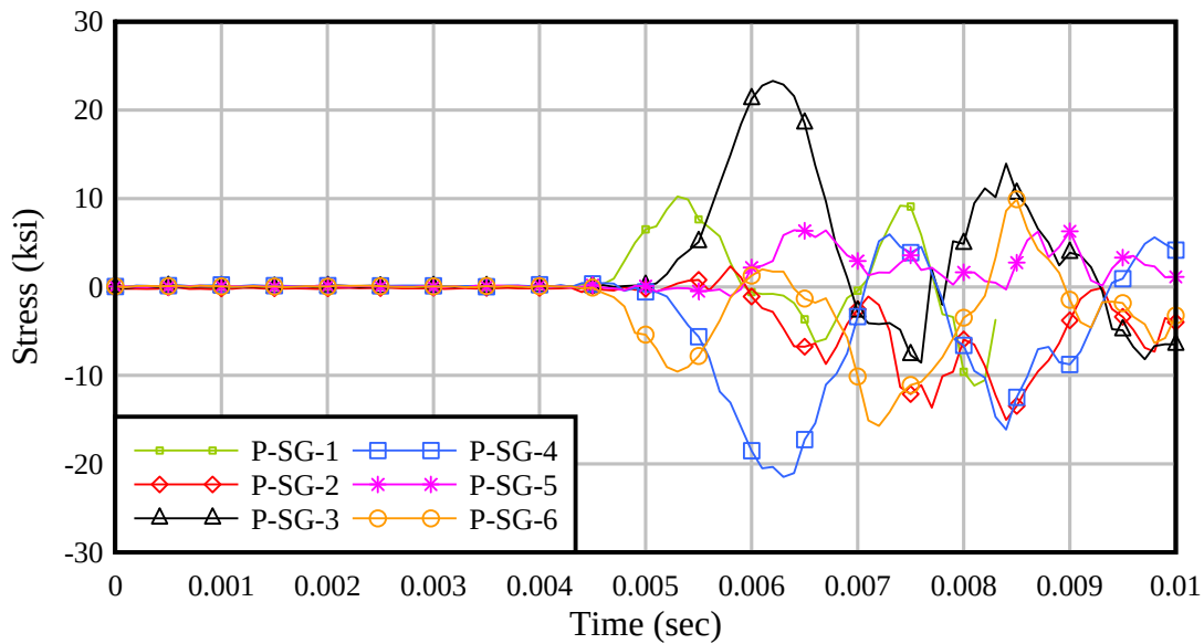
Figure 10-34. Strain gauge data converted to stress (assuming E = 29000 ksi) for test T-0-1
