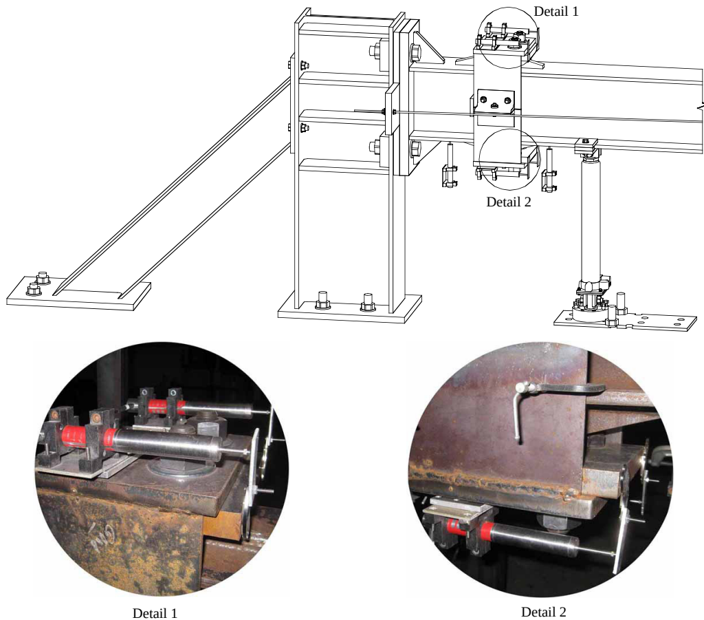
Figure 7-20. LVDTs for measuring in-plane motion of the bolted collar plates
