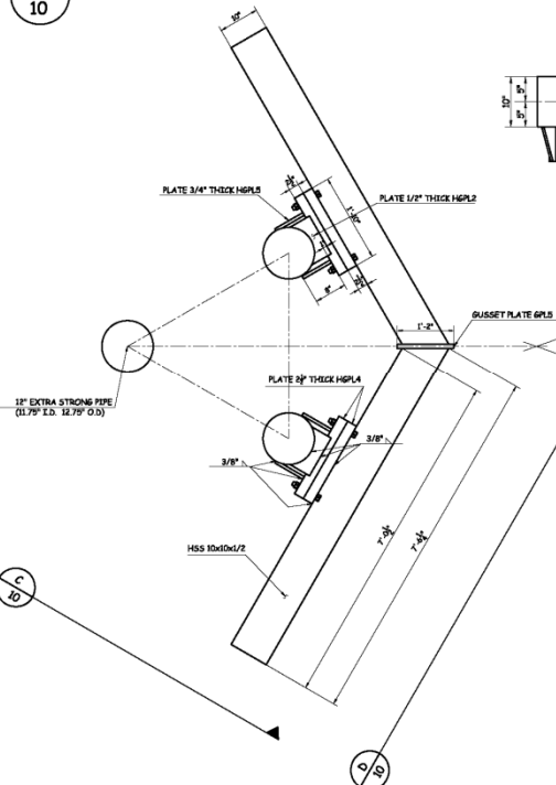
PLAN VIEW OF CABLE HANGER
