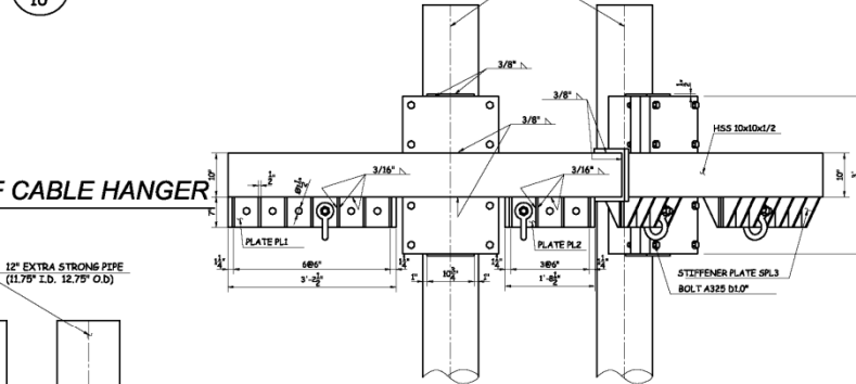
FRONT VIEW OF CABLE HANGER
