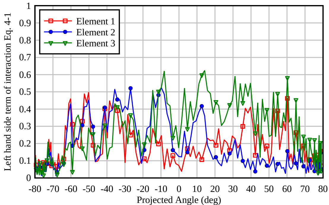
Figure 4-7. Lefthand side terms of AISC interaction equations for three column pipes at base of pylon
