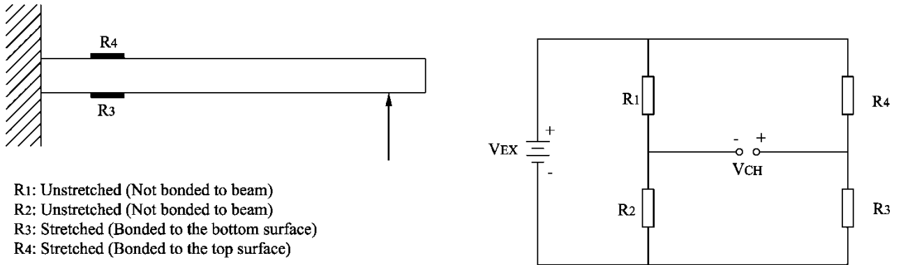
Figure 7-12. Circuit diagram of a strain gauge set
