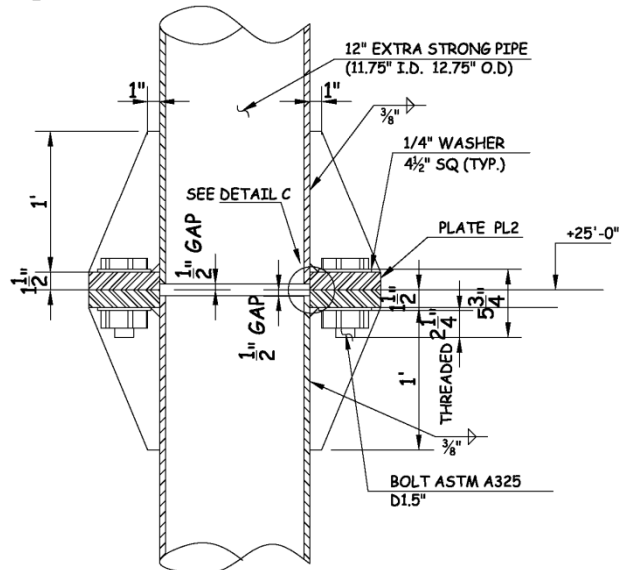
B 6 COLUMN JOINT SECTION VIEW
