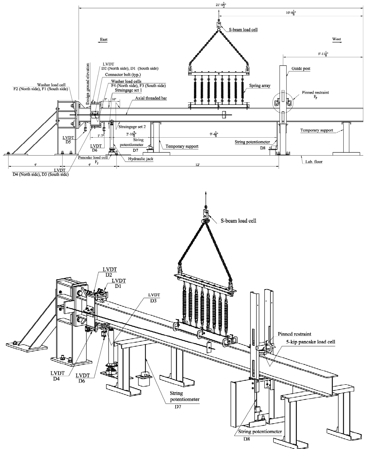
Figure 7-24. "Post pinned at fuse plate" shear test setup
