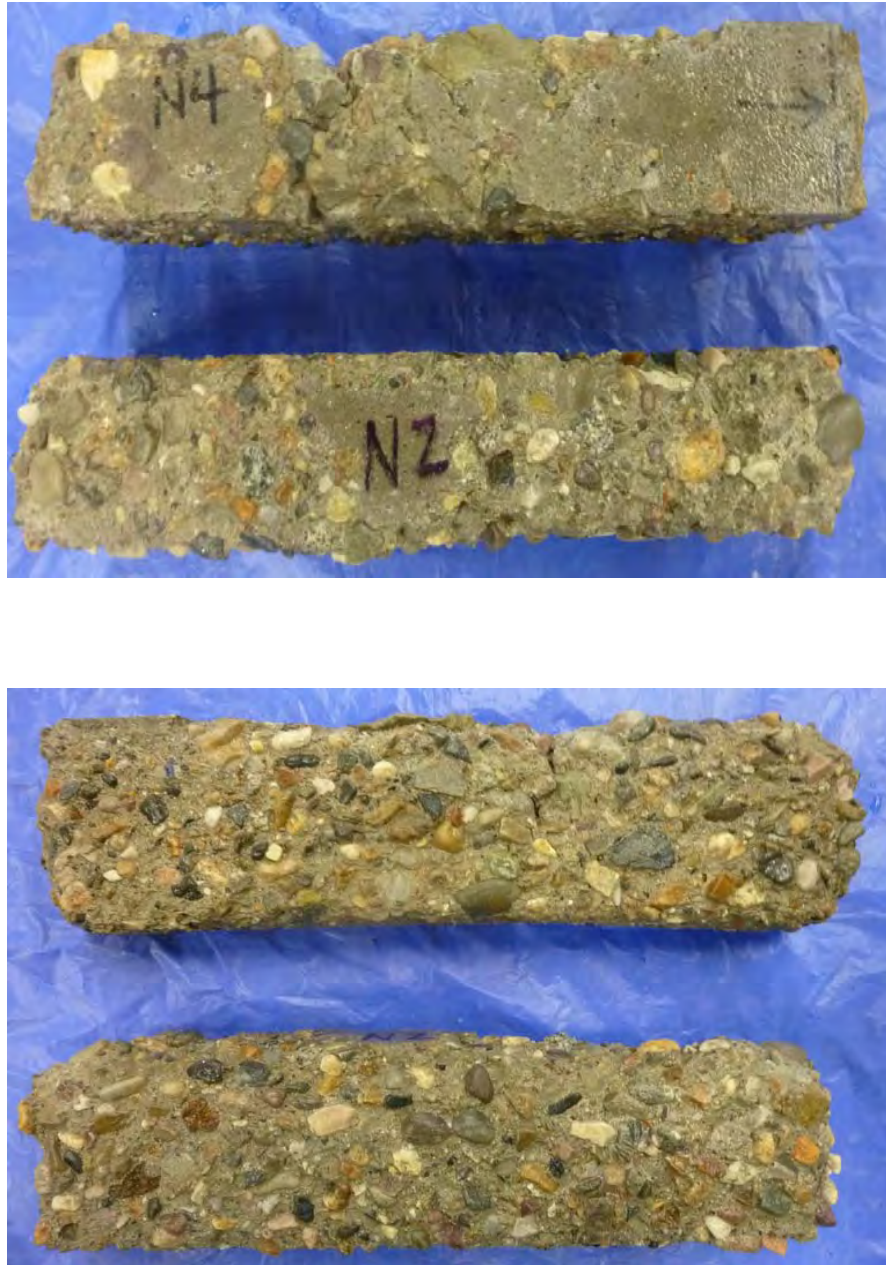
Figure 4.13 Failed Samples in the Second Batch of Concrete with NM Aggregate Sources Due to F/T Damage.
