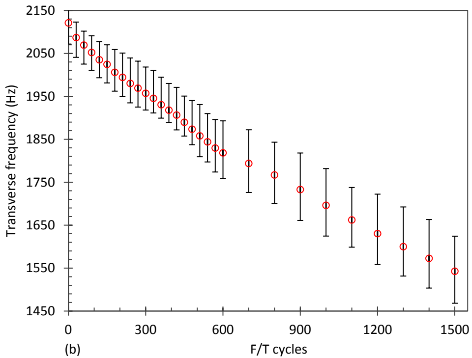
Figure 4.12 Fundamental Transverse Frequency of Concrete Samples with NM Aggregate with Respect to F/T Cycles.
