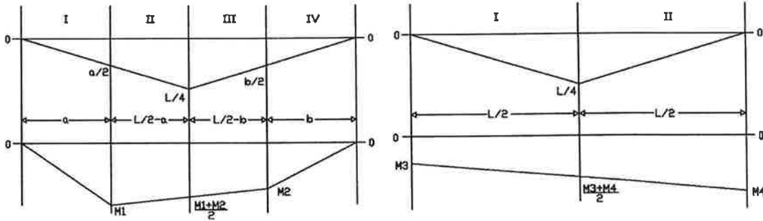
Figure 59: Moment diagrams of real and virtual forces.
