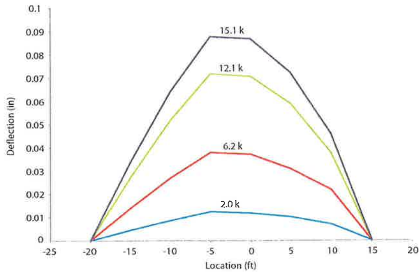
Figure 61: Deflection profile of girder during flexure test 3A at multiple loads.
