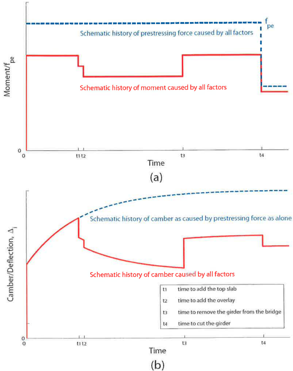
Figure 53: Illustrations of the applied moment and camber histories for the I-244 Bridge girder to the best of our knowledge.
