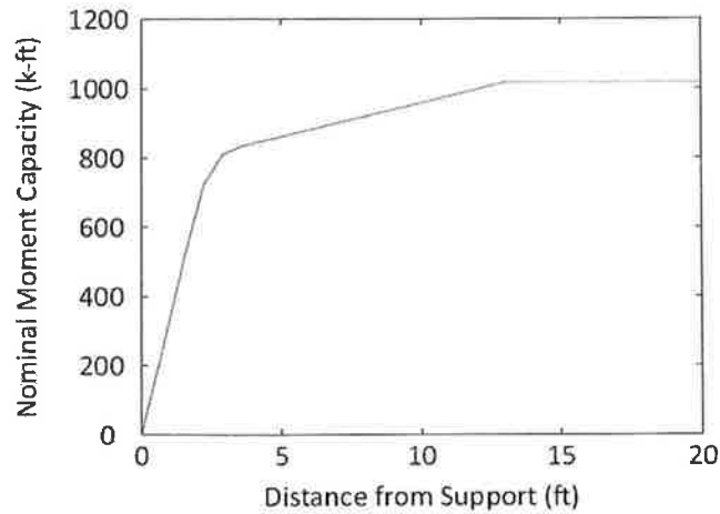
Figure 42: Nominal moment capacity for I-244 girder based on ACI-318.
