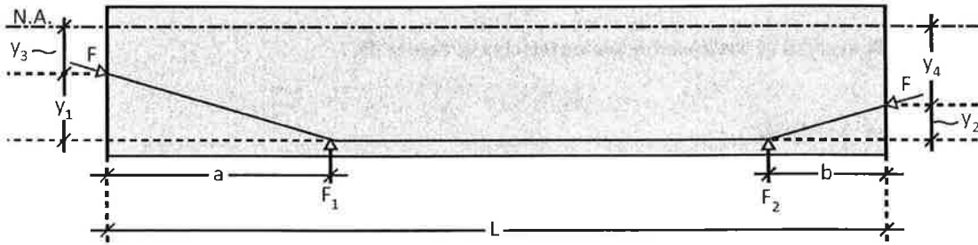
Figure 57: Free body diagram of an asymmetric prestressed girder with draped strands.
