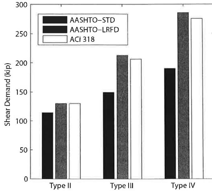
Figure 35: Comparison of ultimate shear demands between codes.
