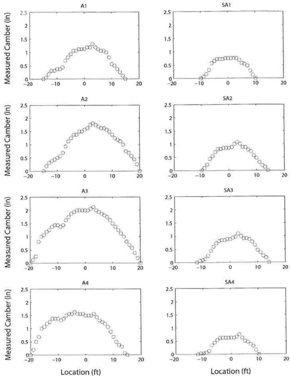
Figure 55: Typical camber profiles of the I-244 Bridge girder in an original and a shortened condition.
