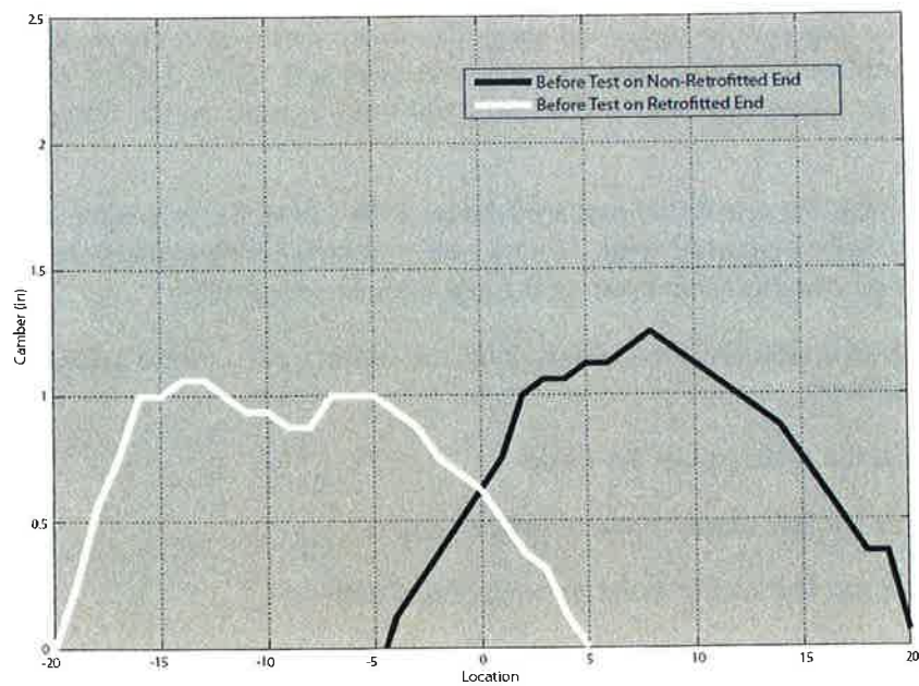
Figure 14: Summary of all measured camber profiles of the original I-244 Bridge girder before shear tests.
