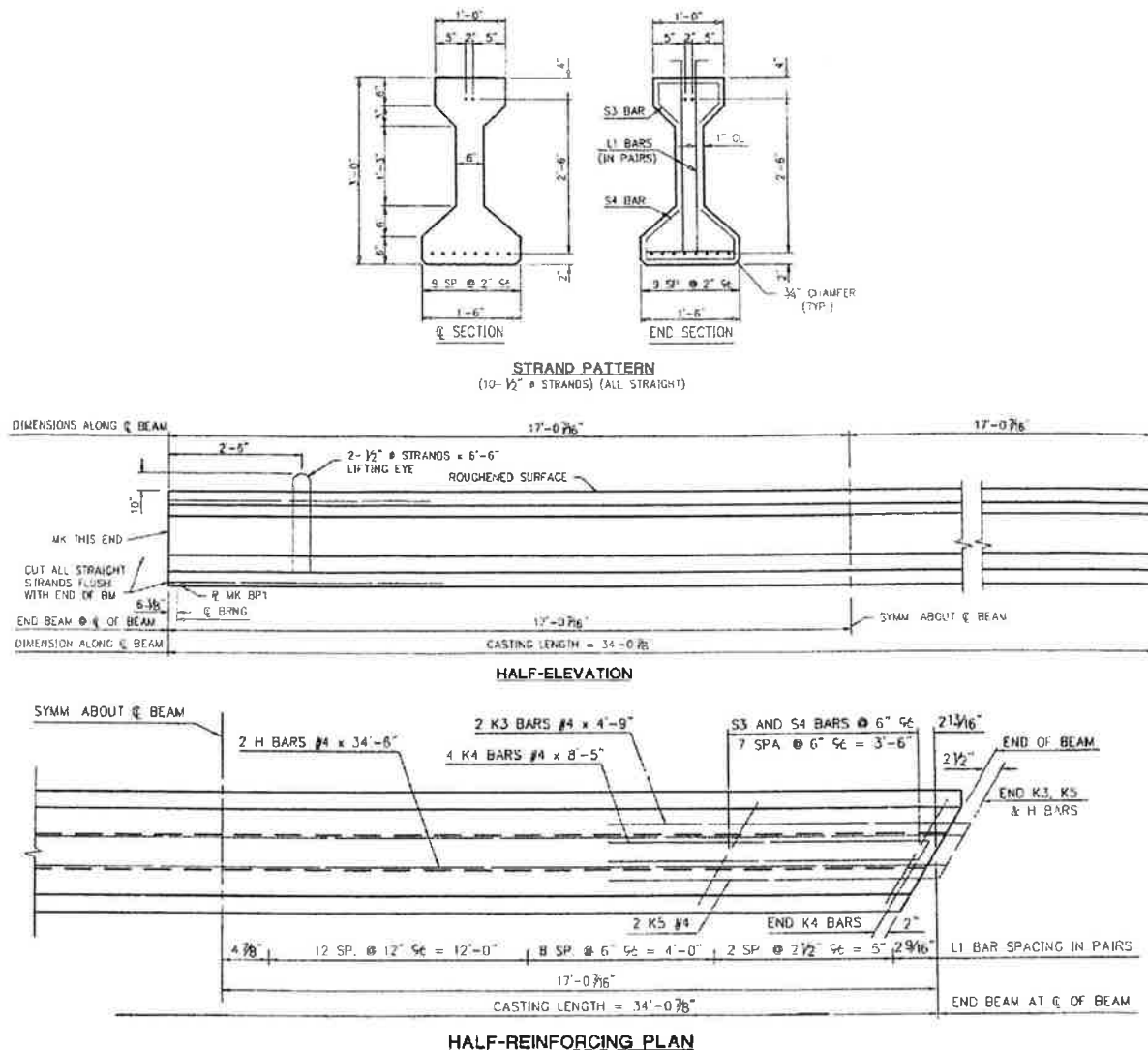
Figure 26: Elevation and details of the selected Wild Horse Creek Bridge girder (Coreslab [2007]).
