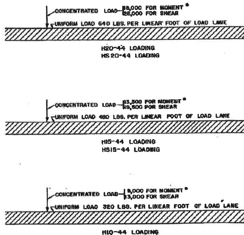
Figure 31: Lane loading for AASHTO-STD based on desired truck loading (AASHTO, 1973).
