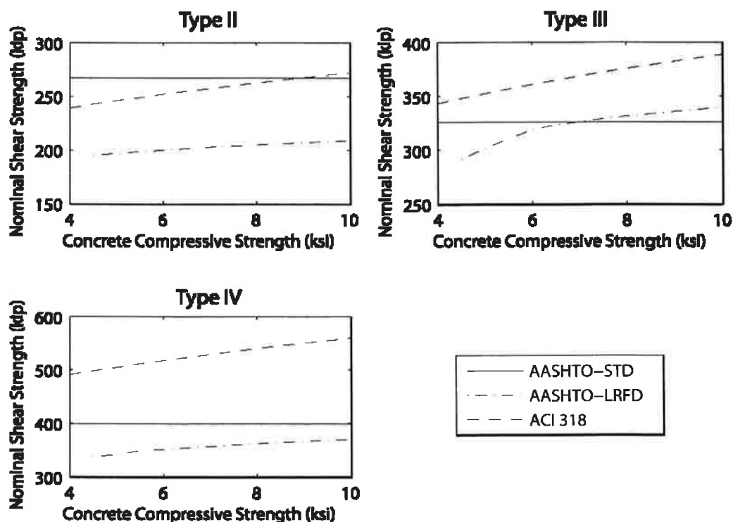
Figure 36: Nominal shear strength as affected by concrete compressive strength for AASHTO Types II, III and IV prestressed concrete girders, respectively.
