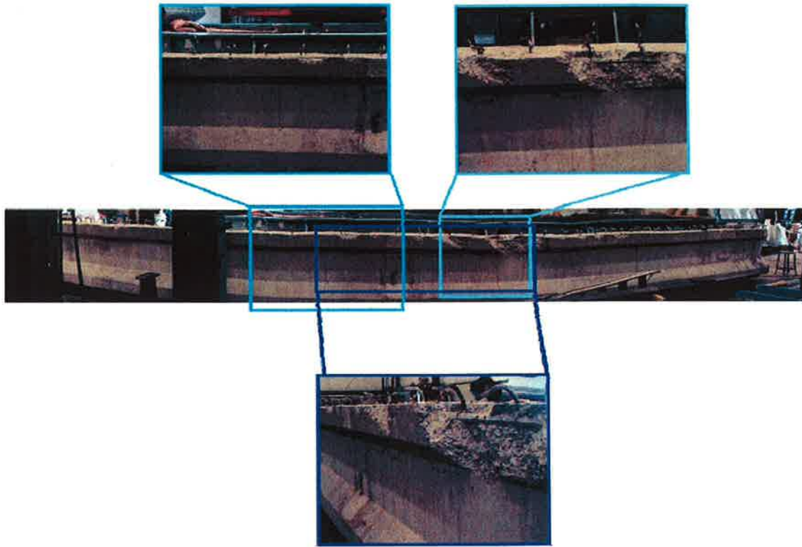
Figure 10: Location and extent of some of damages of the I-244 Bridge girder. These damages include both caused by removing the girder from the bridge and clean-up process.
