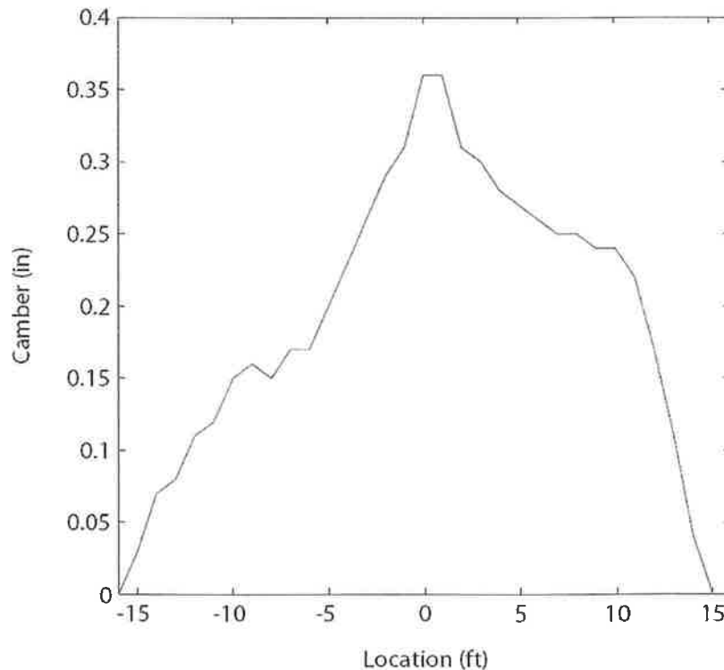
Figure 30: Camber profile of the Wild Horse Creek Bridge girder after Shear Test #1 failure
