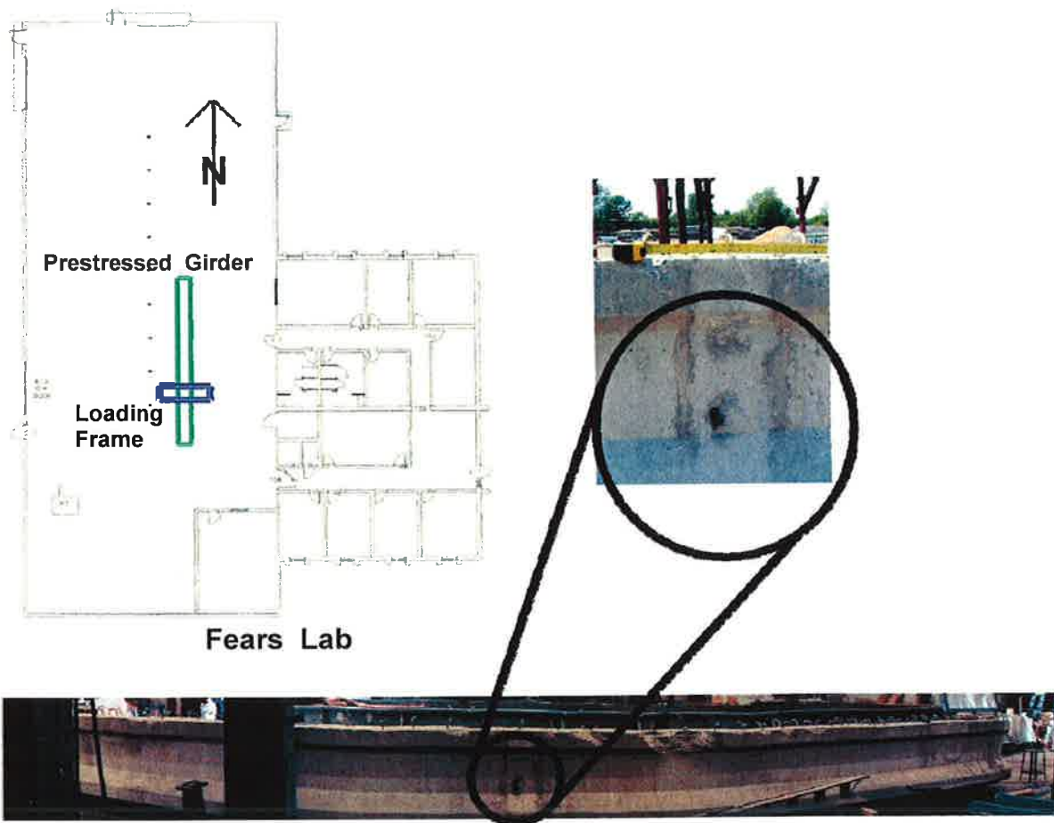
Figure 11: A schematic plan view of Fears Lab shows where the I-244 Bridge girder and loading frame are located as well as two photos to show where the diaphragm hole is located.
