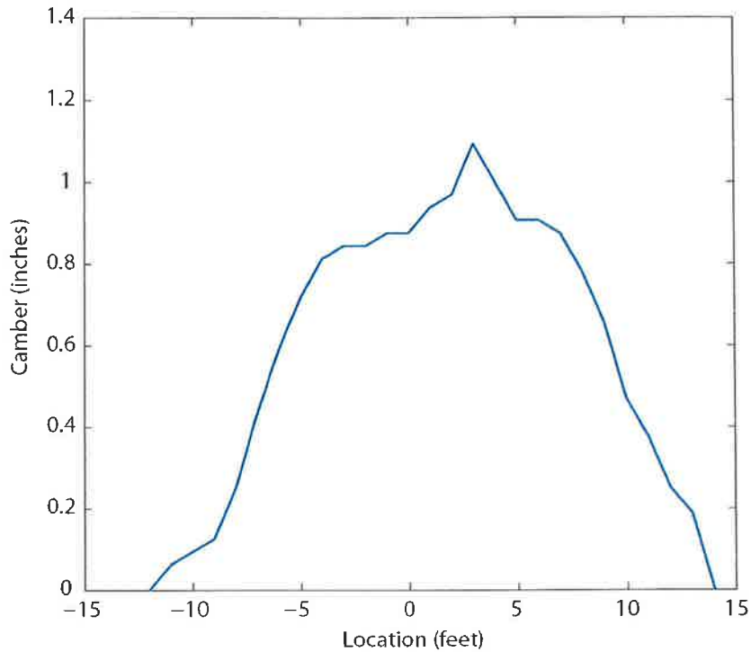
Figure 25: A sample camber profile of the shortened I-244 Bridge girder measured before flexure test configuration #3.
