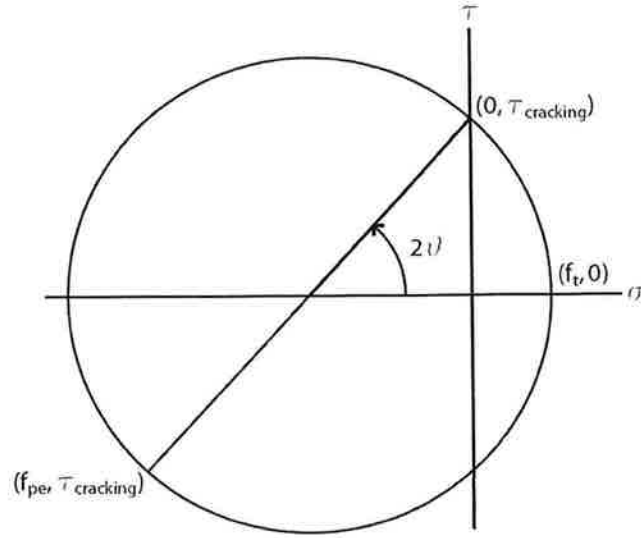
Figure 60: Mohr's Circle of an element at the neutral axis of a prestressed concrete girder when shear cracking begins.
