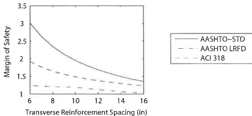
Figure 39: Margin of safety of a Type II girder with varying stirrup spacing
