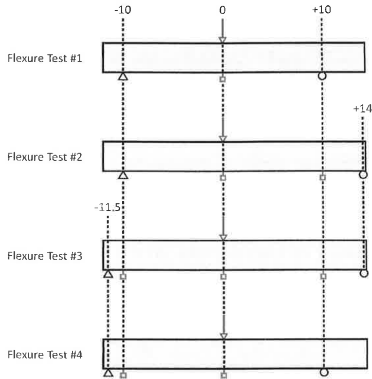
Figure 23: Flexure test configurations for shortened I-244 Bridge girder.
