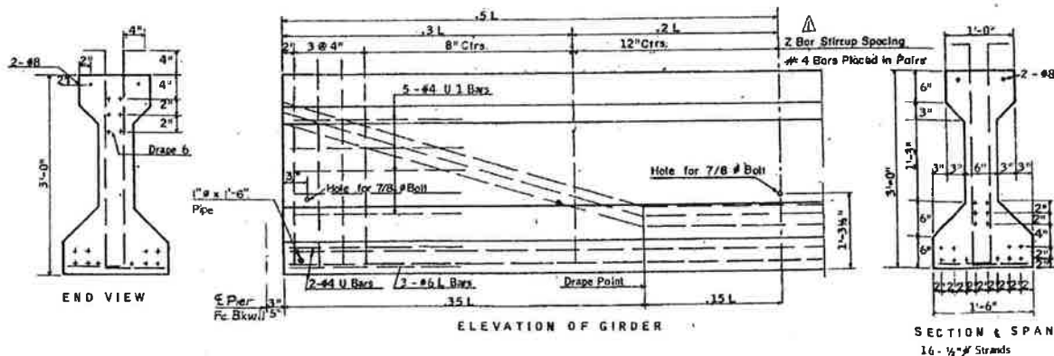
Figure 2: Elevation and details of the selected I-244 Bridge girder (ODOT [2006]).
