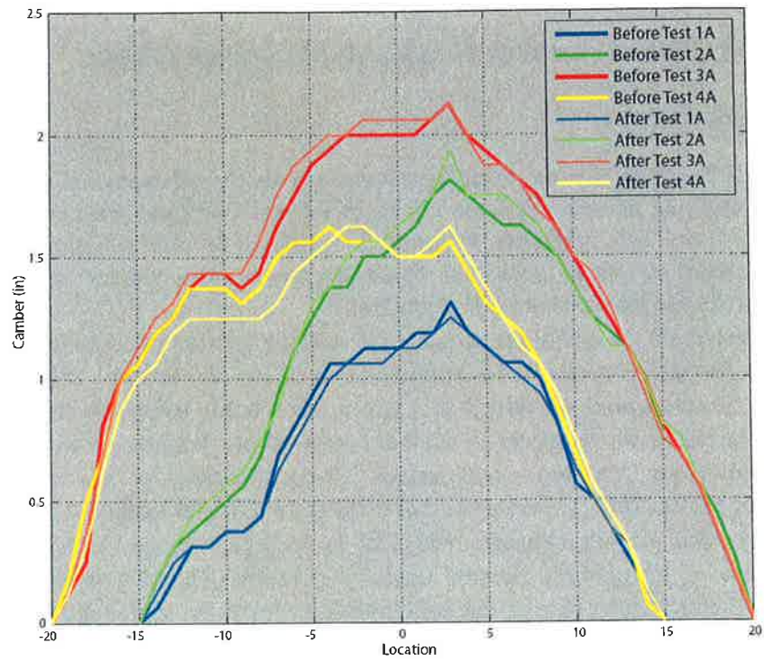
Figure 13: Summary of all measured camber profiles of the original I-244 Bridge girder before and after flexural stiffness tests.
