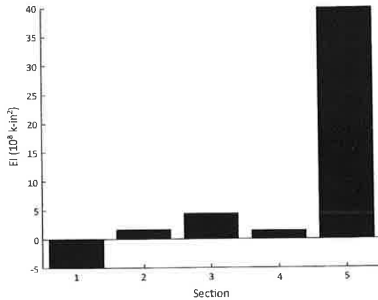
Figure 50: Unconstrained linear least-squares results for piecewise flexural stiffness of the I-244 girder with initial values of zero.
